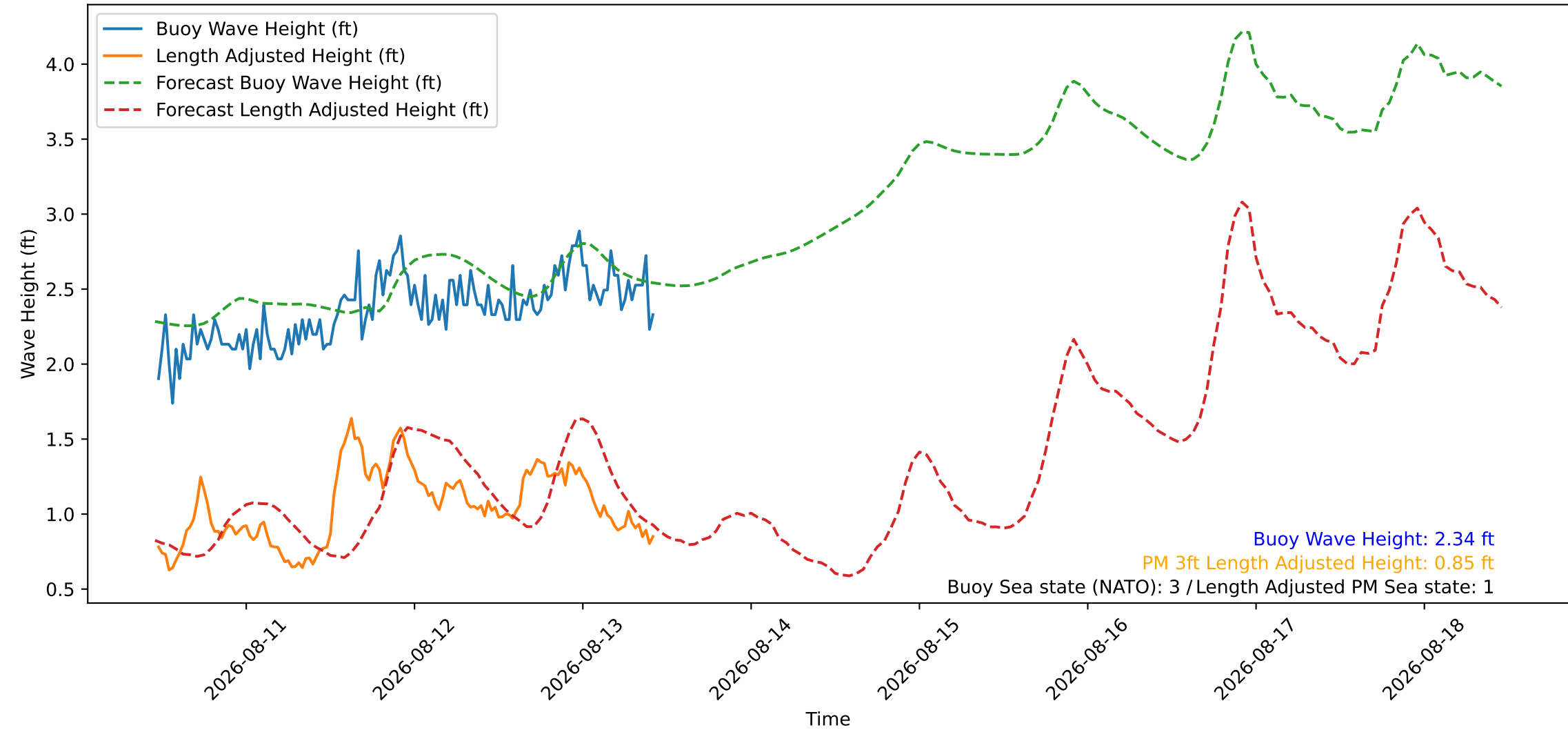
Wave Heights over Time for Red Beach at 2026-08-13 11:00:45
