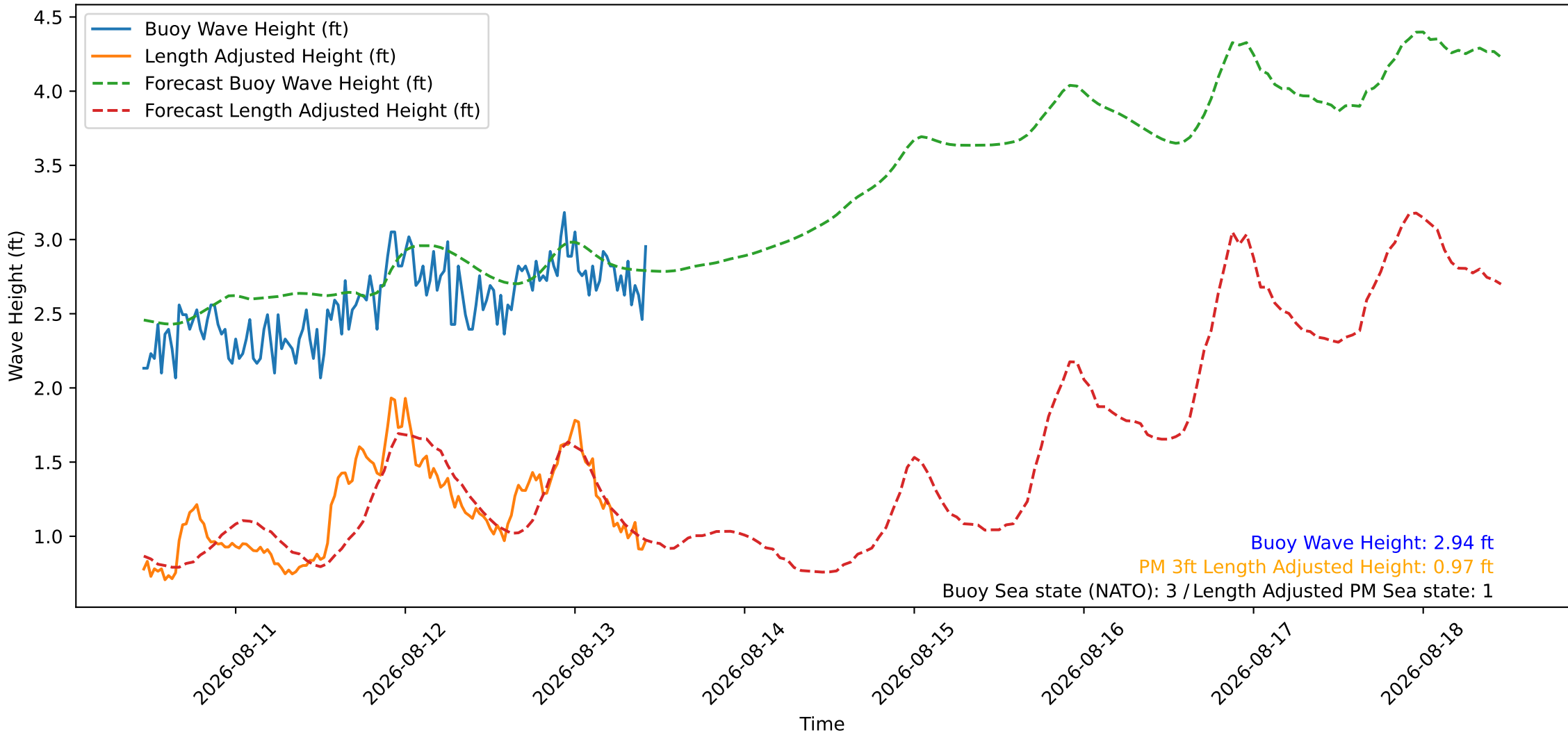
Wave Heights over Time for Oceanside Harbor at 2026-08-13 11:00:26
