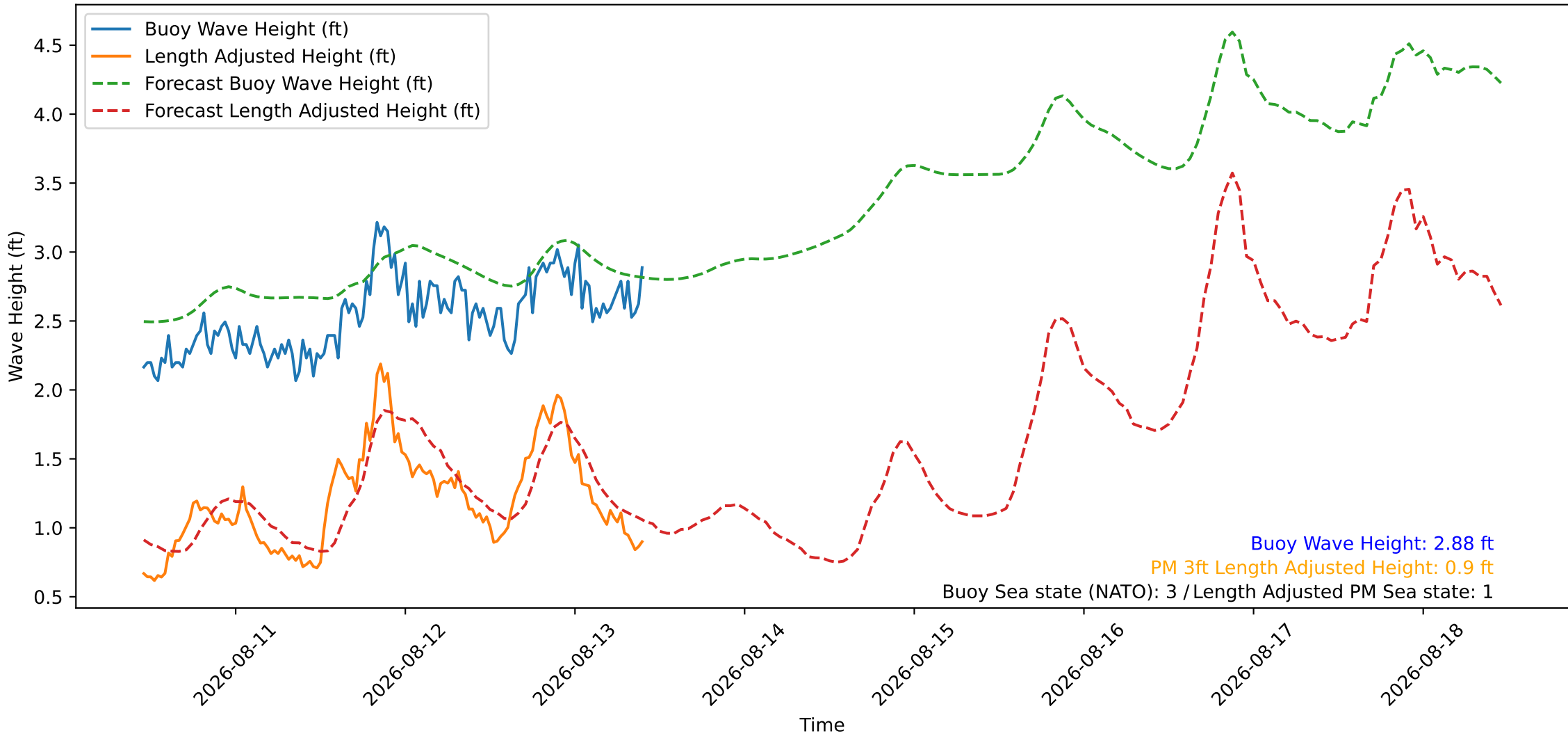
Wave Heights over Time for Green Beach at 2026-08-13 11:01:08
