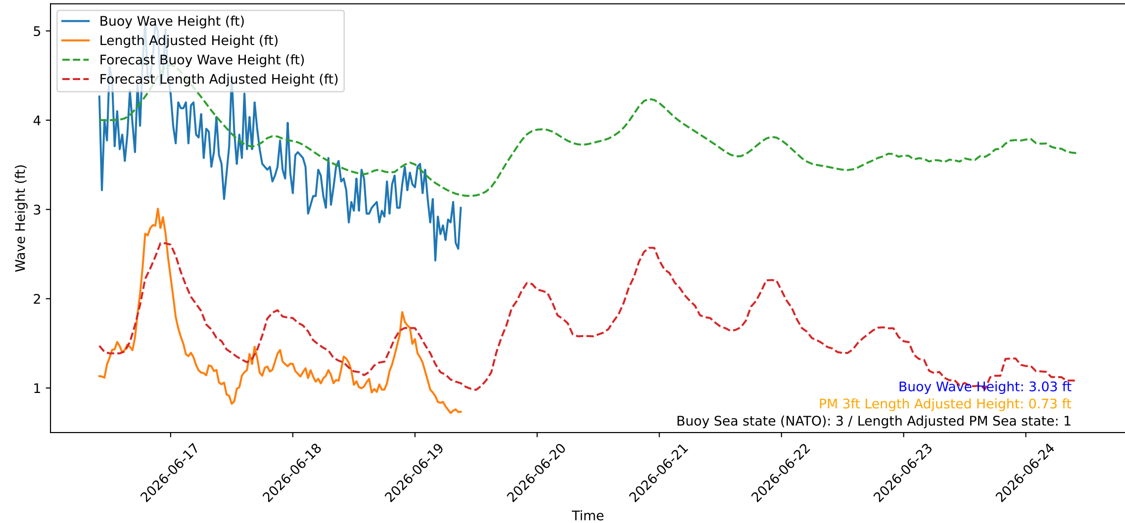
Wave Heights over Time for Green Beach at 2026-06-19 10:01:08
