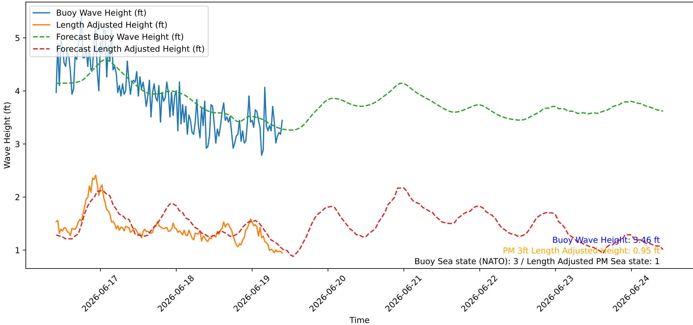
Wave Heights over Time for Oceanside Harbor at 2026-06-19 10:00:26
