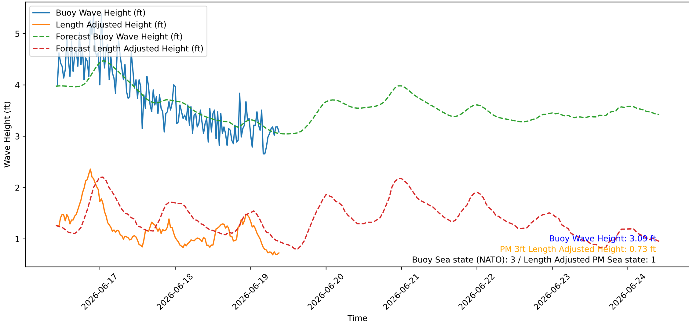
Wave Heights over Time for Red Beach at 2026-06-19 10:00:46
