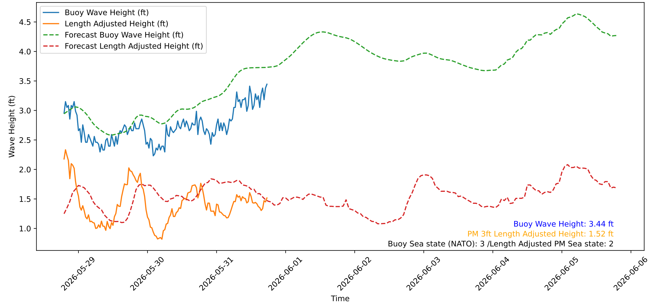
Wave Heights over Time for Red Beach at 2026-05-31 18:30:45
