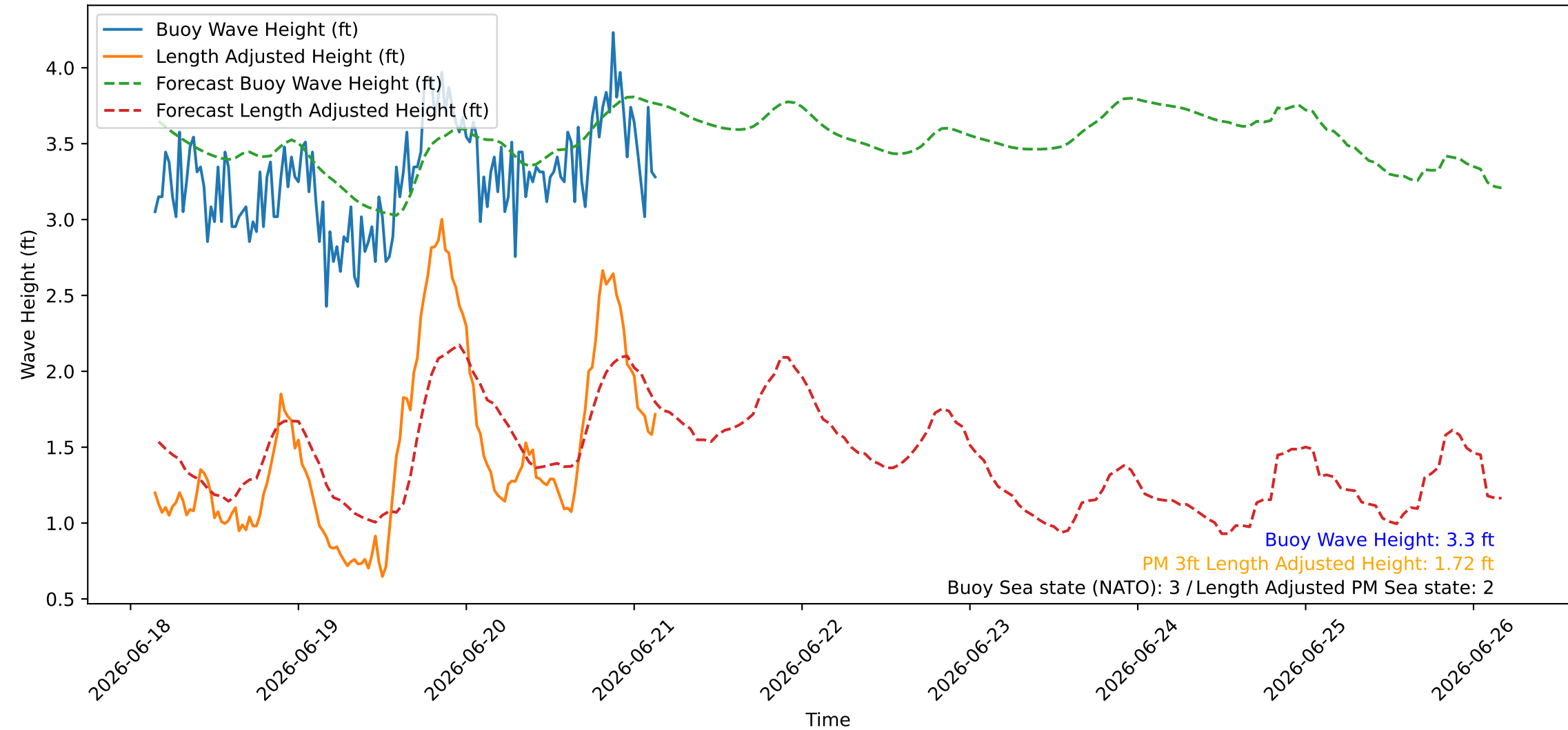
Wave Heights over Time for Green Beach at 2026-06-21 03:41:07
