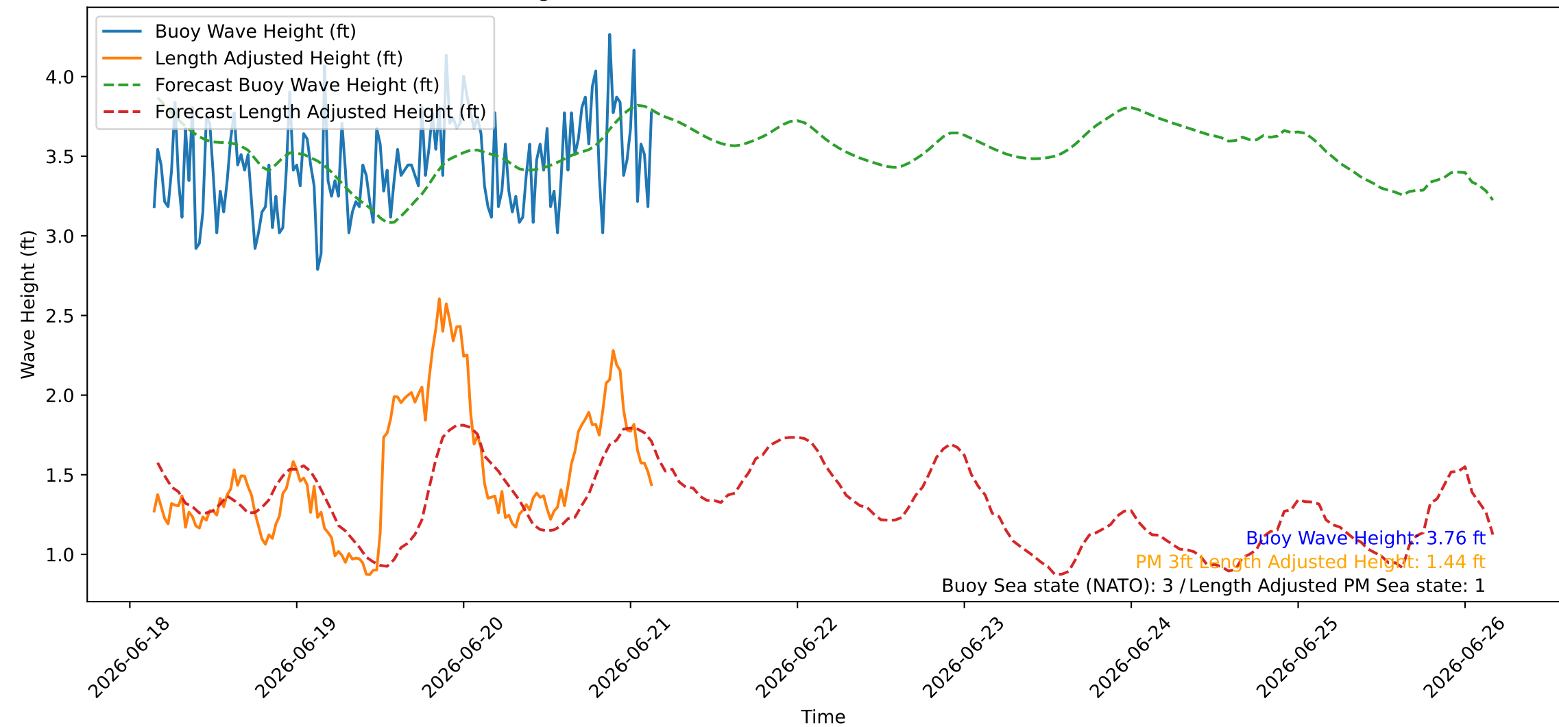
Wave Heights over Time for Oceanside Harbor at 2026-06-21 03:40:26
