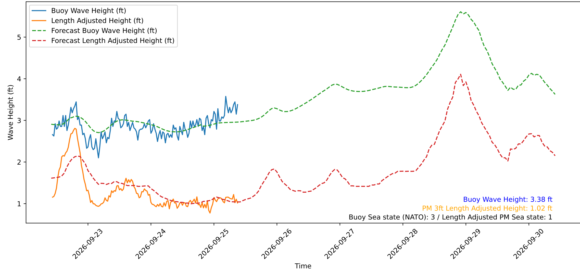
Wave Heights over Time for Green Beach at 2026-09-25 10:01:10
