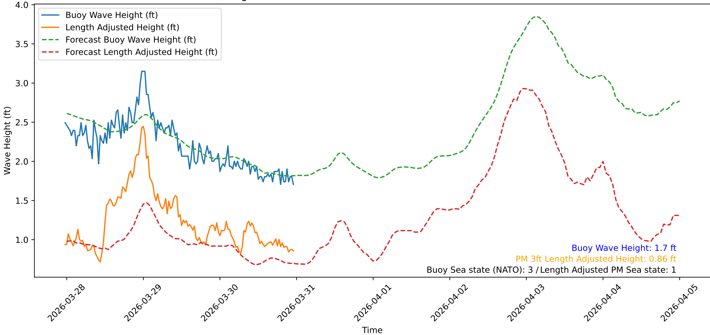
Wave Heights over Time for Oceanside Harbor at 2026-03-30 23:30:31
