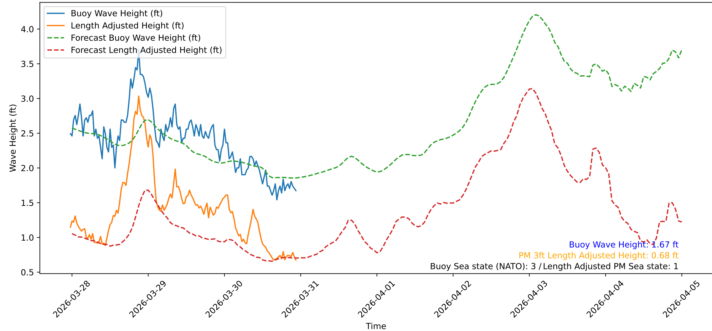
Wave Heights over Time for Green Beach at 2026-03-30 23:31:10
