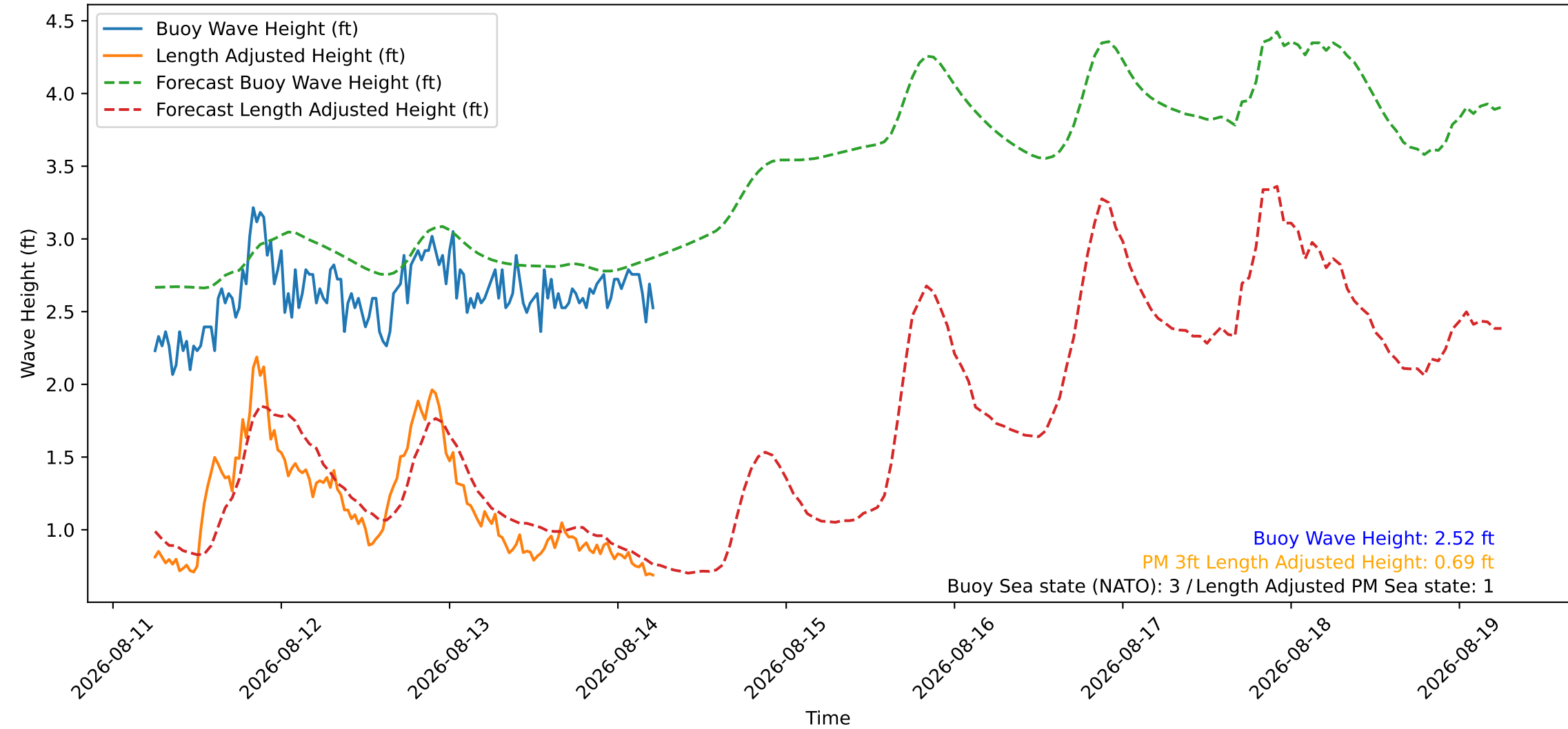
Wave Heights over Time for Green Beach at 2026-08-14 05:51:10
