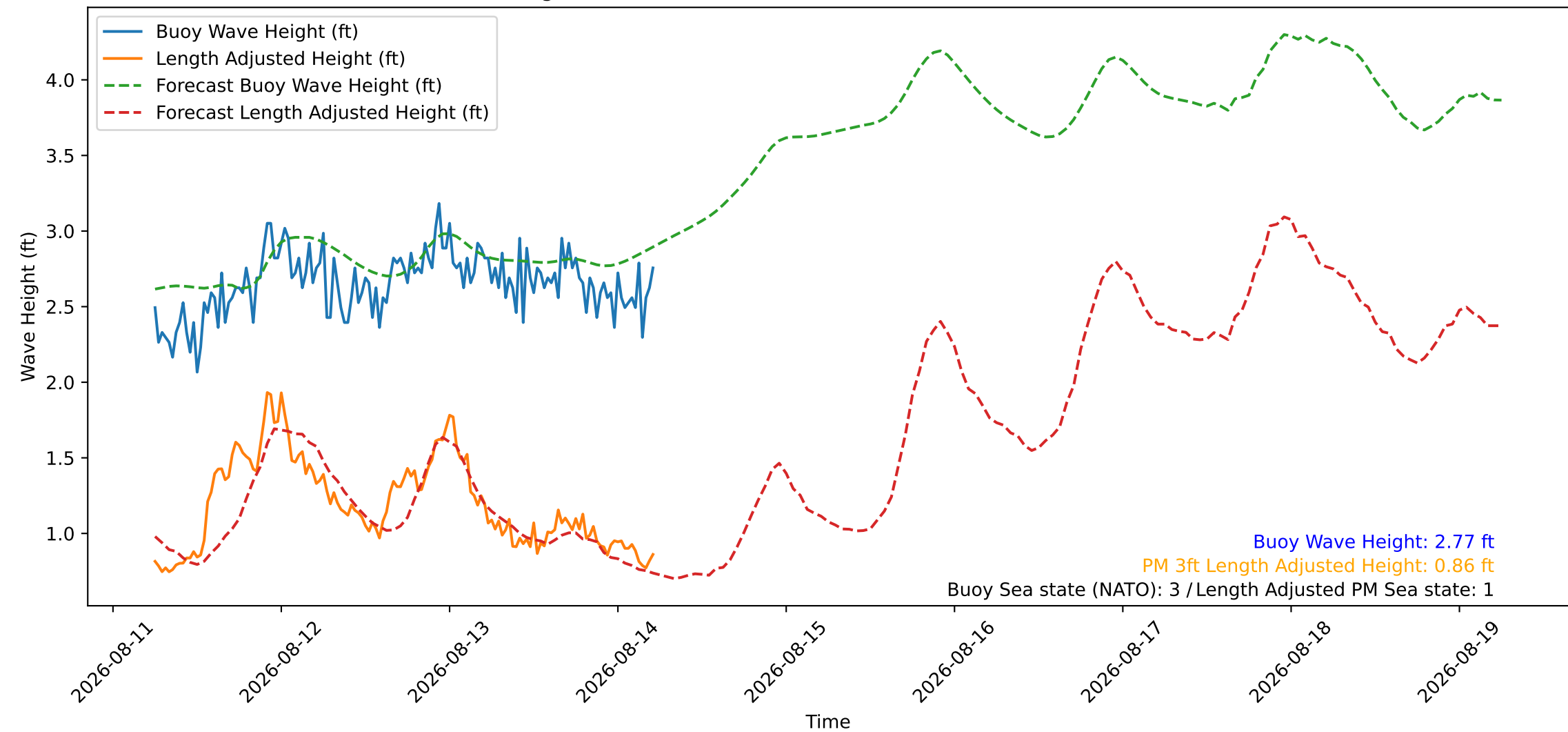
Wave Heights over Time for Oceanside Harbor at 2026-08-14 05:50:26
