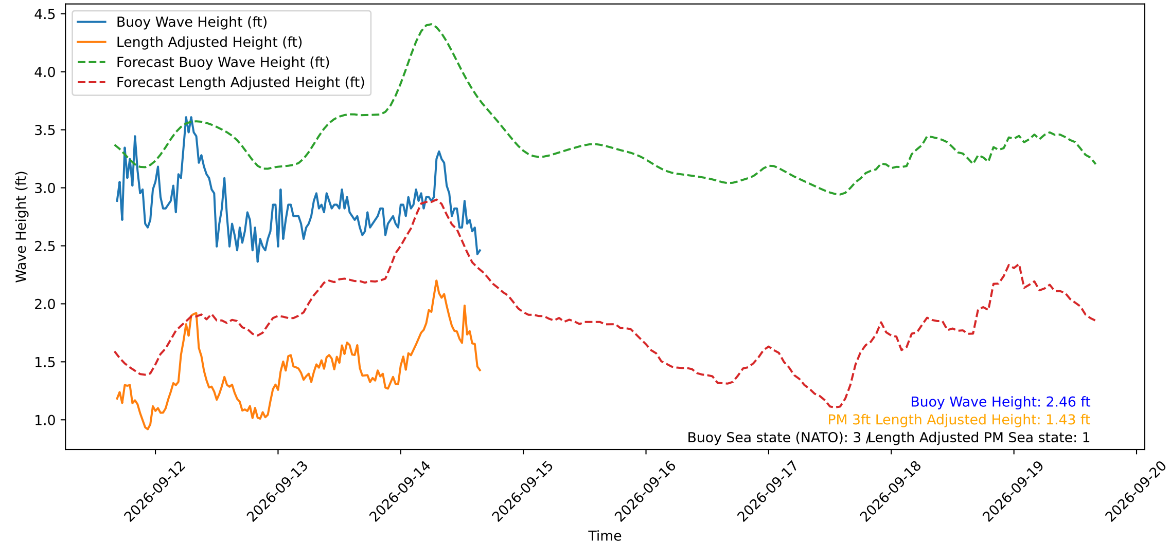
Wave Heights over Time for Green Beach at 2026-09-14 16:11:11
