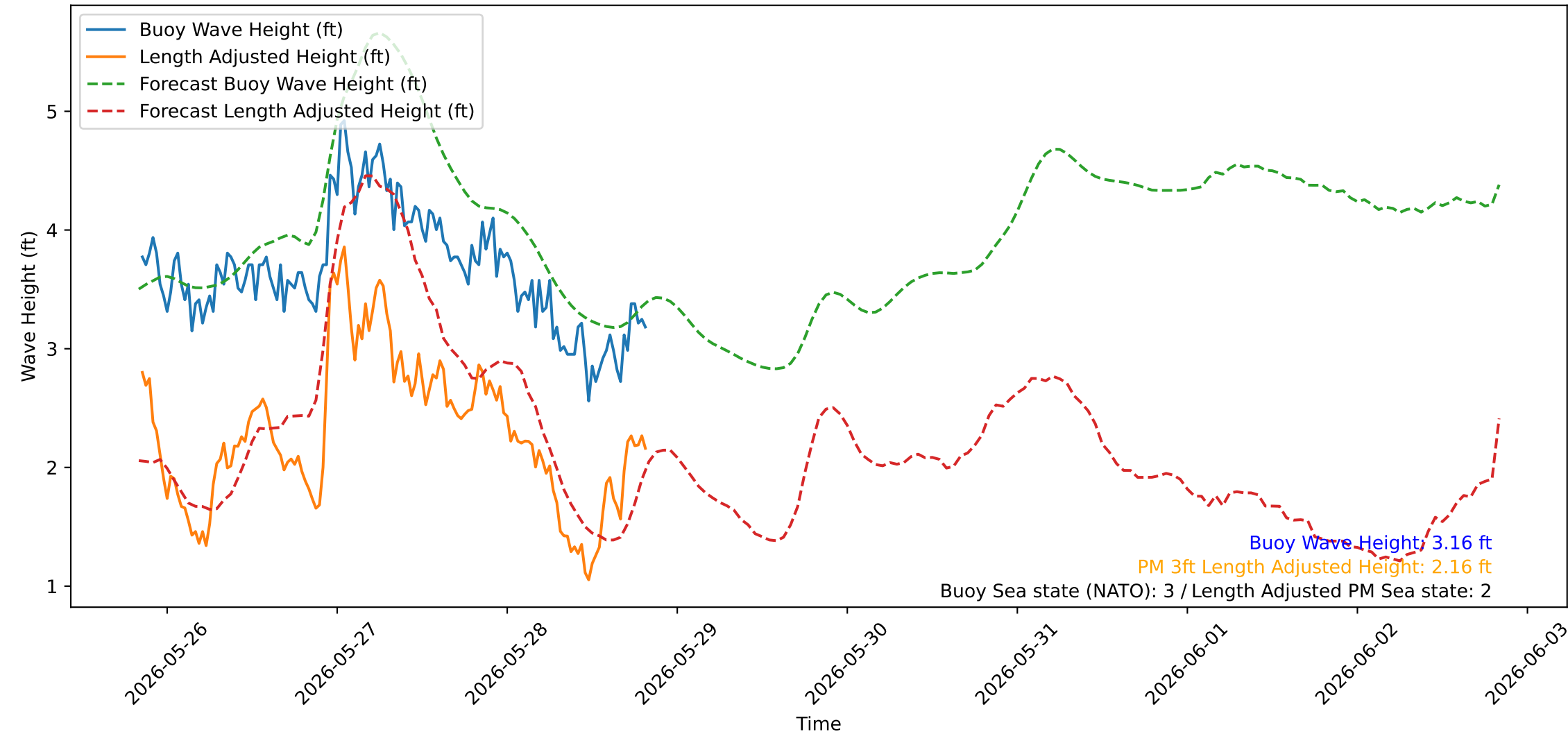
Wave Heights over Time for Green Beach at 2026-05-28 20:21:02
