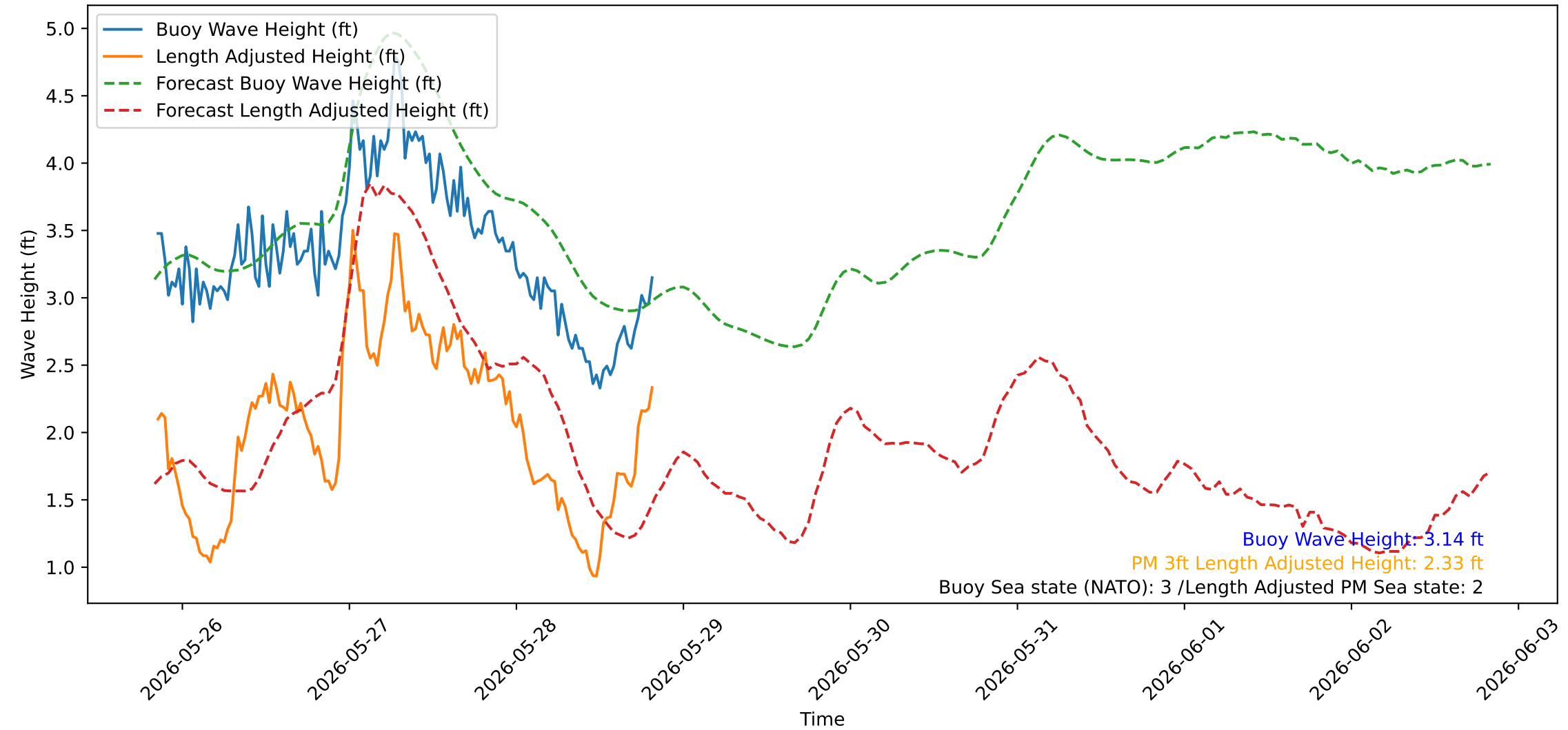
Wave Heights over Time for Red Beach at 2026-05-28 20:20:39
