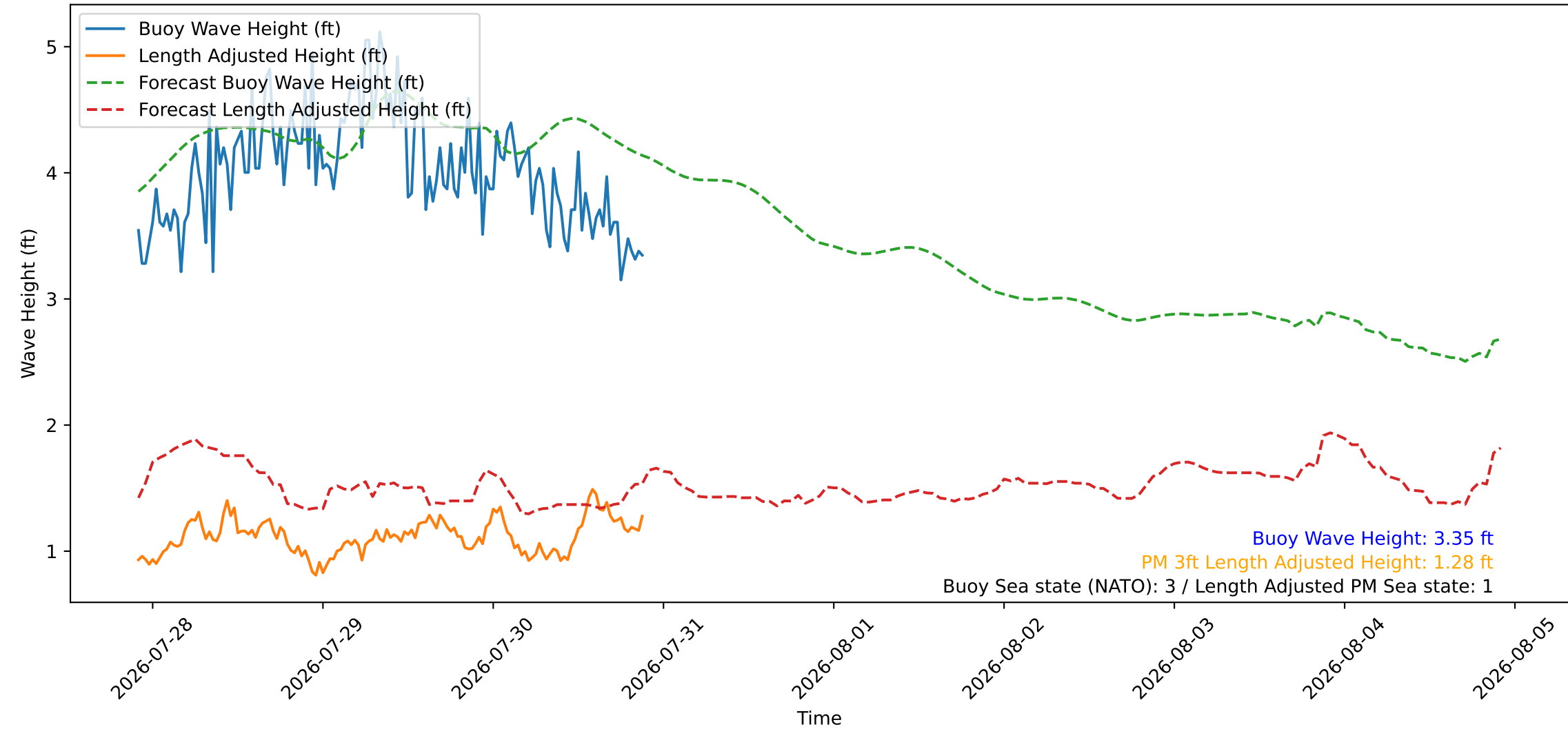
Wave Heights over Time for Red Beach at 2026-07-30 21:40:46
