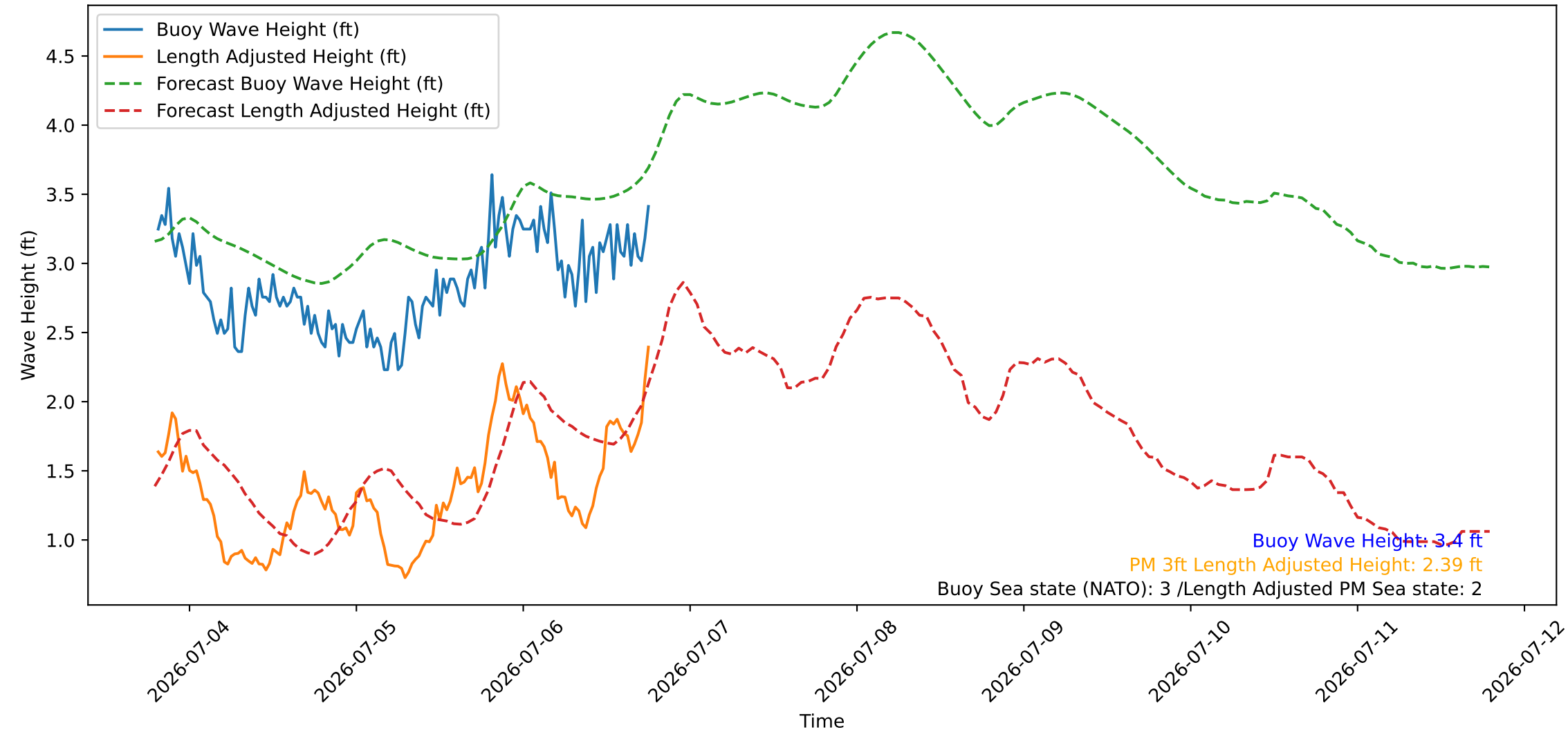
Wave Heights over Time for Red Beach at 2026-07-06 19:10:46
