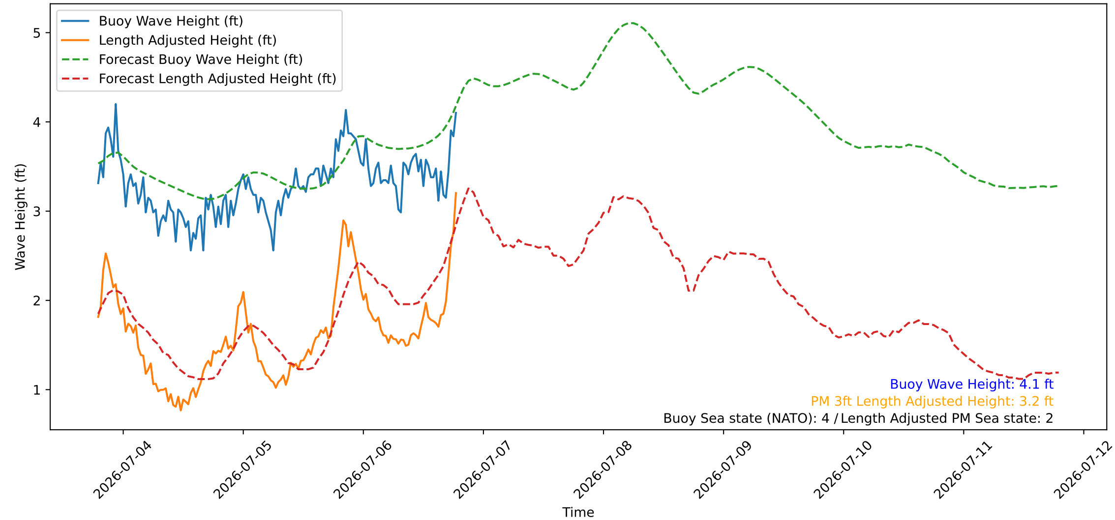
Wave Heights over Time for Green Beach at 2026-07-06 19:11:08
