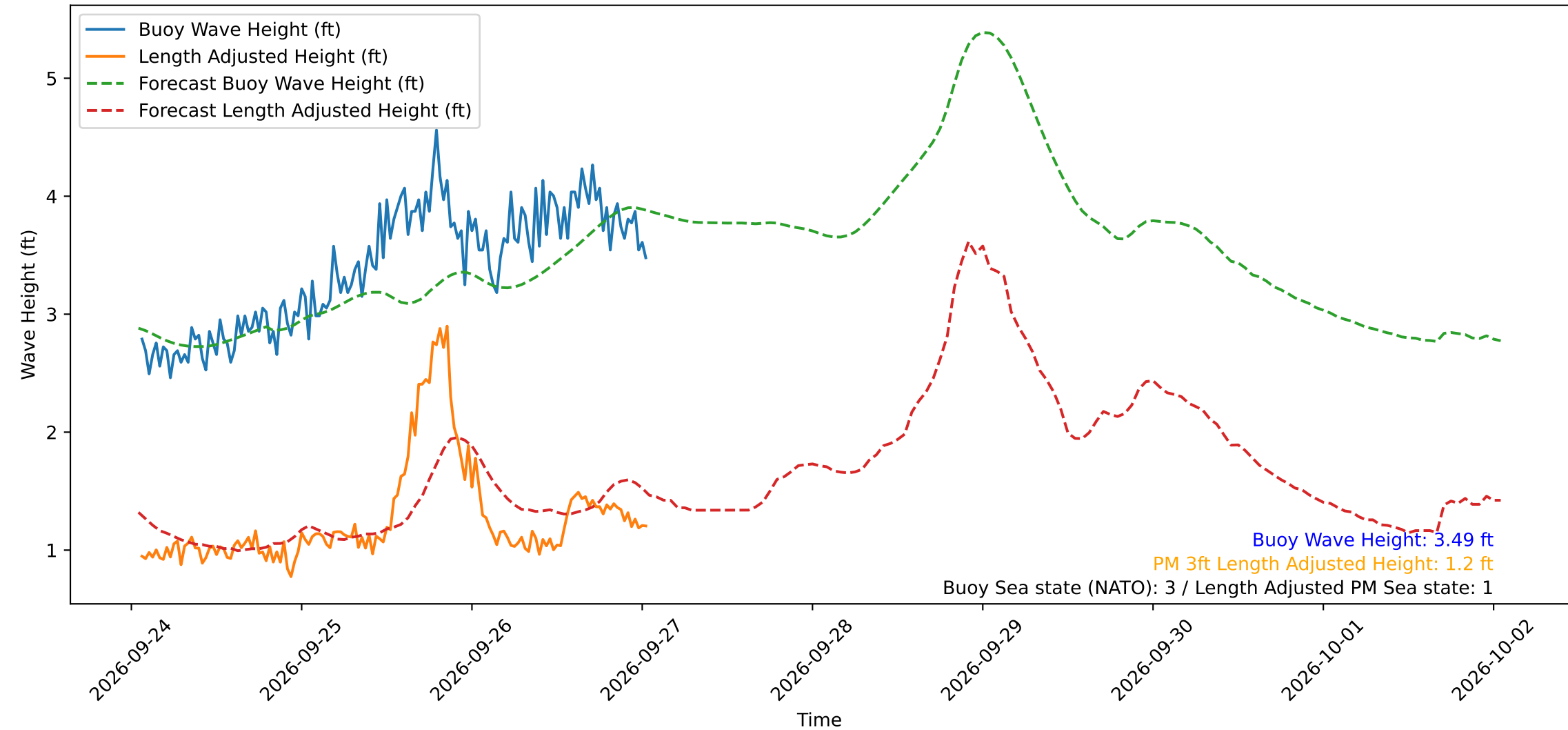
Wave Heights over Time for Green Beach at 2026-09-27 01:11:12
