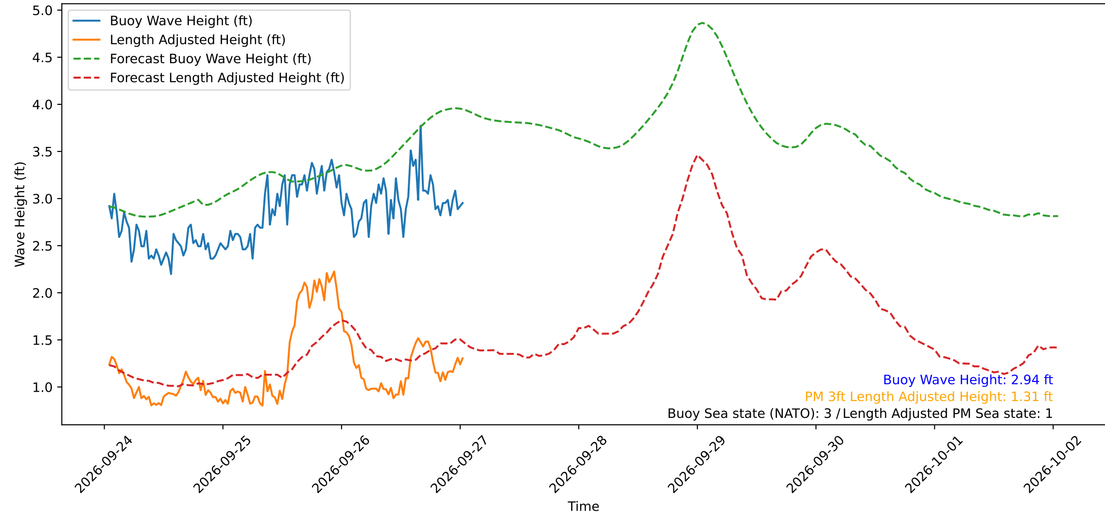
Wave Heights over Time for Oceanside Harbor at 2026-09-27 01:10:30
