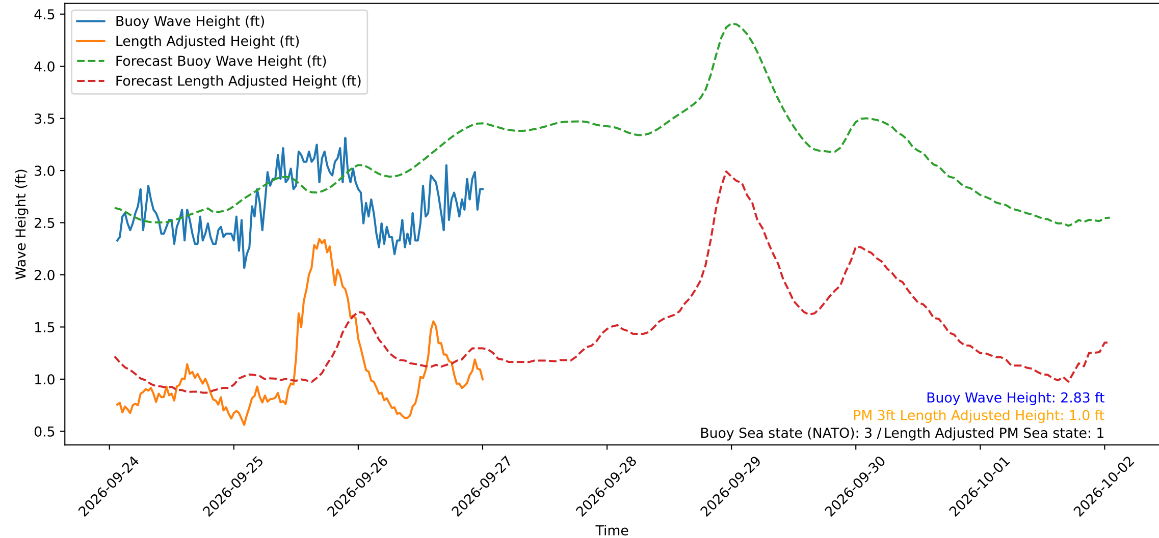
Wave Heights over Time for Red Beach at 2026-09-27 01:10:49
