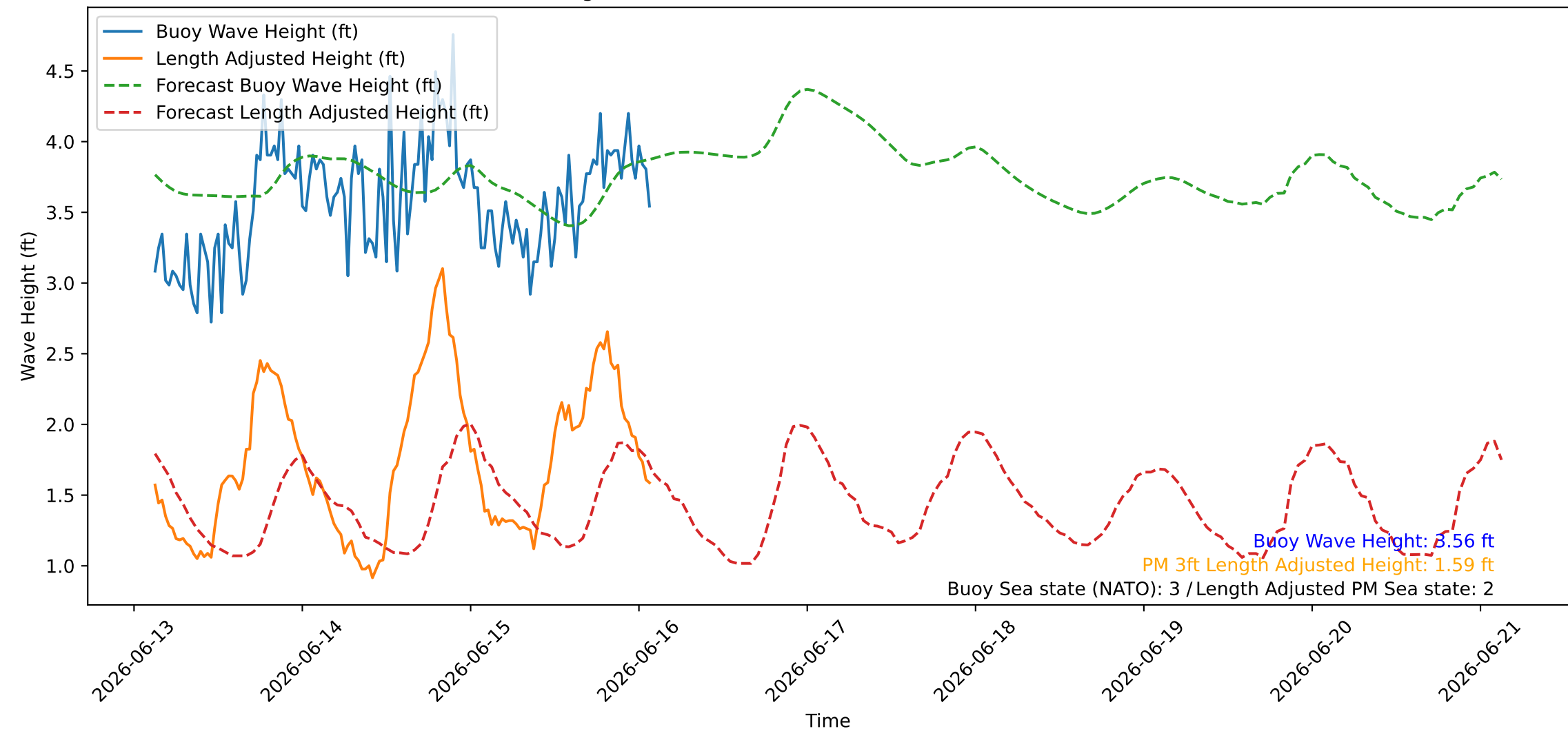
Wave Heights over Time for Red Beach at 2026-06-16 02:30:46
