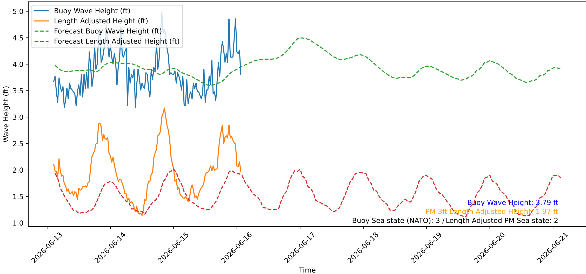
Wave Heights over Time for Oceanside Harbor at 2026-06-16 02:30:27
