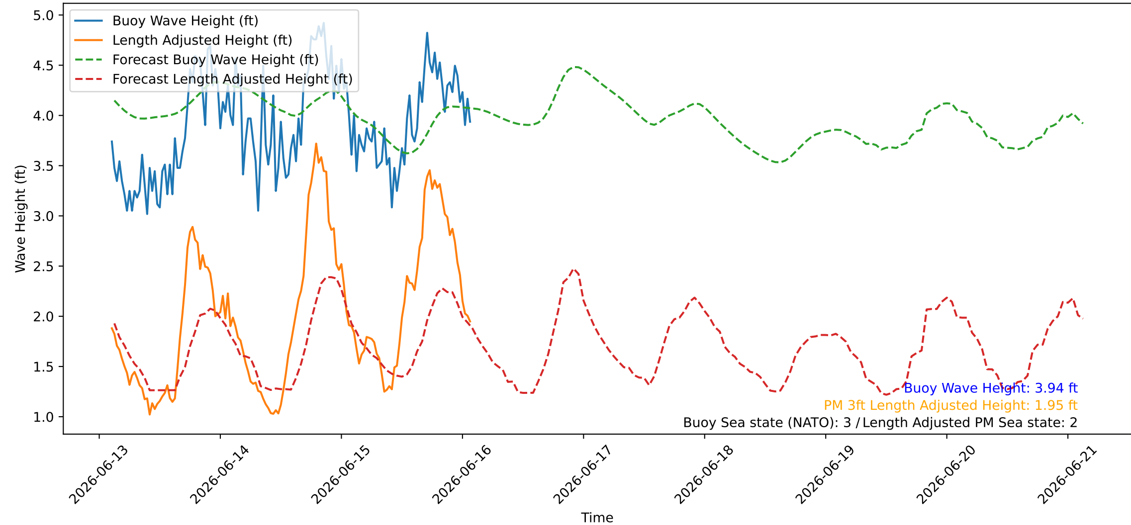
Wave Heights over Time for Green Beach at 2026-06-16 02:31:08
