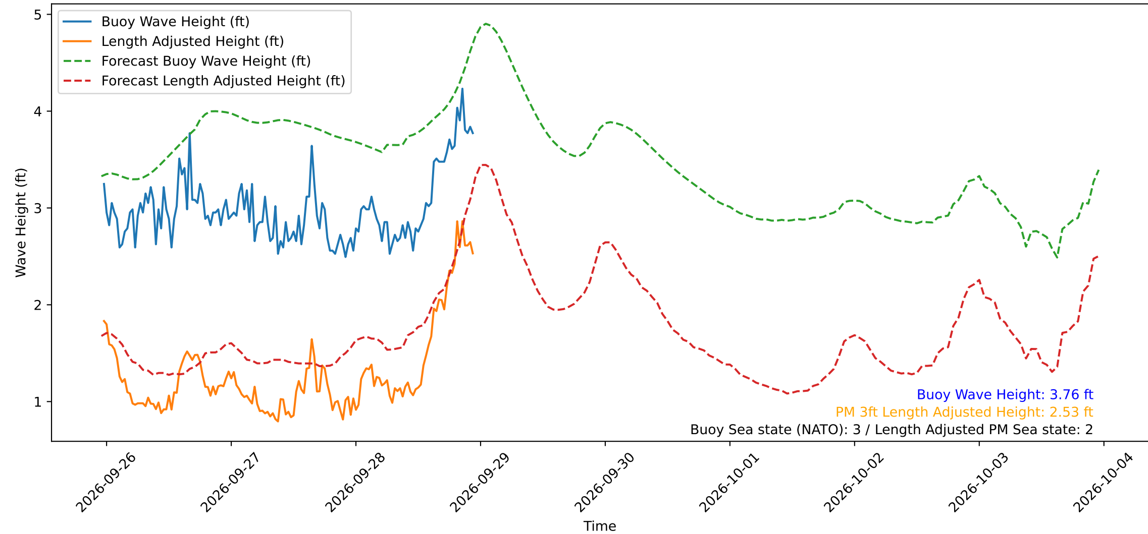
Wave Heights over Time for Oceanside Harbor at 2026-09-28 23:20:30
