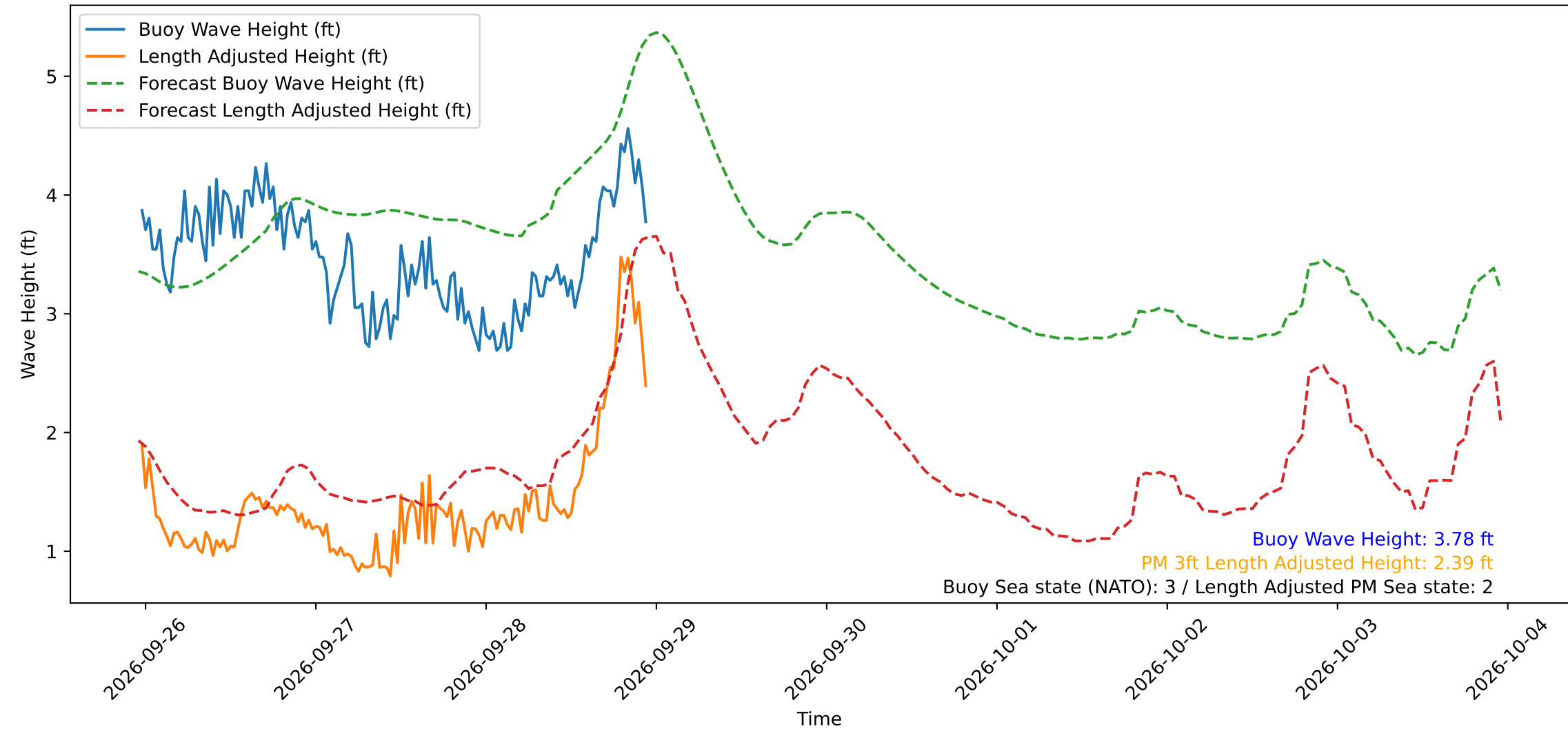
Wave Heights over Time for Green Beach at 2026-09-28 23:21:16
