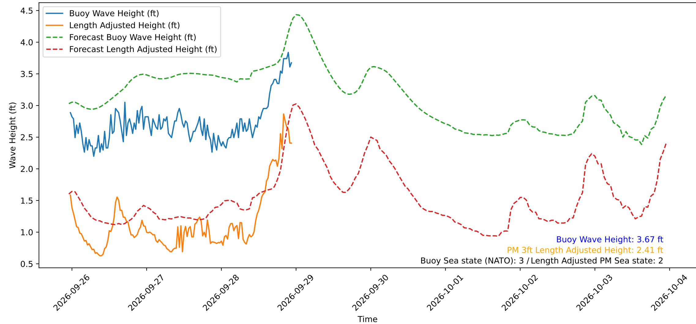
Wave Heights over Time for Red Beach at 2026-09-28 23:20:52
