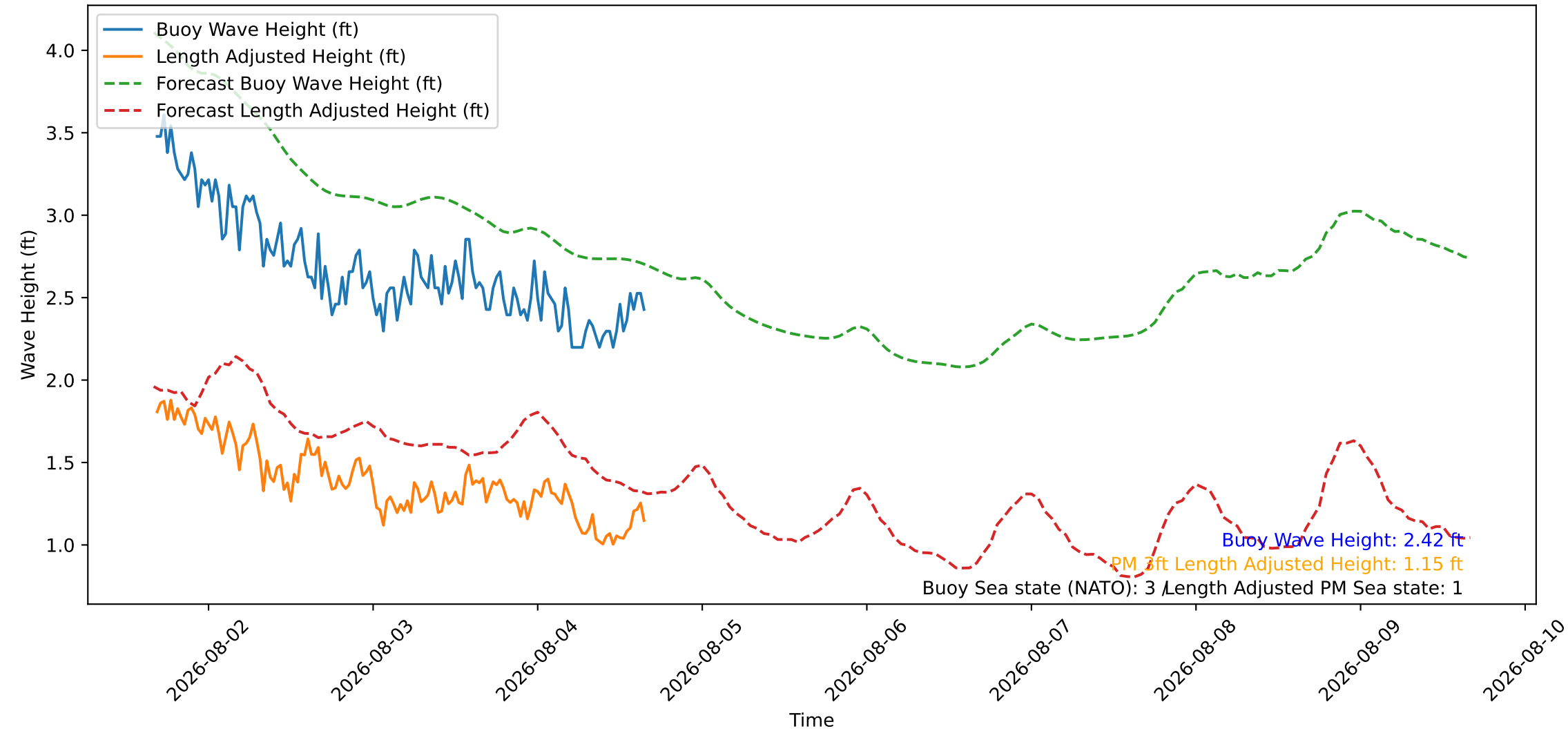
Wave Heights over Time for Oceanside Harbor at 2026-08-04 16:20:26
