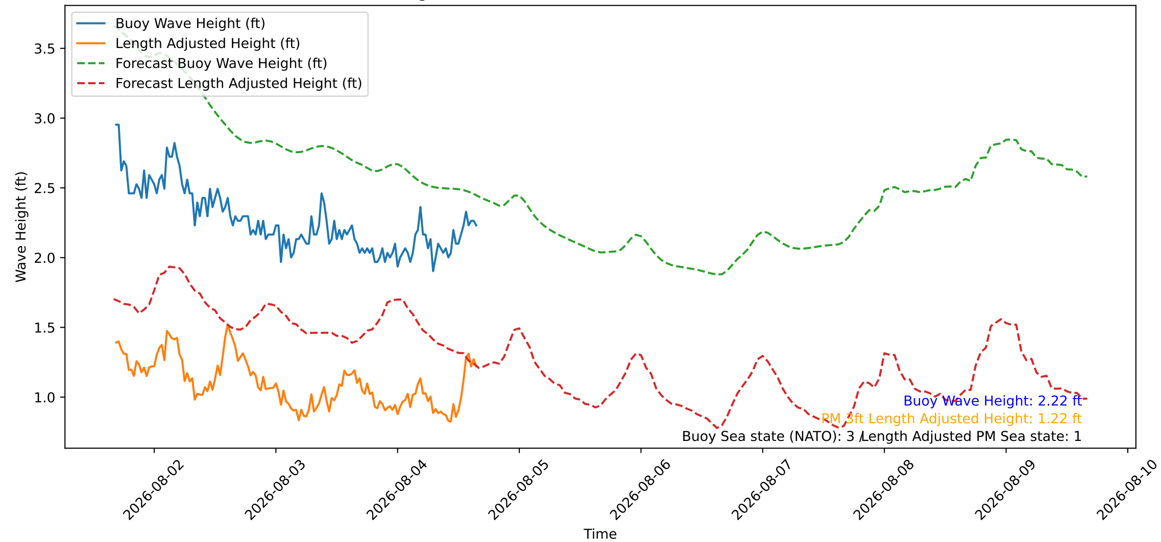
Wave Heights over Time for Red Beach at 2026-08-04 16:20:47
