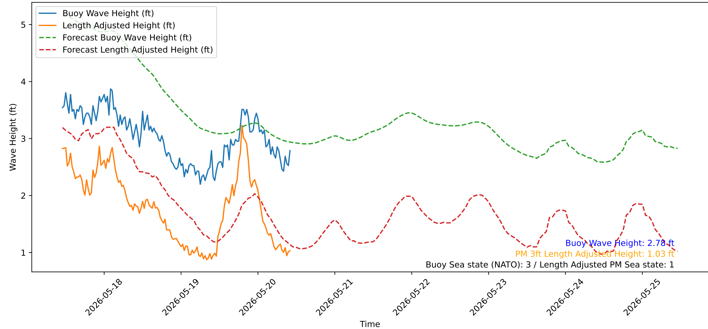
Wave Heights over Time for Oceanside Harbor at 2026-05-20 10:50:31
