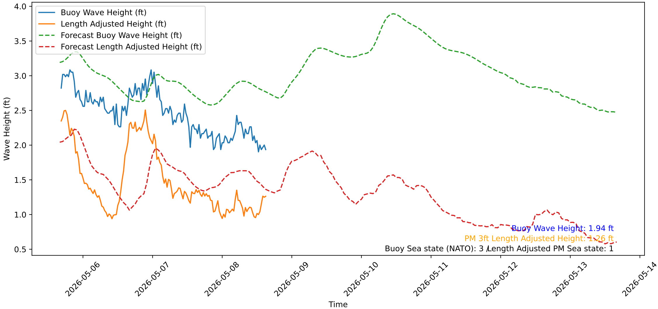
Wave Heights over Time for Red Beach at 2026-05-08 16:10:50
