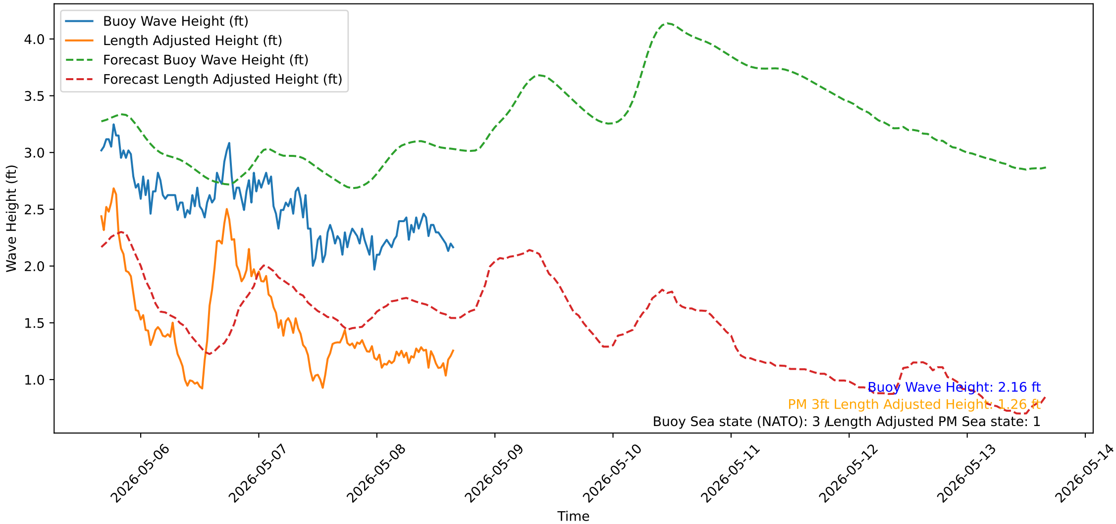
Wave Heights over Time for Oceanside Harbor at 2026-05-08 16:10:31
