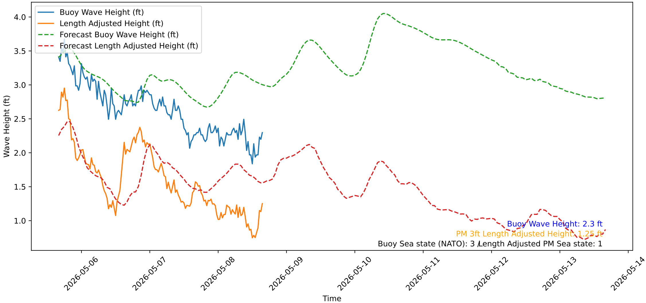
Wave Heights over Time for Green Beach at 2026-05-08 16:11:12
