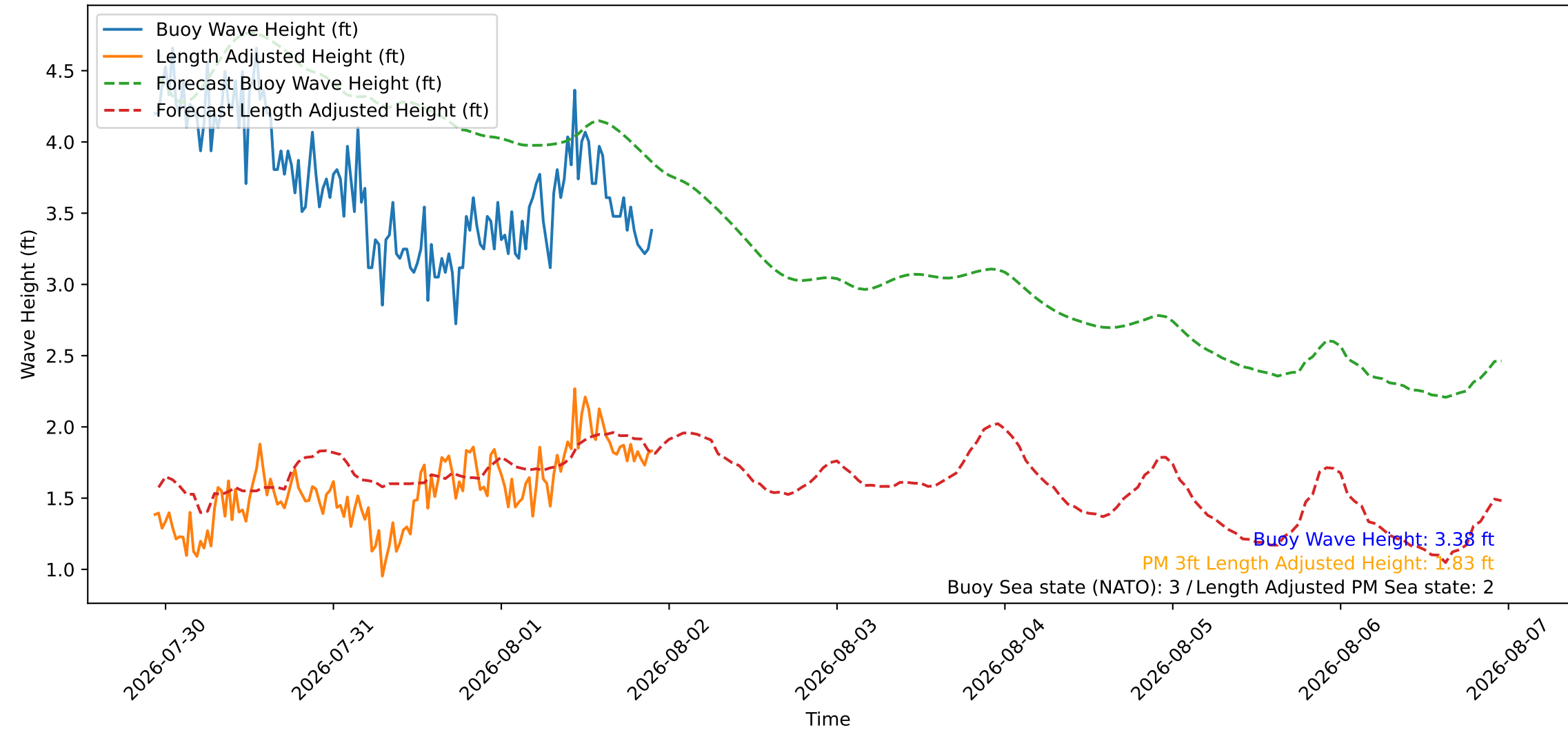
Wave Heights over Time for Oceanside Harbor at 2026-08-01 22:30:26
