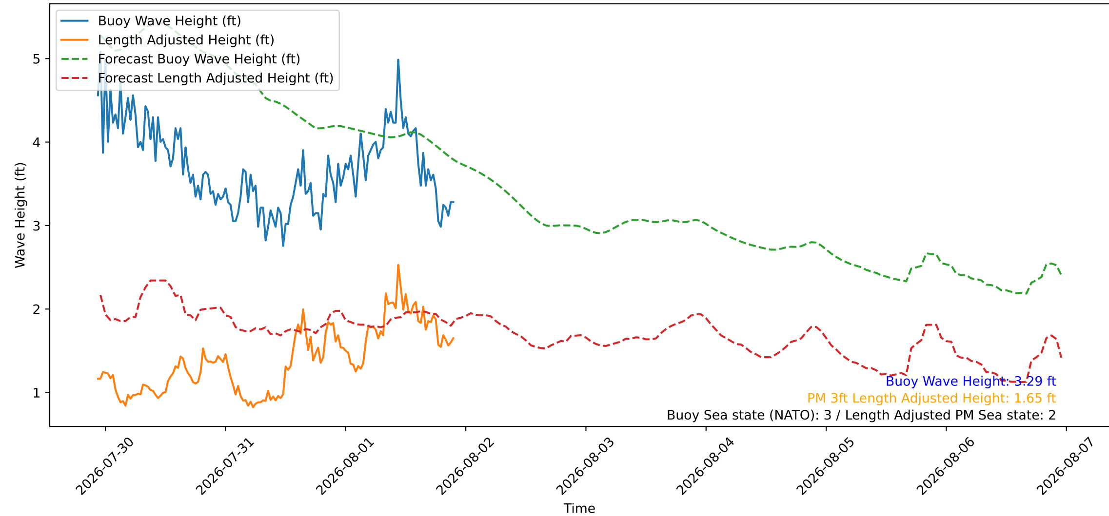
Wave Heights over Time for Green Beach at 2026-08-01 22:31:08
