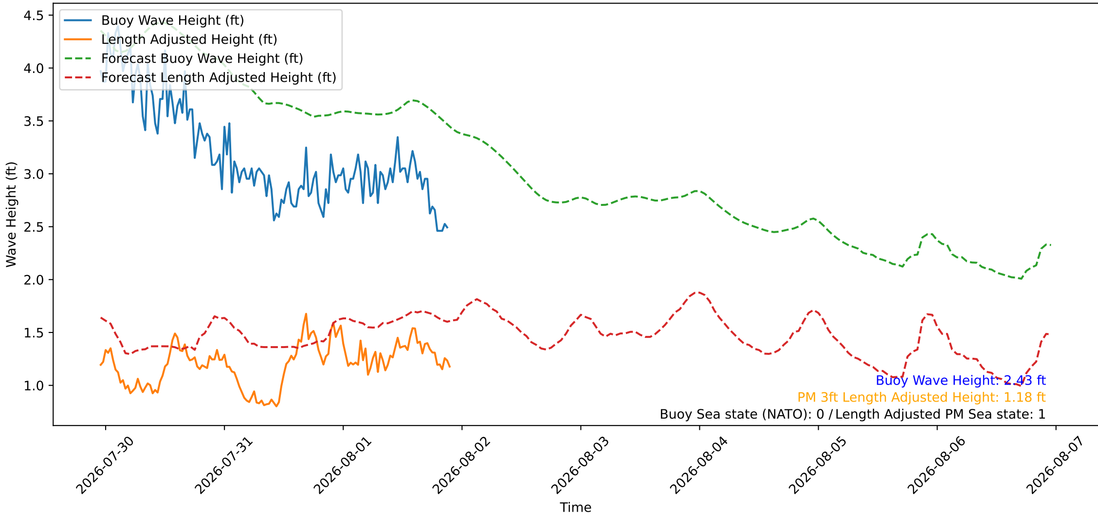
Wave Heights over Time for Red Beach at 2026-08-01 22:30:46
