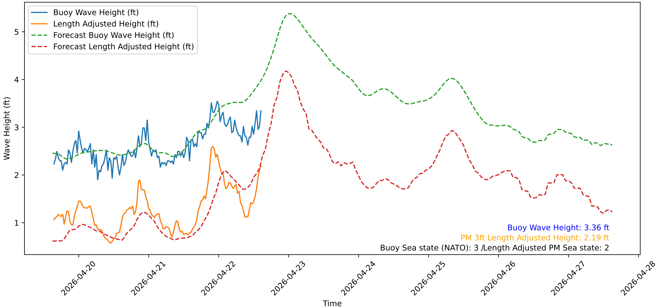
Wave Heights over Time for Green Beach at 2026-04-22 15:21:13
