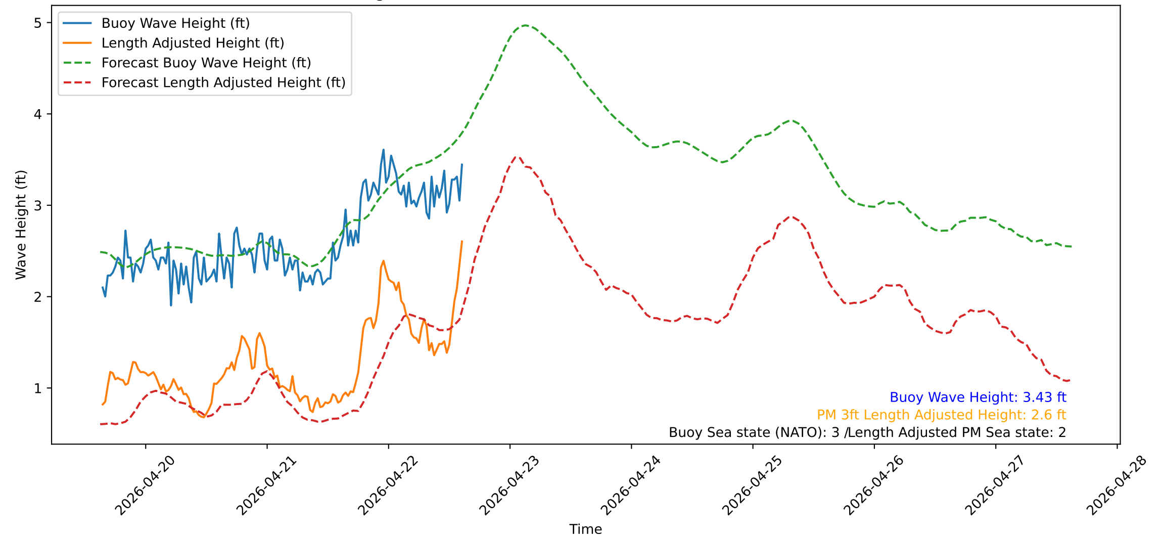
Wave Heights over Time for Oceanside Harbor at 2026-04-22 15:20:31
