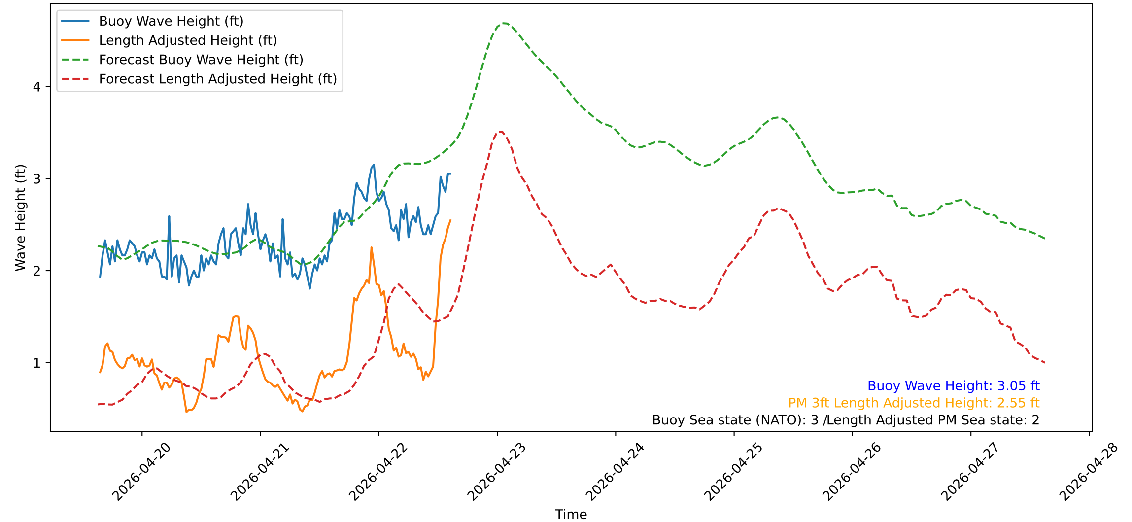
Wave Heights over Time for Red Beach at 2026-04-22 15:20:51
