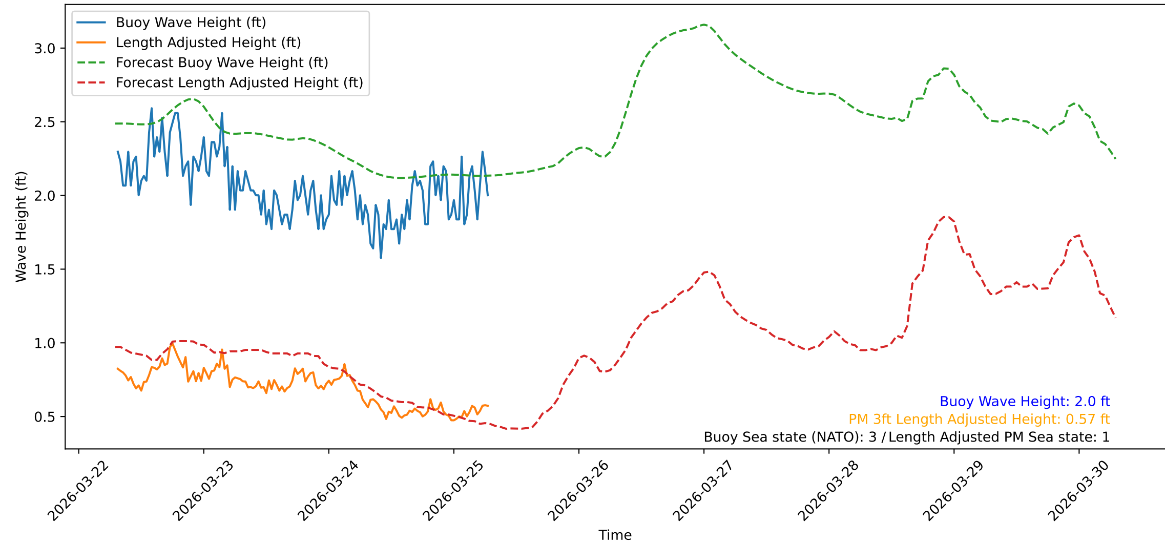
Wave Heights over Time for Oceanside Harbor at 2026-03-25 07:20:31
