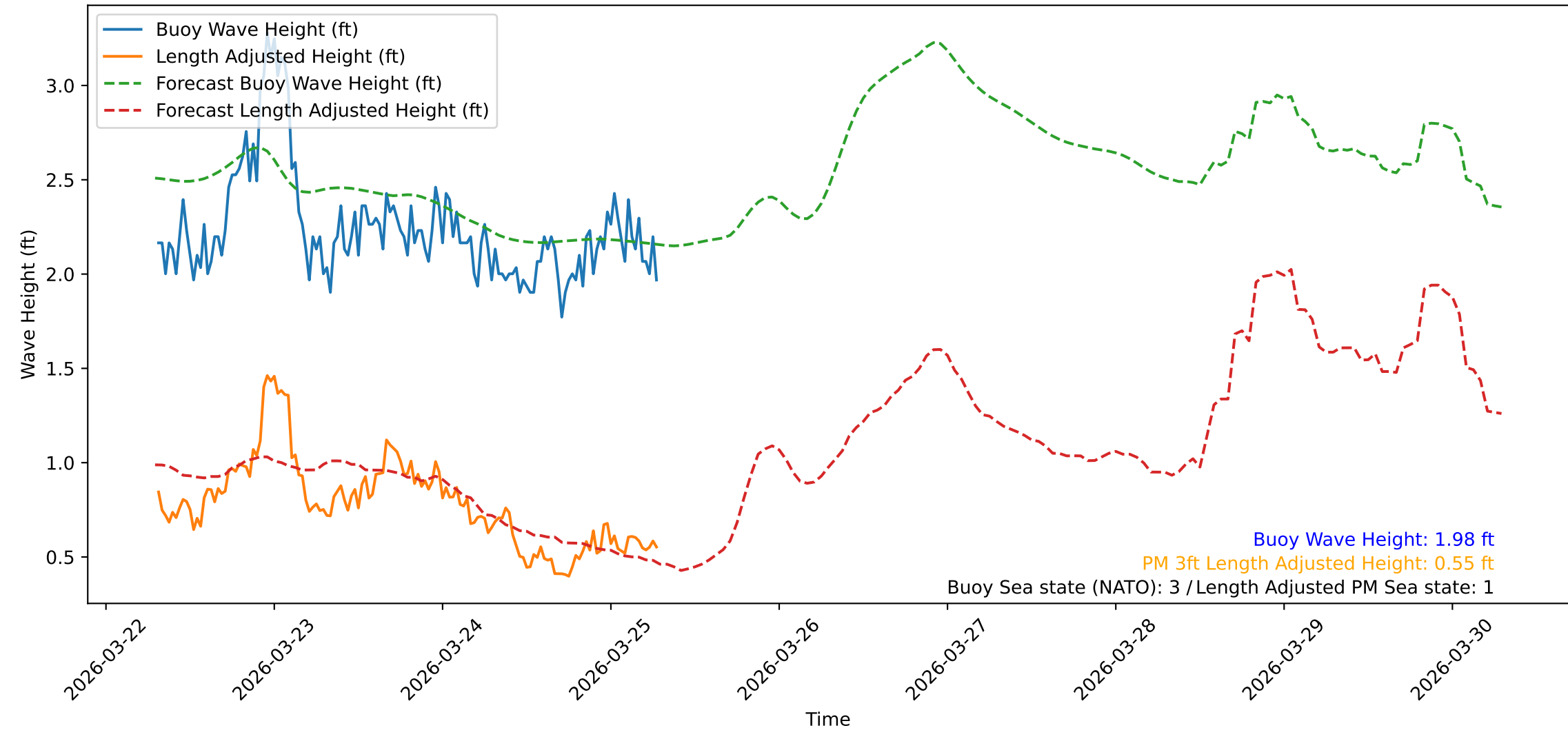
Wave Heights over Time for Green Beach at 2026-03-25 07:21:09
