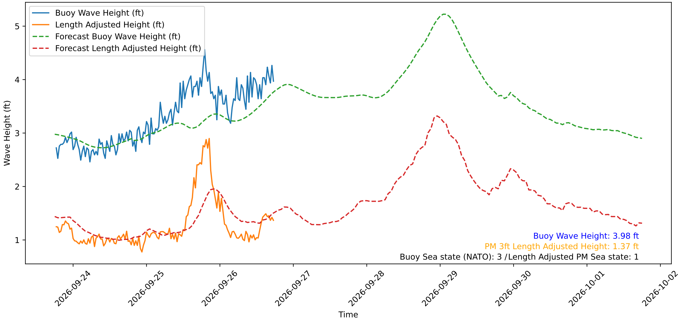
Wave Heights over Time for Green Beach at 2026-09-26 18:21:13
