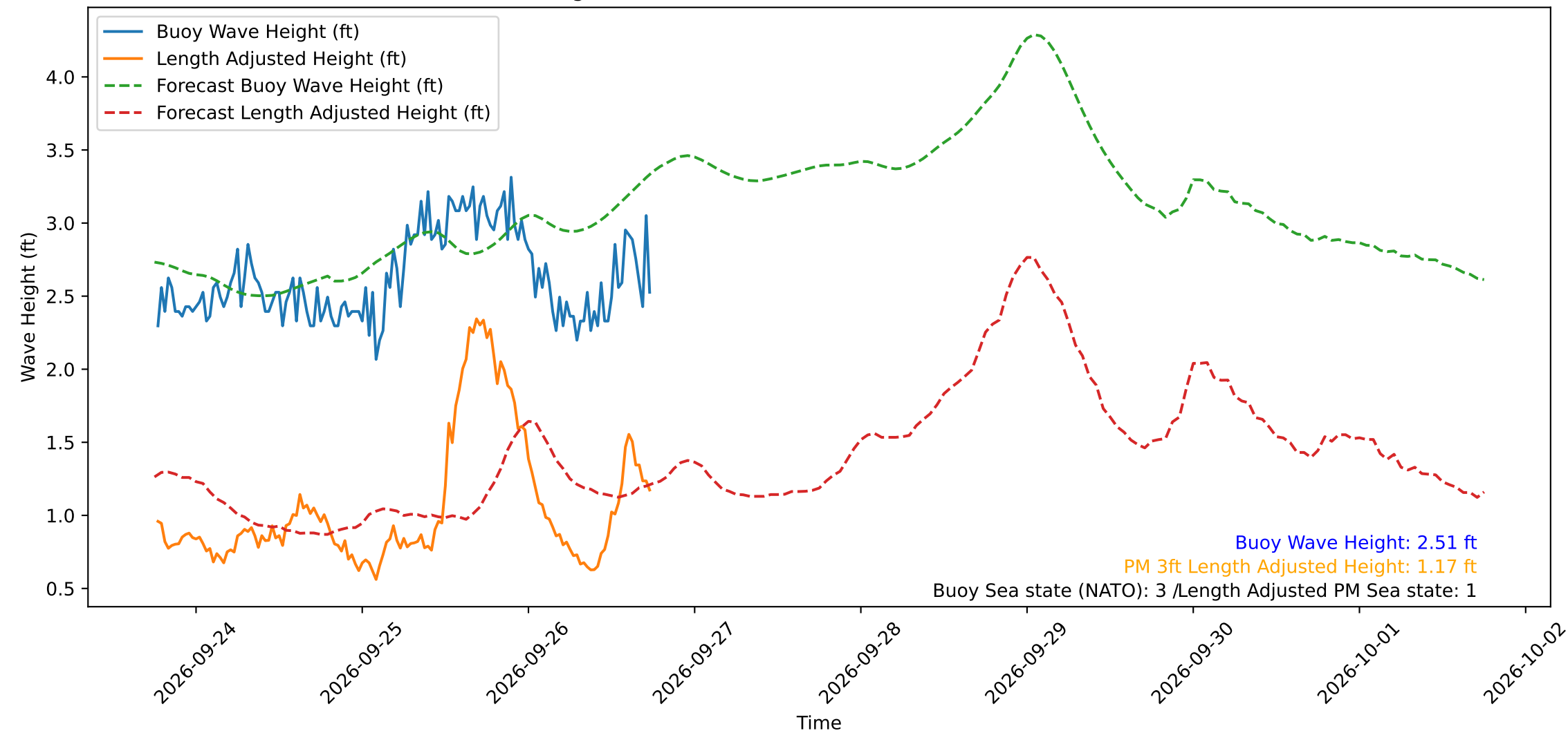
Wave Heights over Time for Red Beach at 2026-09-26 18:20:50
