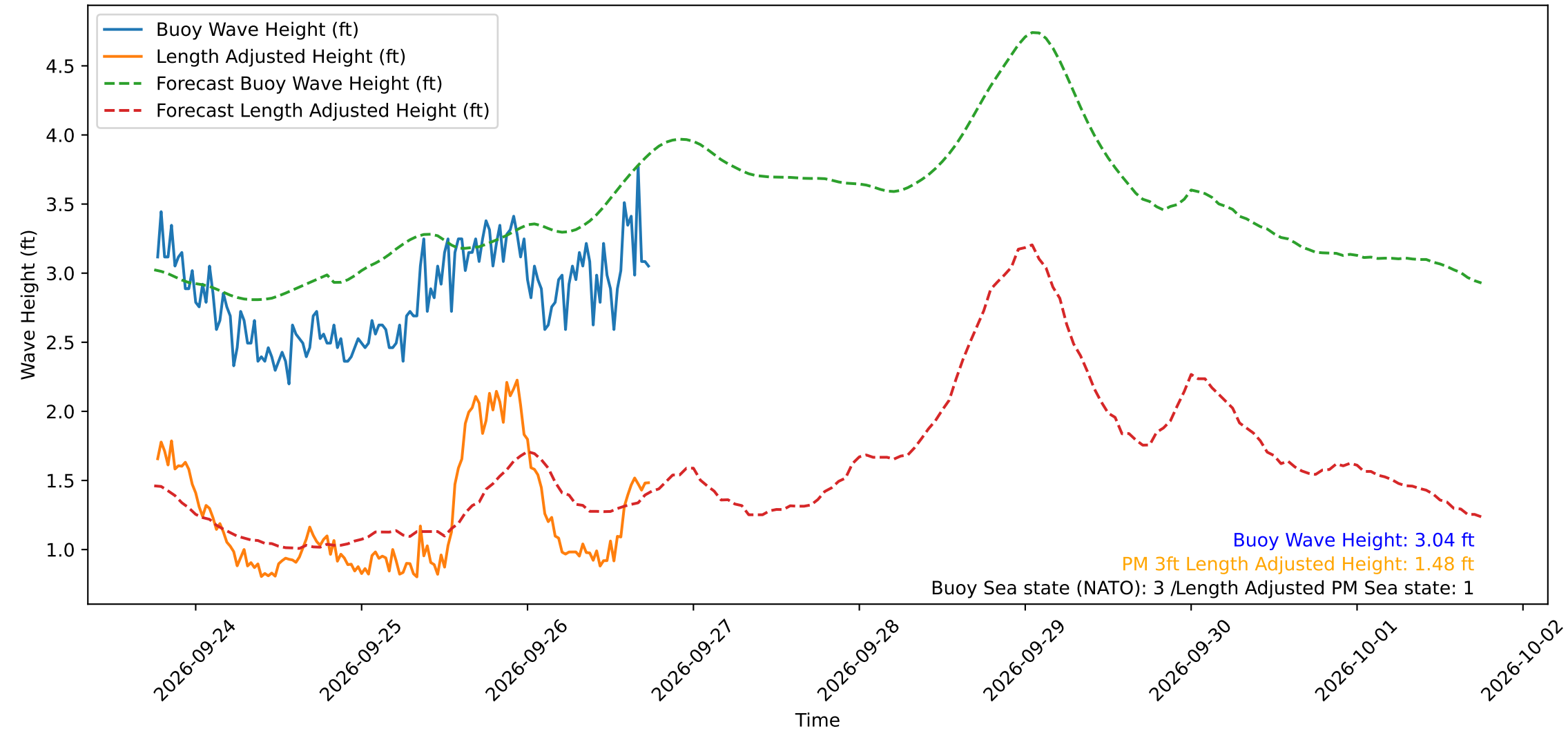
Wave Heights over Time for Oceanside Harbor at 2026-09-26 18:20:29
