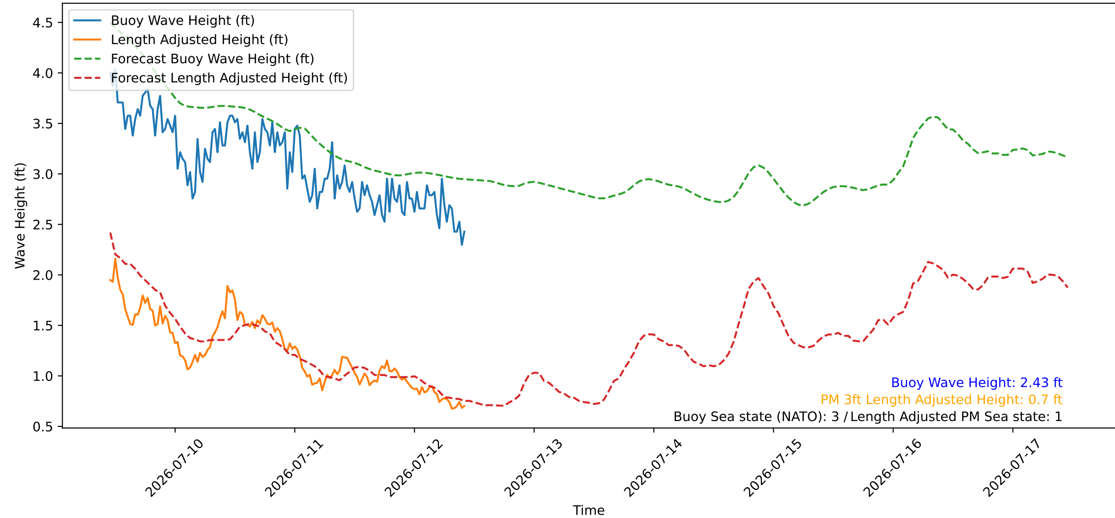
Wave Heights over Time for Green Beach at 2026-07-12 11:11:08
