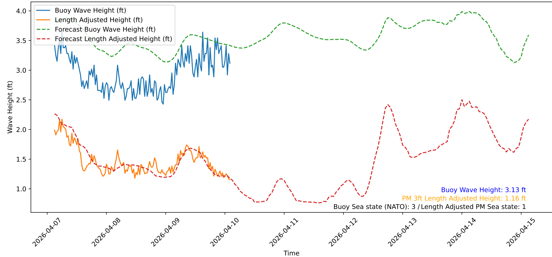
Wave Heights over Time for Oceanside Harbor at 2026-04-10 03:00:31
