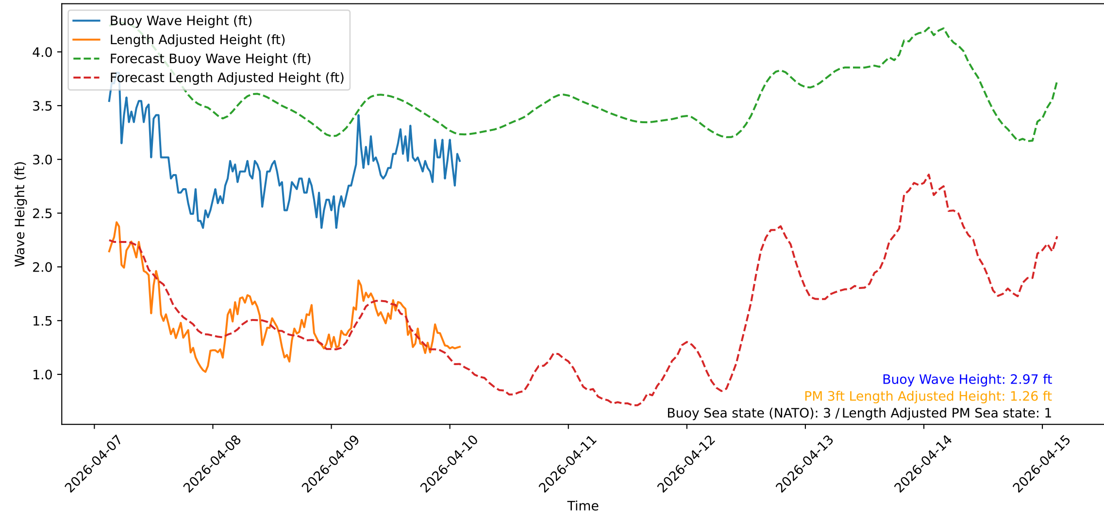
Wave Heights over Time for Green Beach at 2026-04-10 03:01:12
