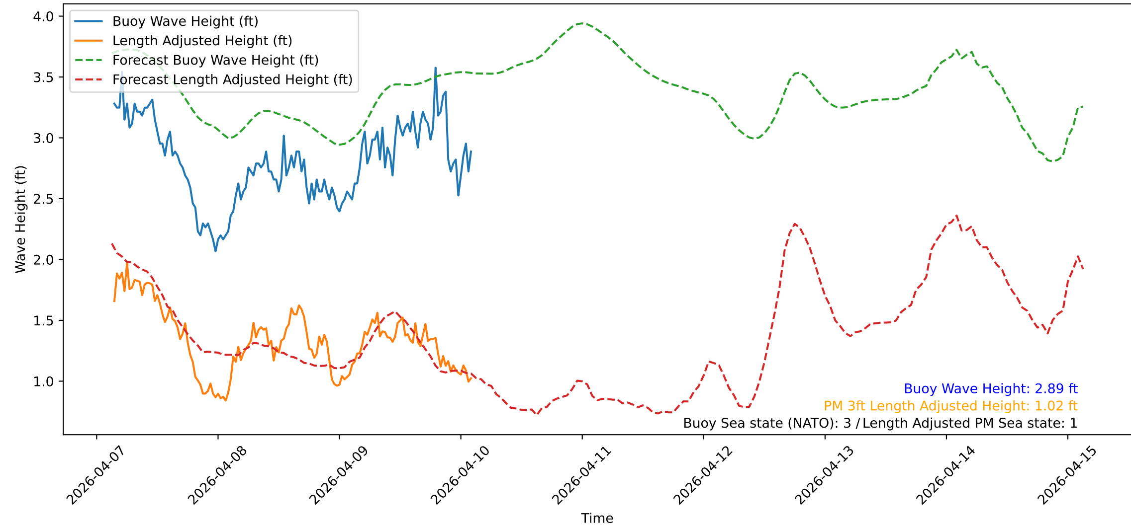
Wave Heights over Time for Red Beach at 2026-04-10 03:00:50
