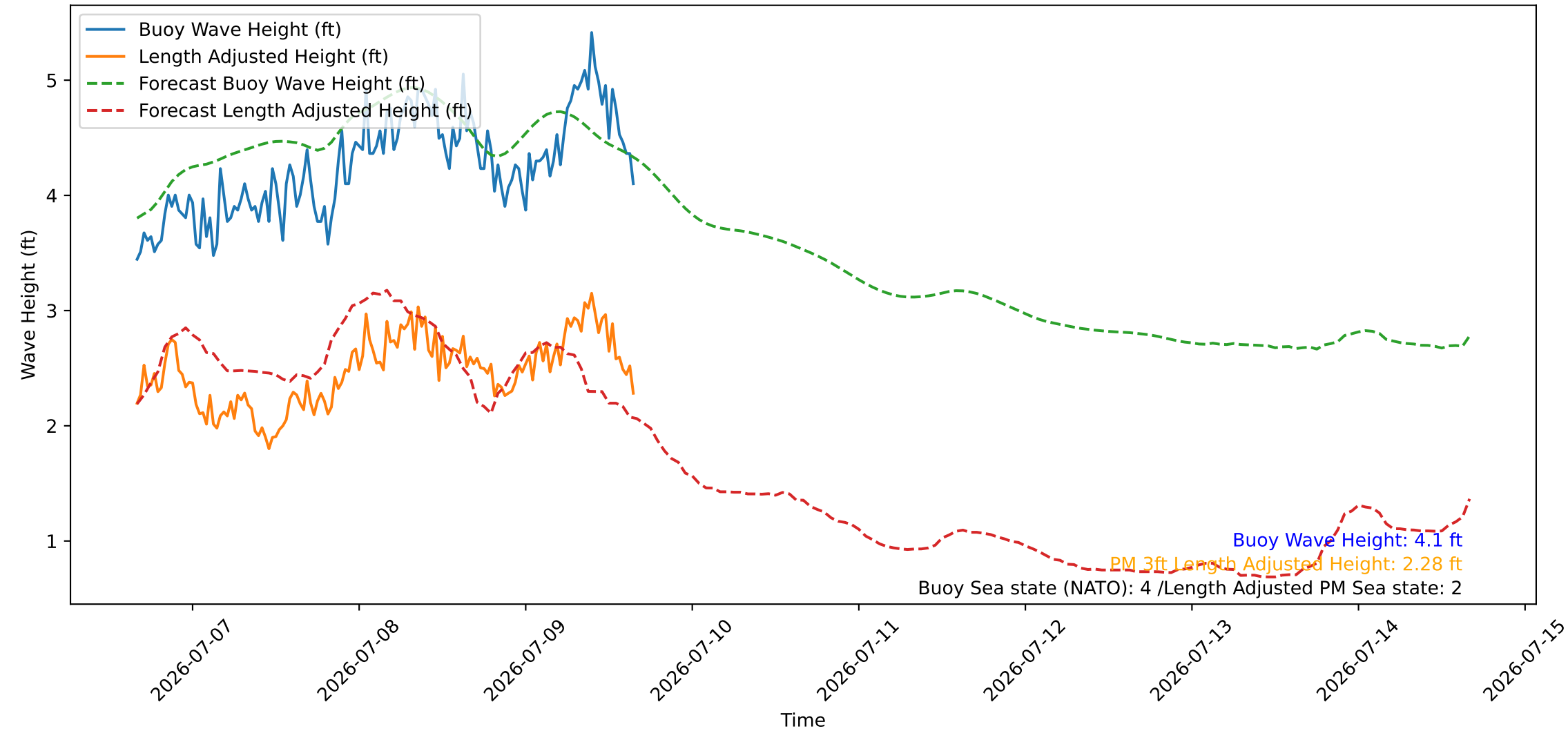
Wave Heights over Time for Oceanside Harbor at 2026-07-09 16:00:26
