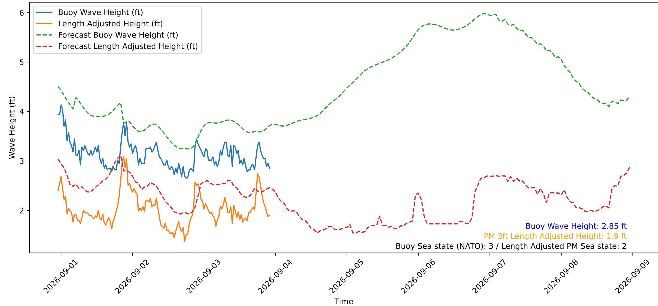
Wave Heights over Time for Green Beach at 2026-09-03 22:51:16
