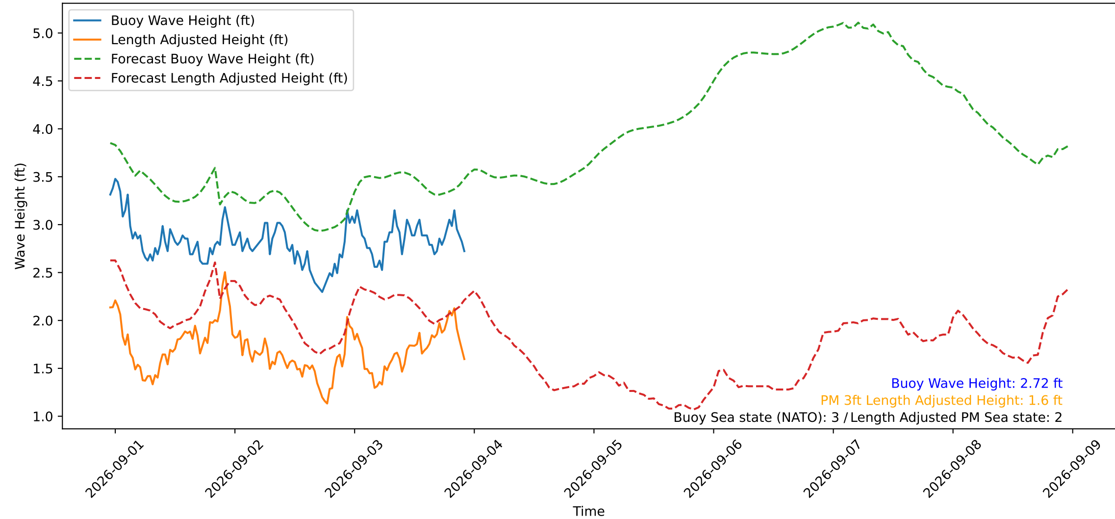
Wave Heights over Time for Red Beach at 2026-09-03 22:50:51
