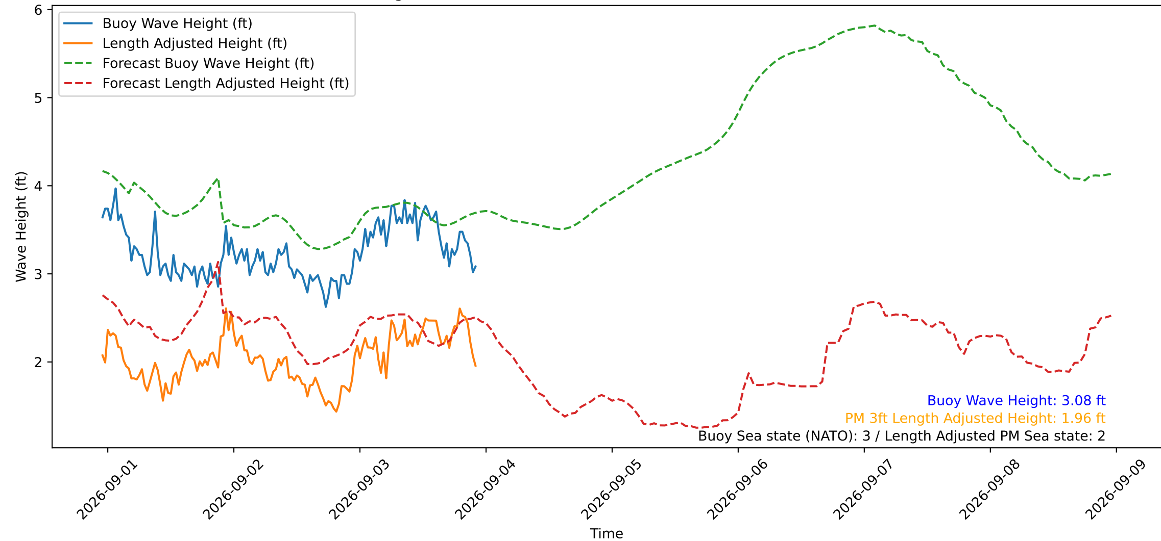
Wave Heights over Time for Oceanside Harbor at 2026-09-03 22:50:30
