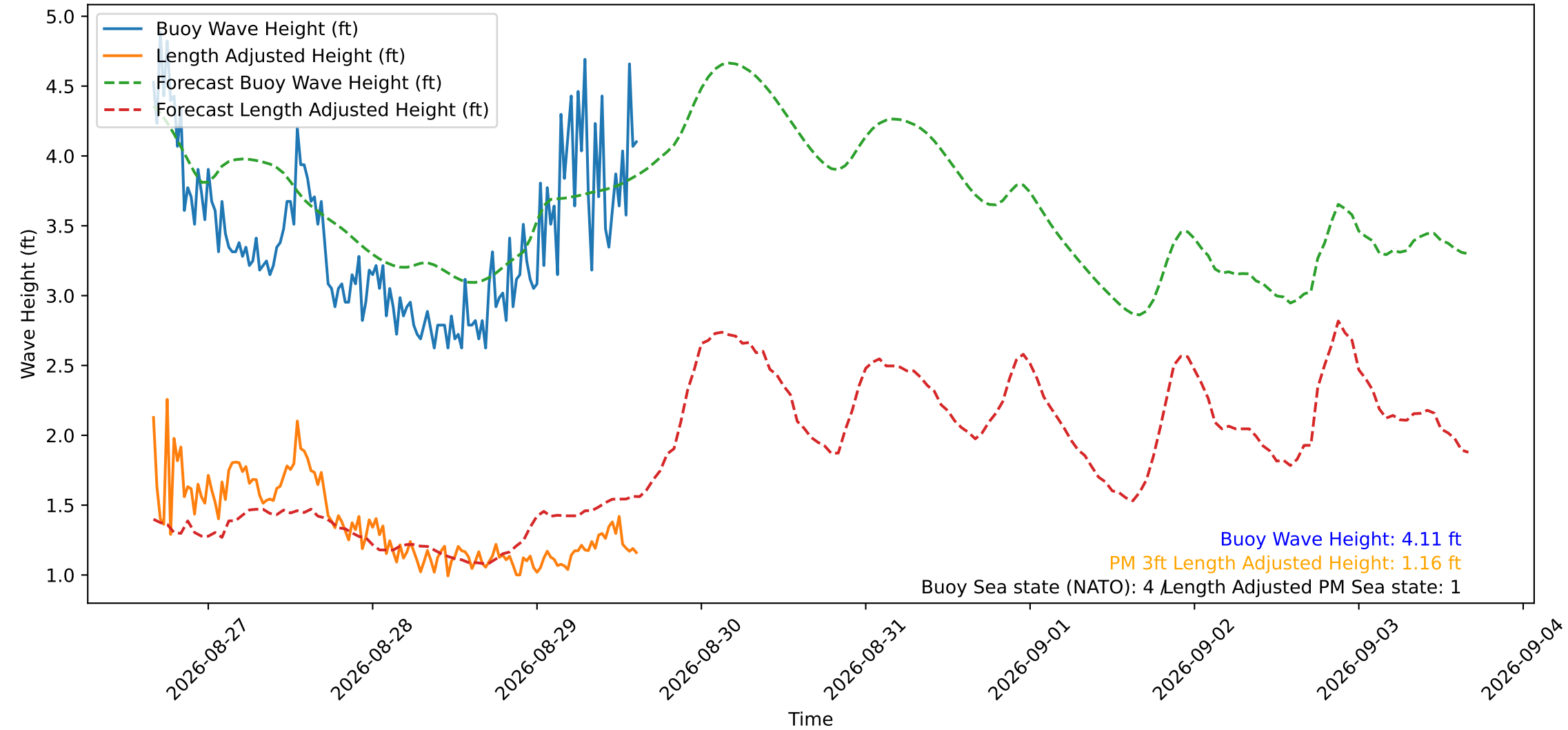
Wave Heights over Time for Red Beach at 2026-08-29 15:30:49
