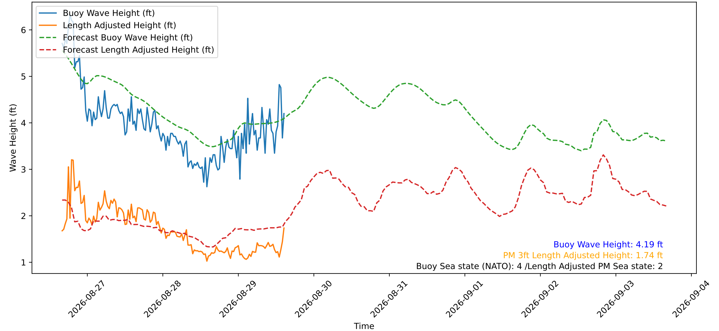
Wave Heights over Time for Green Beach at 2026-08-29 15:31:12
