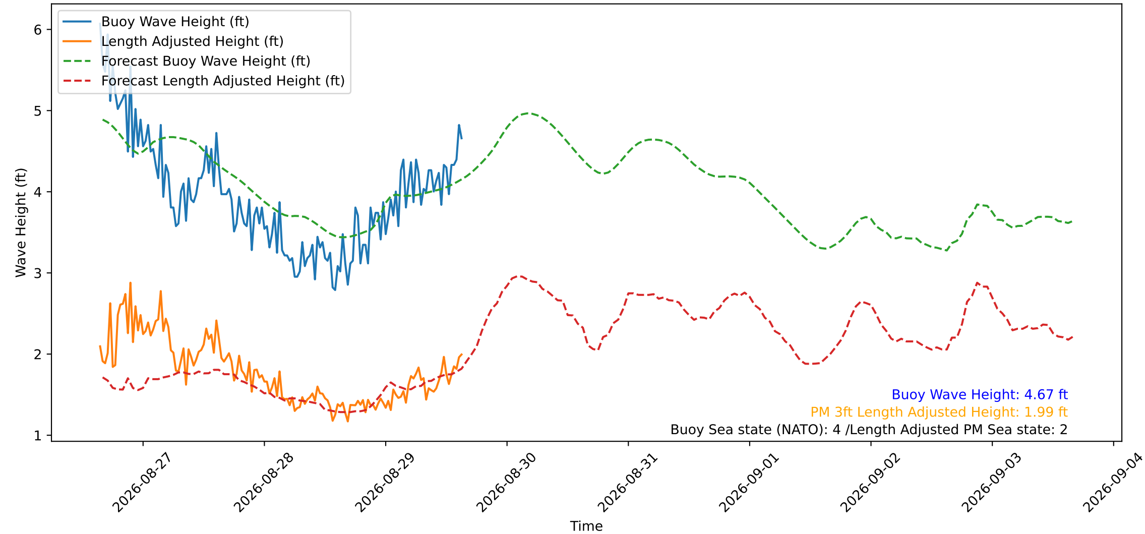
Wave Heights over Time for Oceanside Harbor at 2026-08-29 15:30:29
