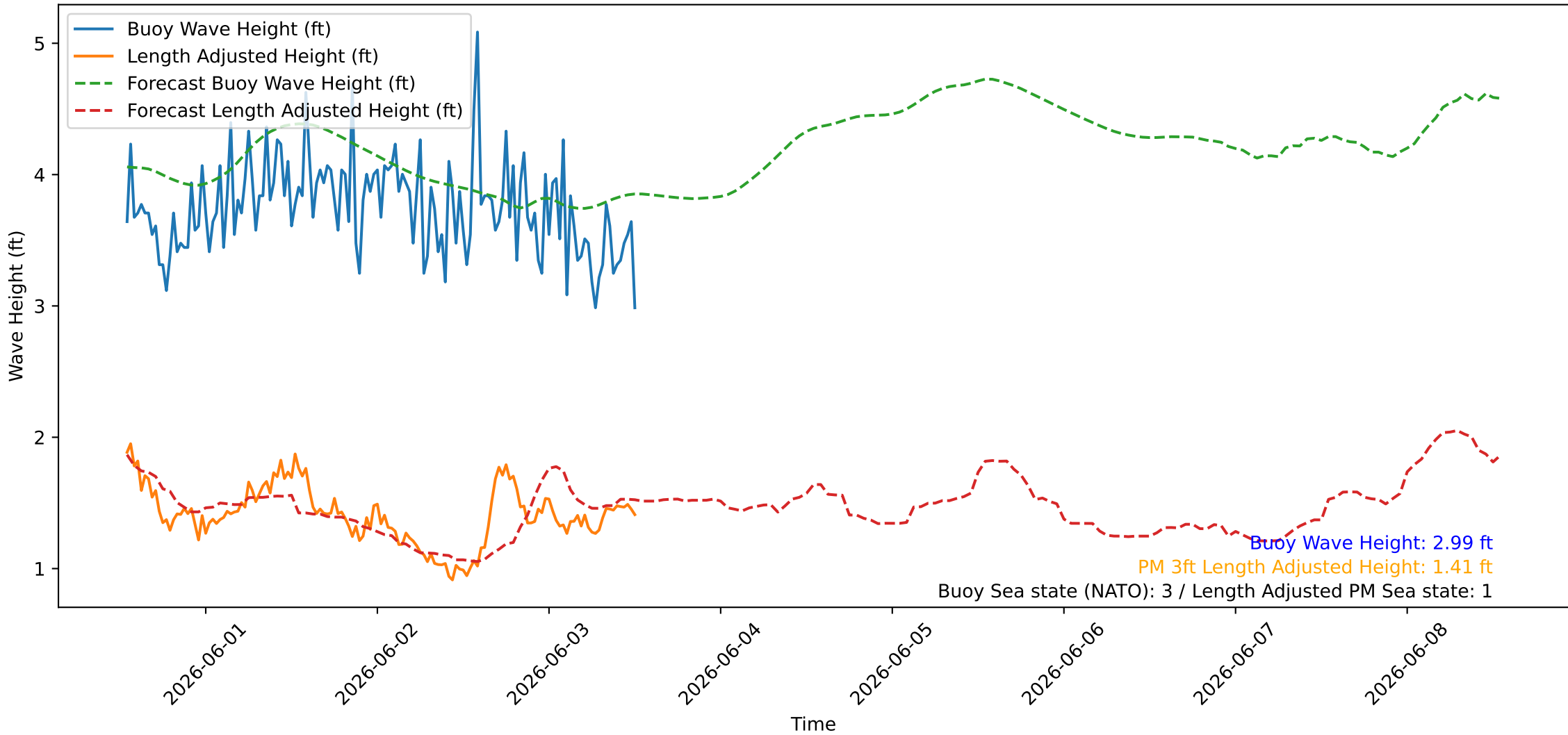
Wave Heights over Time for Oceanside Harbor at 2026-06-03 12:50:26
