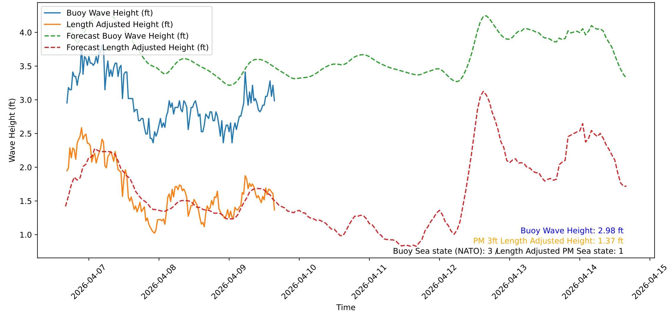
Wave Heights over Time for Green Beach at 2026-04-09 16:21:09
