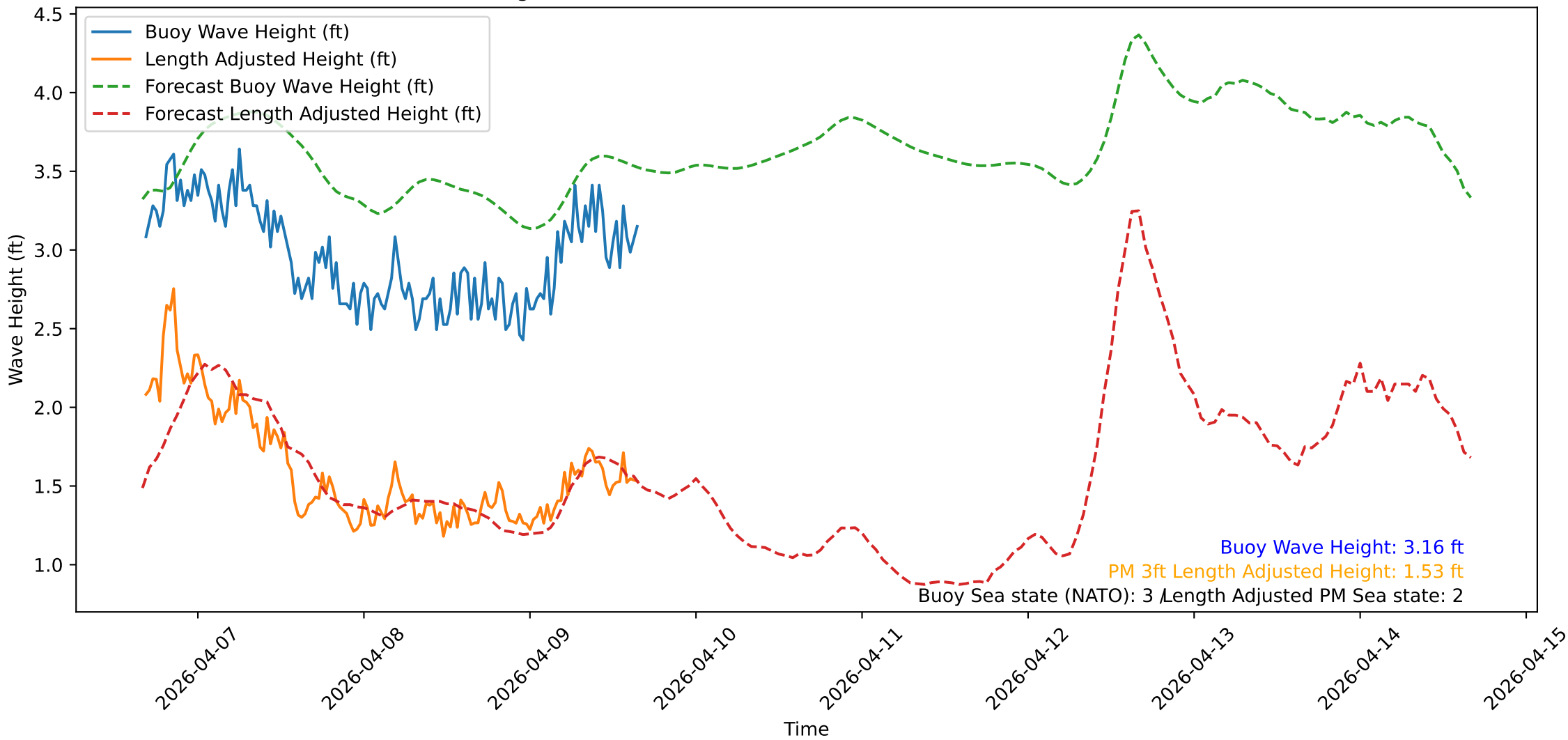
Wave Heights over Time for Oceanside Harbor at 2026-04-09 16:20:31
