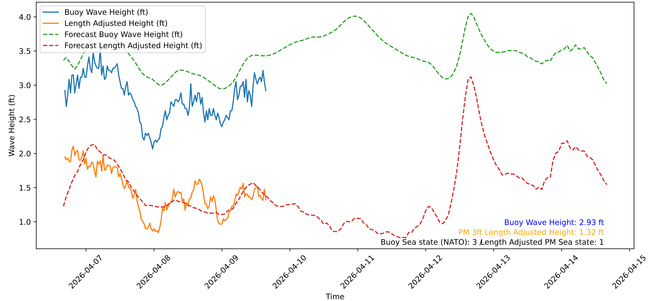
Wave Heights over Time for Red Beach at 2026-04-09 16:20:47
