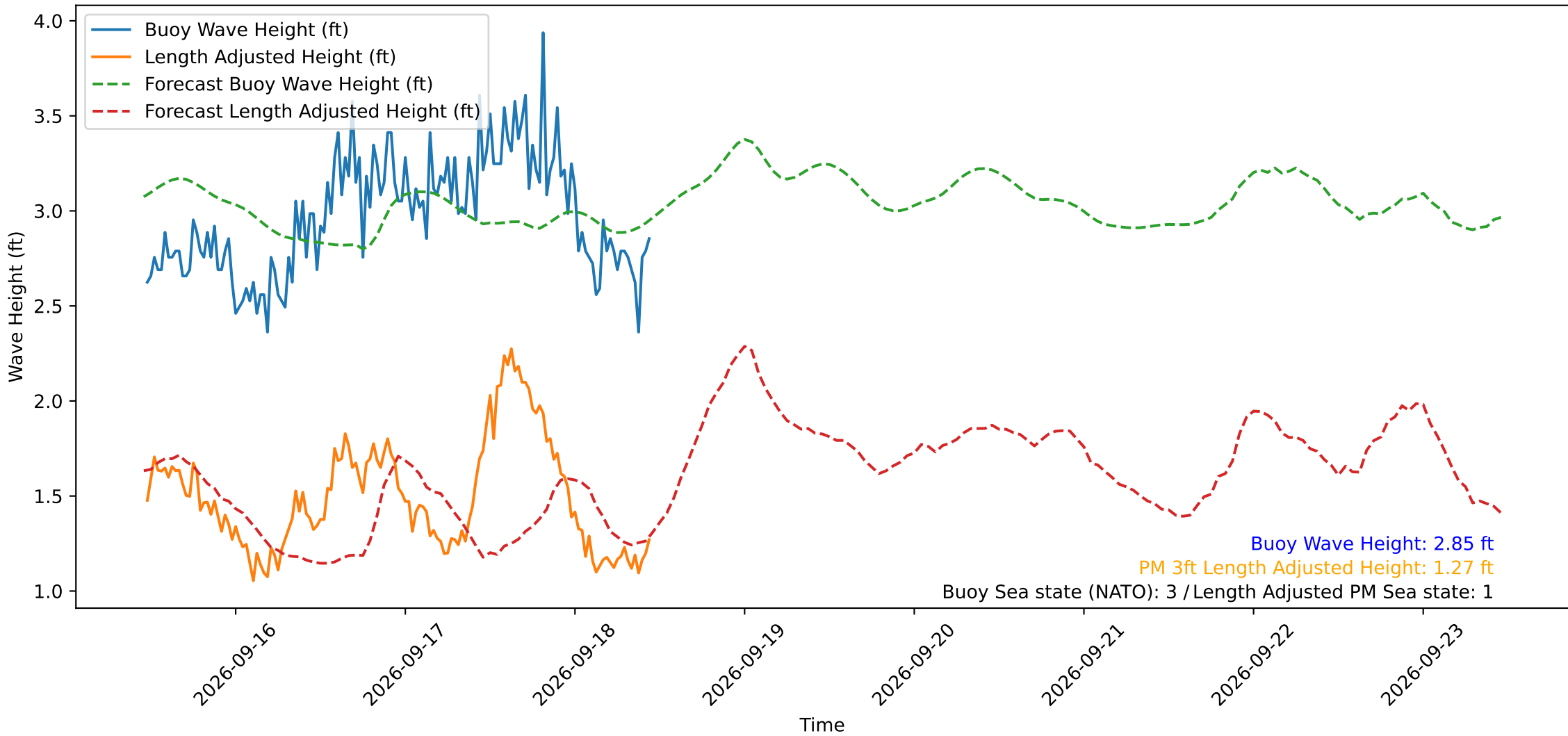
Wave Heights over Time for Oceanside Harbor at 2026-09-18 11:20:31
