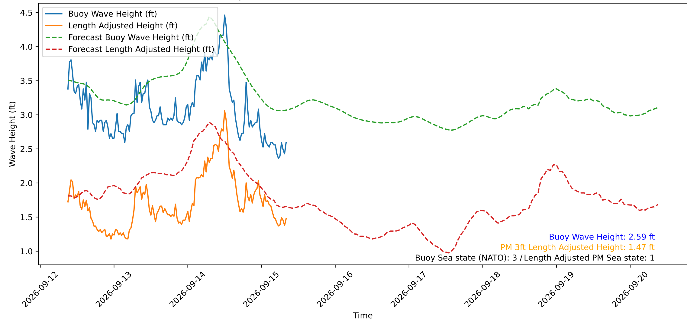
Wave Heights over Time for Oceanside Harbor at 2026-09-15 08:50:29
