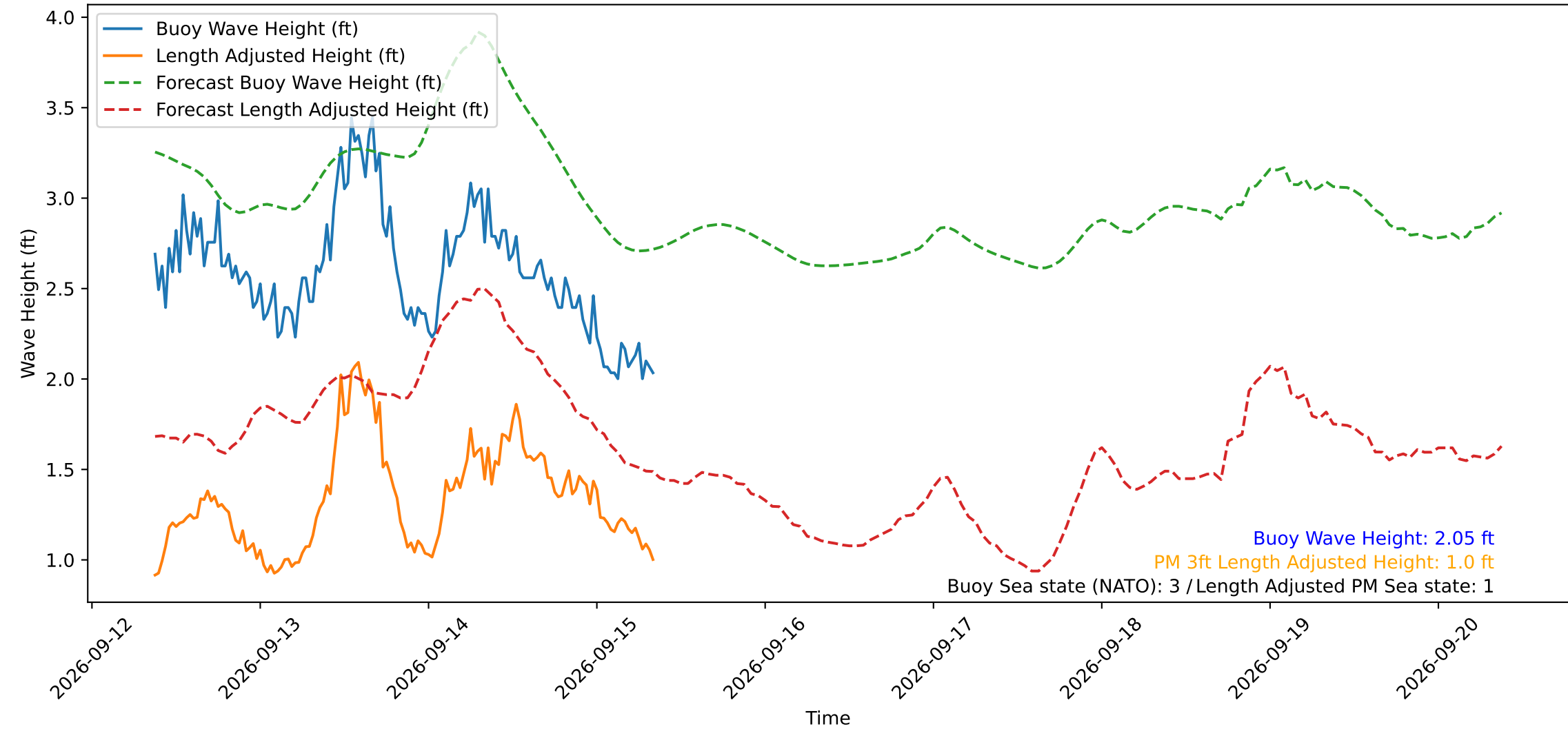
Wave Heights over Time for Red Beach at 2026-09-15 08:50:50
