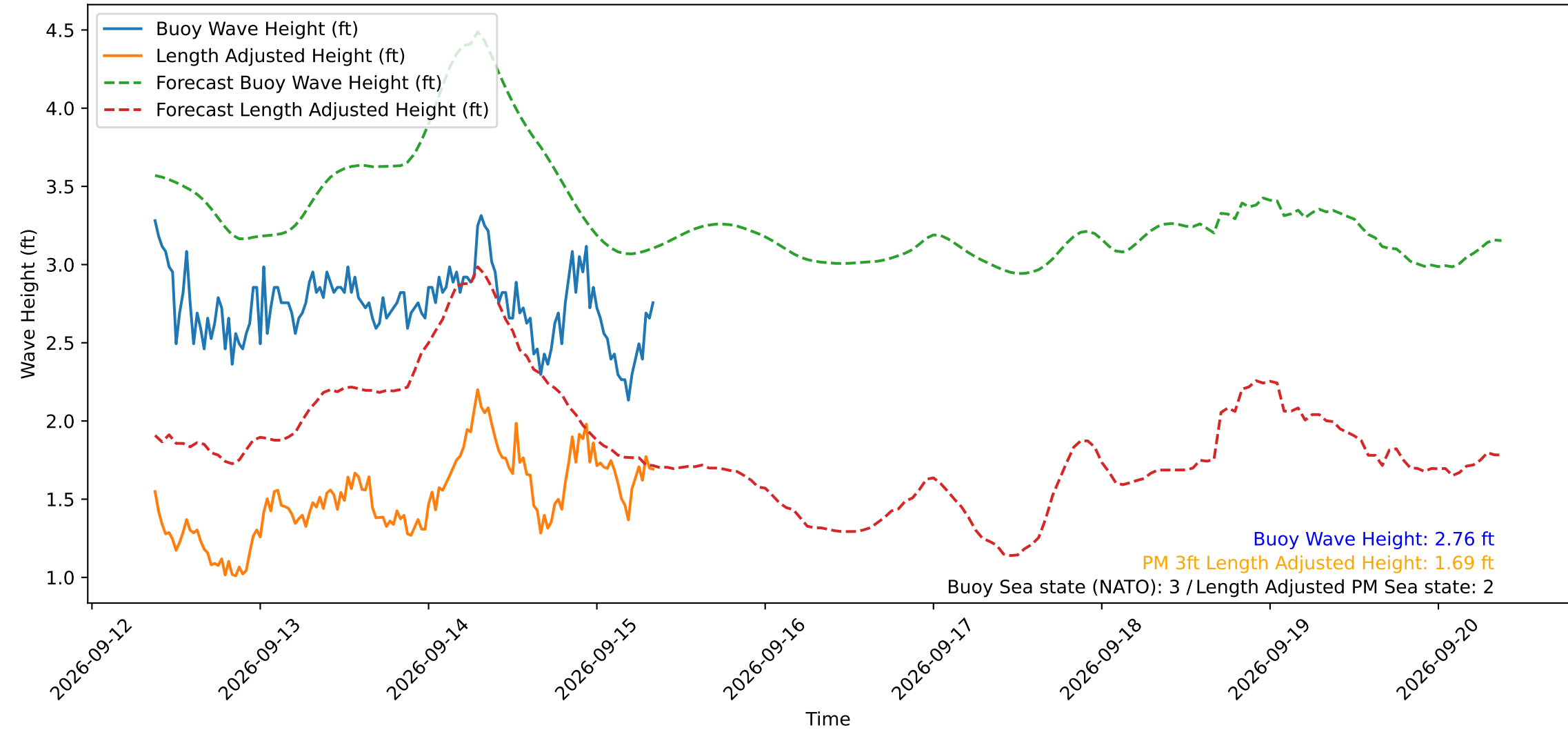
Wave Heights over Time for Green Beach at 2026-09-15 08:51:14
