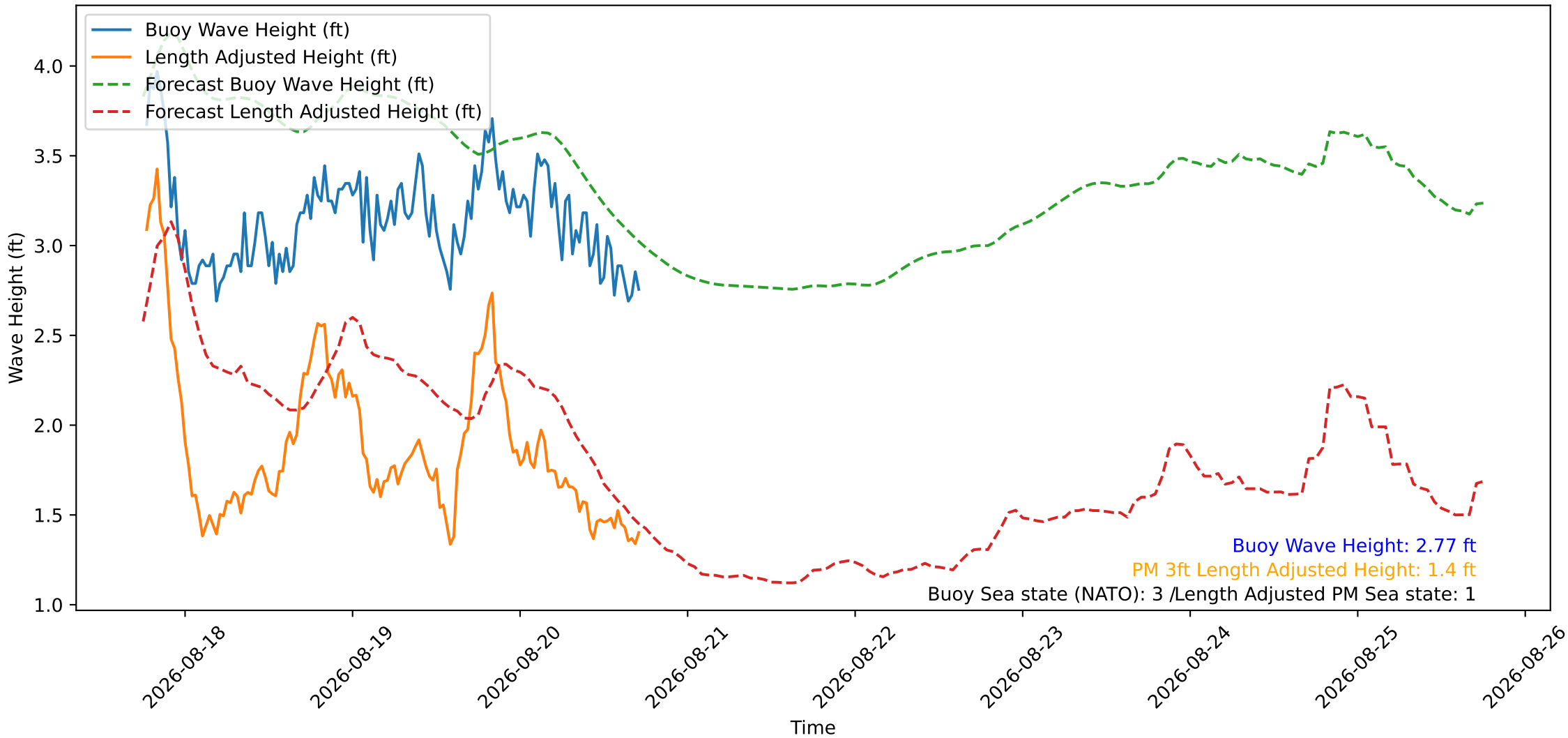
Wave Heights over Time for Green Beach at 2026-08-20 18:01:08
