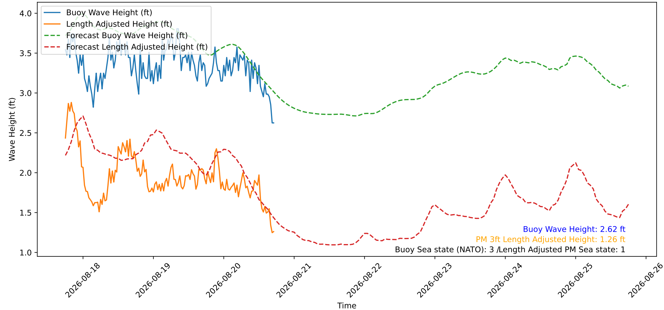
Wave Heights over Time for Oceanside Harbor at 2026-08-20 18:00:26
