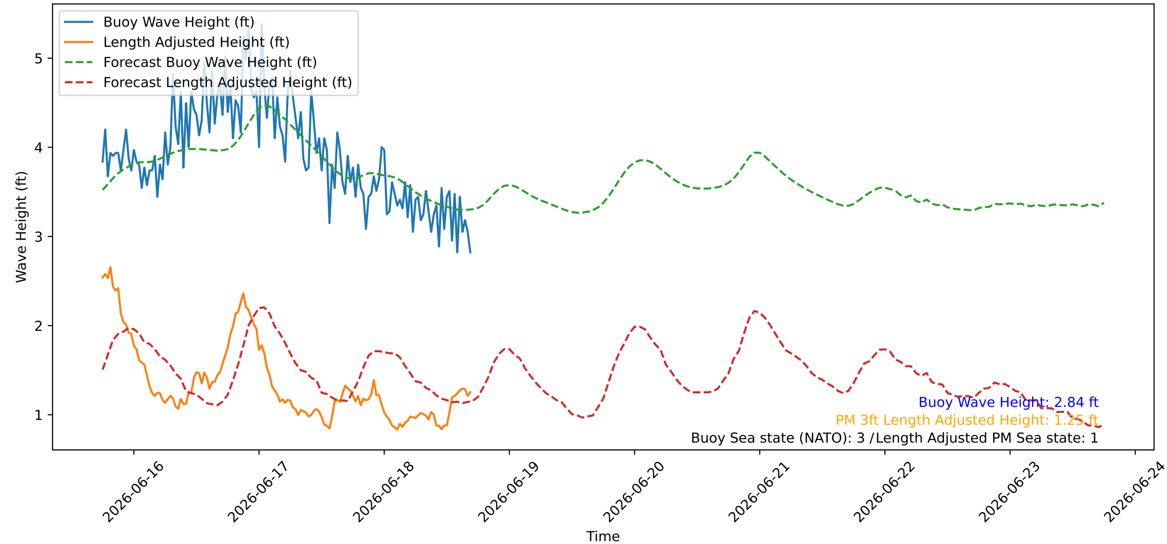
Wave Heights over Time for Red Beach at 2026-06-18 17:30:45
