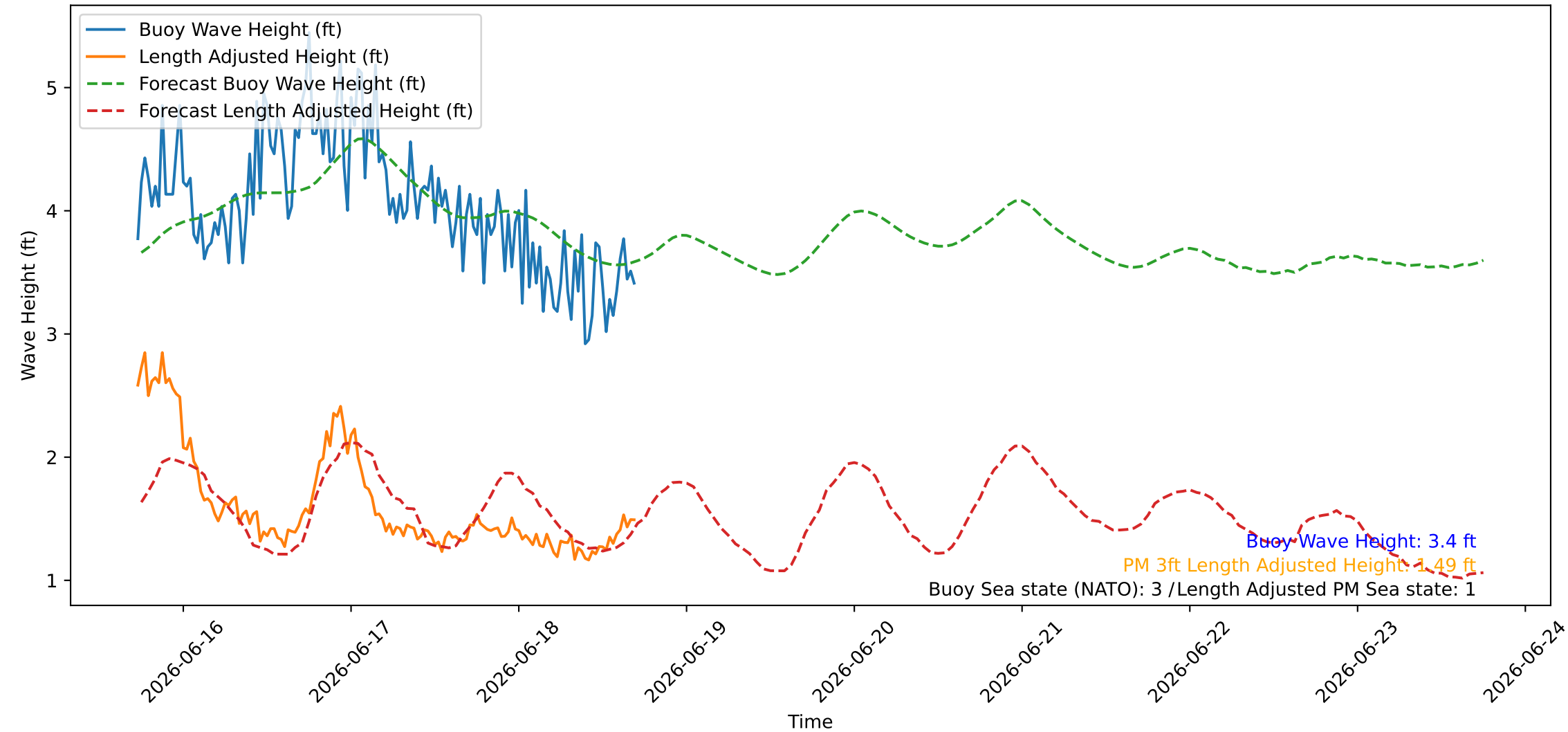
Wave Heights over Time for Oceanside Harbor at 2026-06-18 17:30:26
