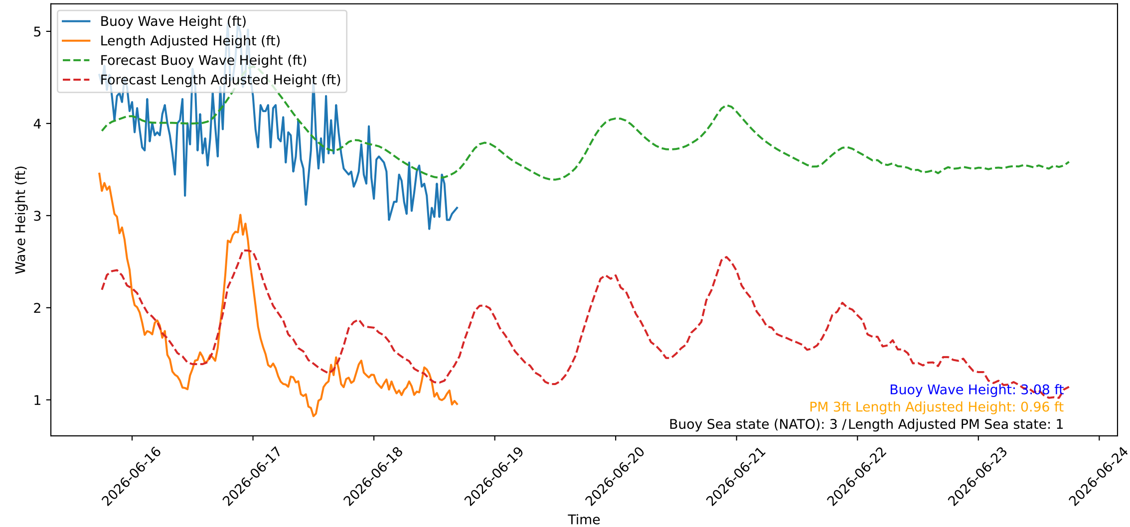
Wave Heights over Time for Green Beach at 2026-06-18 17:31:07
