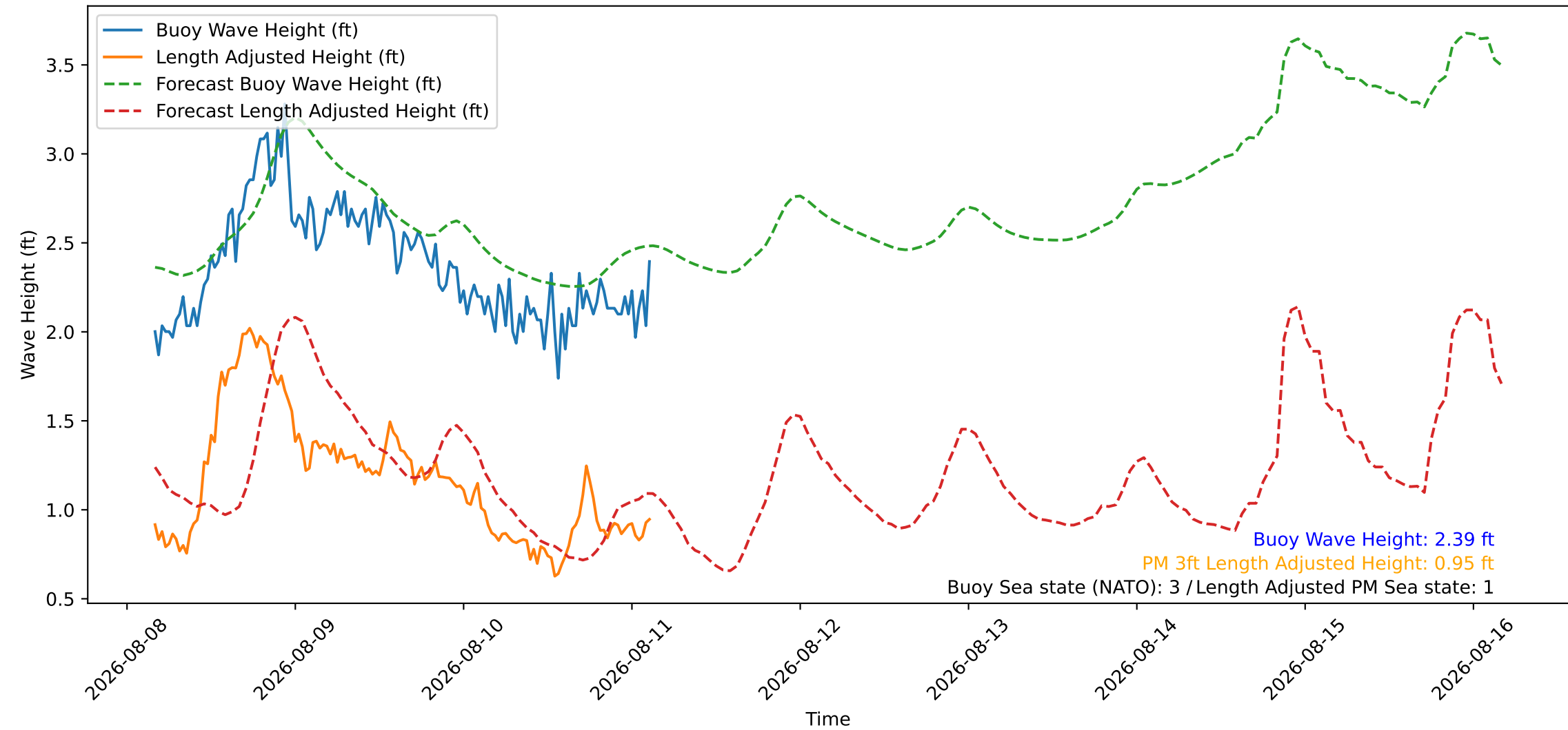
Wave Heights over Time for Red Beach at 2026-08-11 03:30:46
