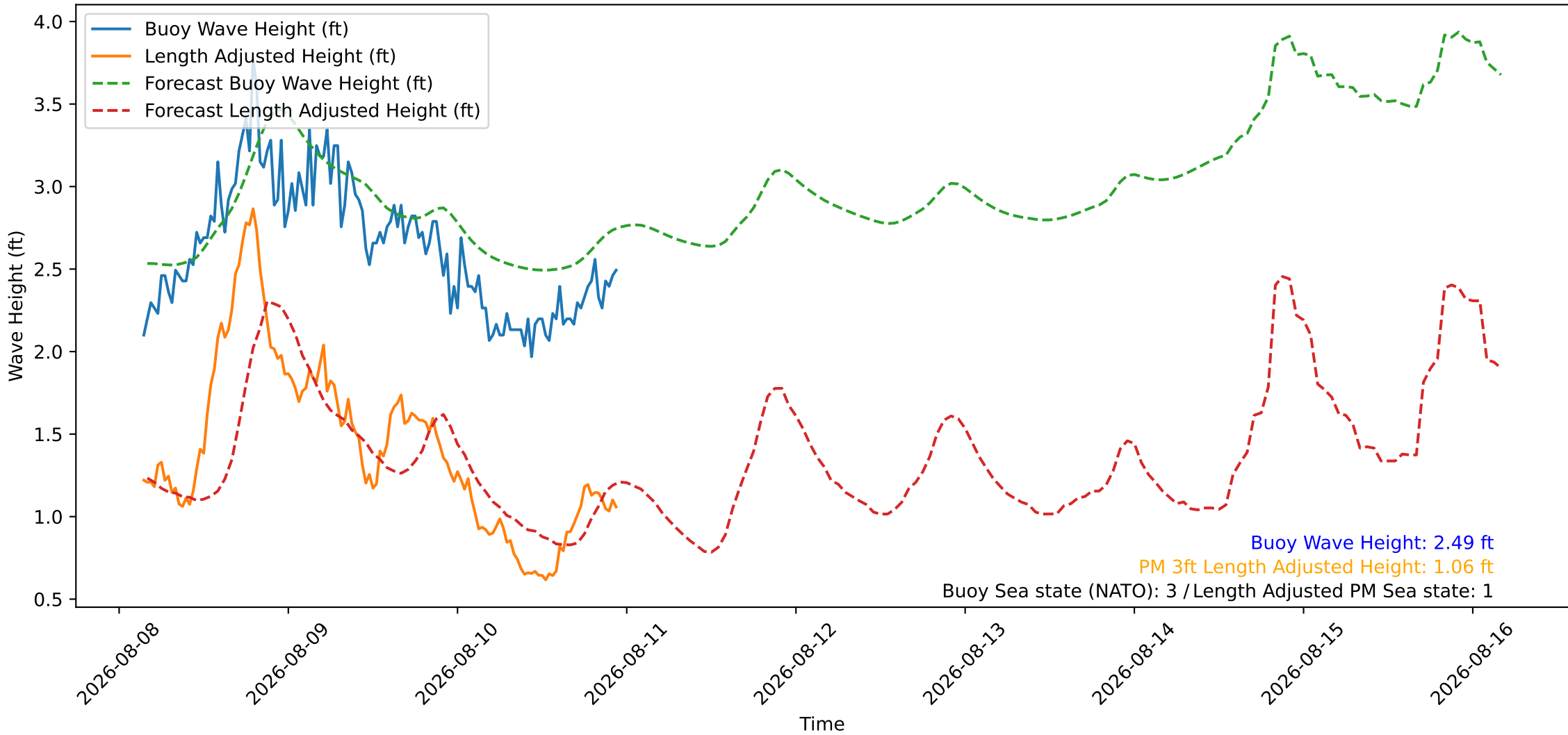
Wave Heights over Time for Green Beach at 2026-08-11 03:31:08
