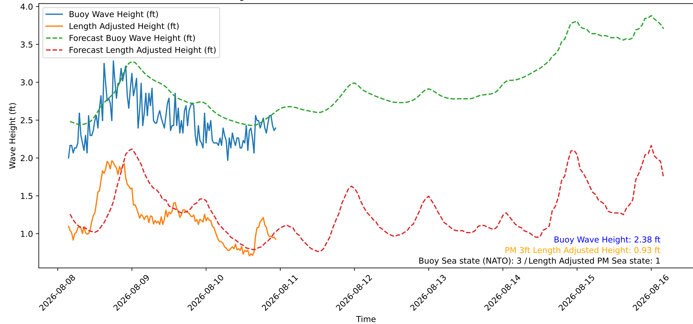
Wave Heights over Time for Oceanside Harbor at 2026-08-11 03:30:26
