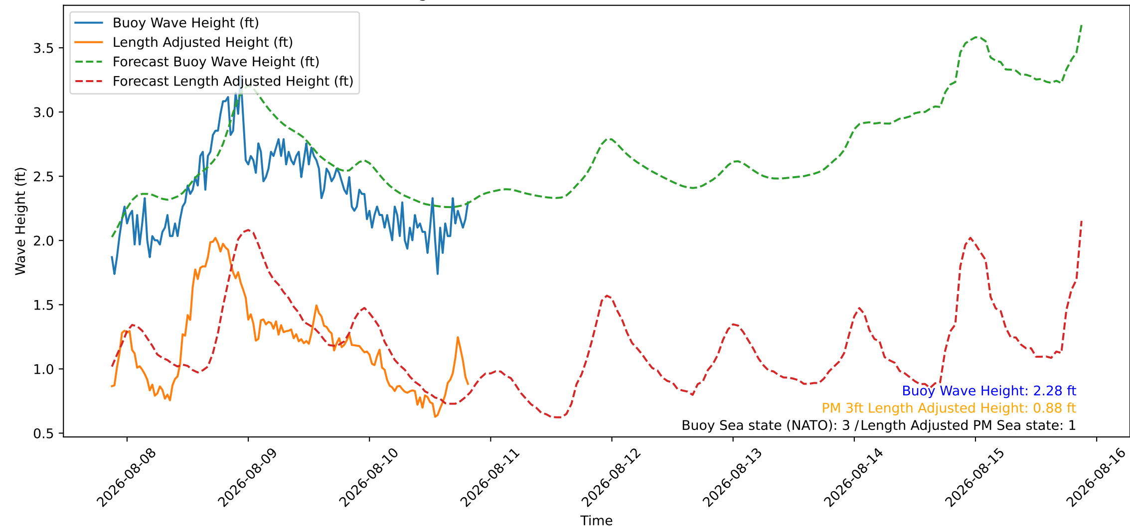
Wave Heights over Time for Red Beach at 2026-08-10 20:30:46
