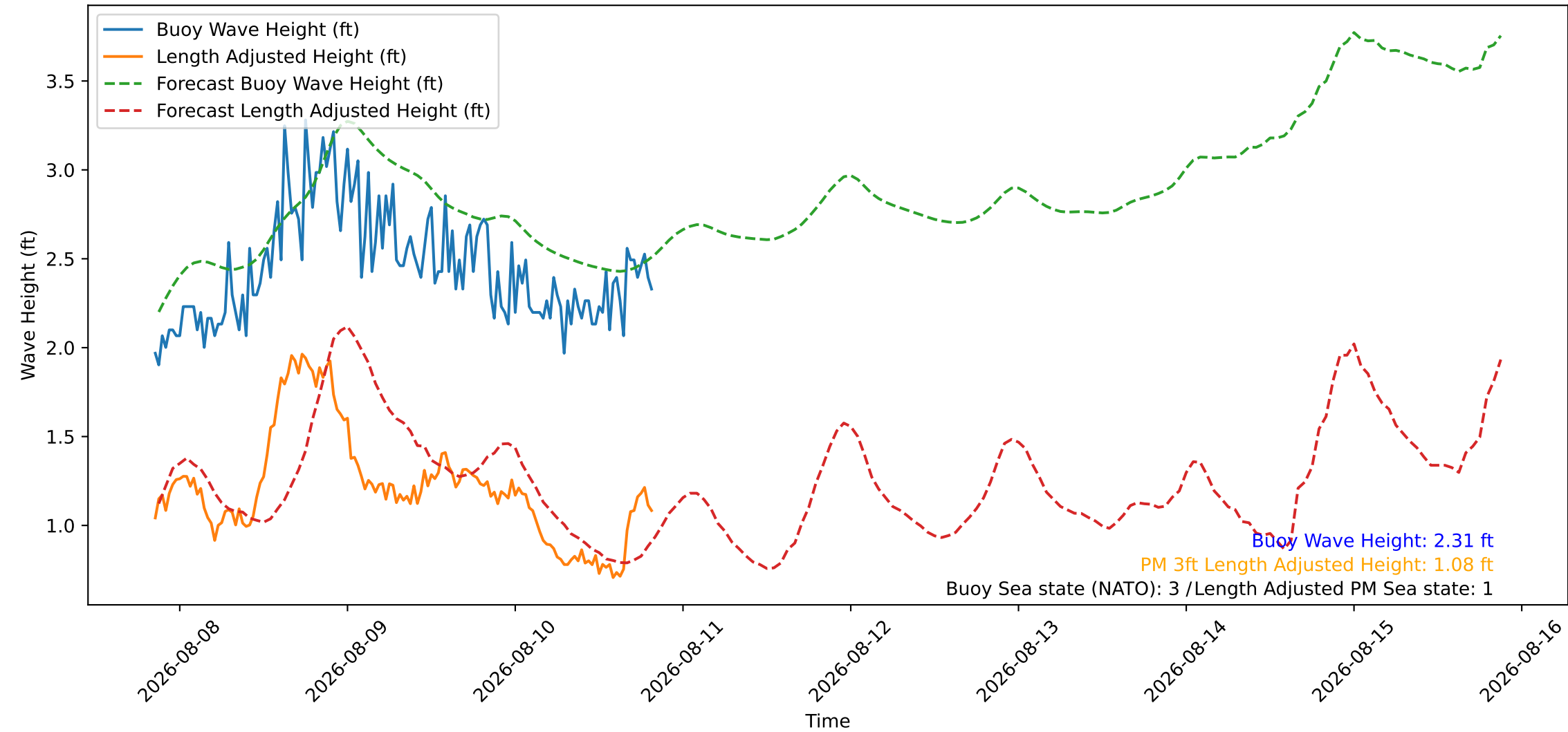
Wave Heights over Time for Oceanside Harbor at 2026-08-10 20:30:26
