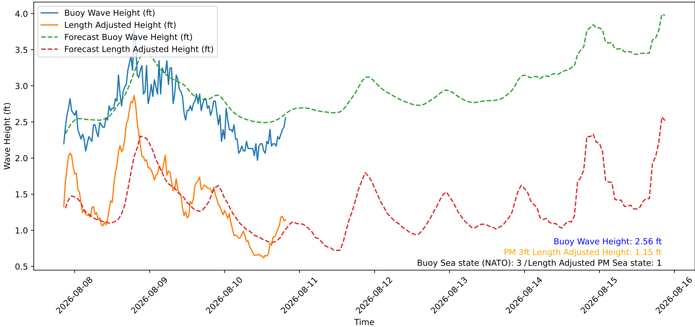
Wave Heights over Time for Green Beach at 2026-08-10 20:31:09
