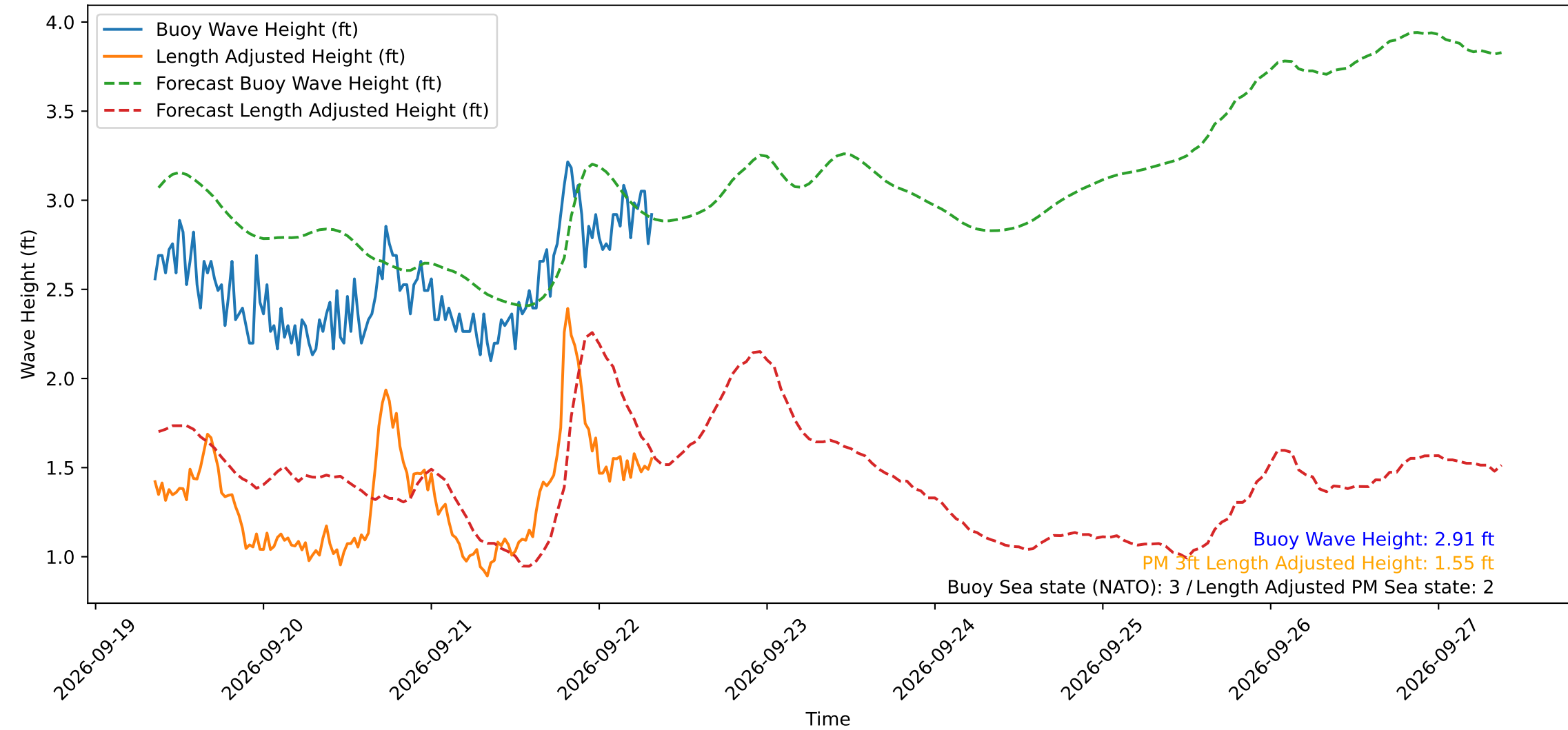
Wave Heights over Time for Oceanside Harbor at 2026-09-22 08:30:30
