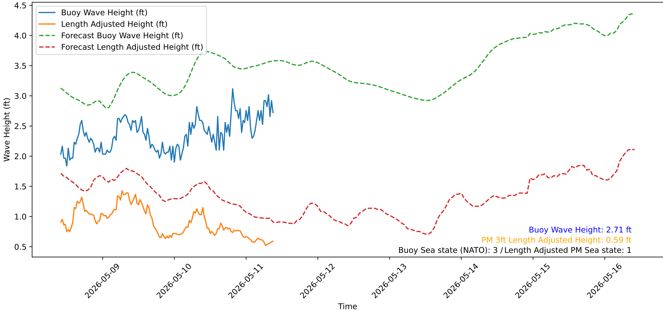
Wave Heights over Time for Green Beach at 2026-05-11 10:01:12
