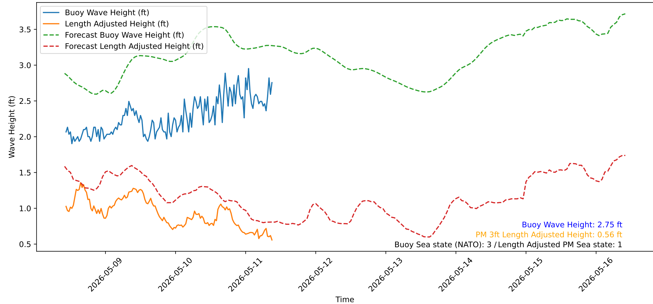
Wave Heights over Time for Red Beach at 2026-05-11 10:00:50
