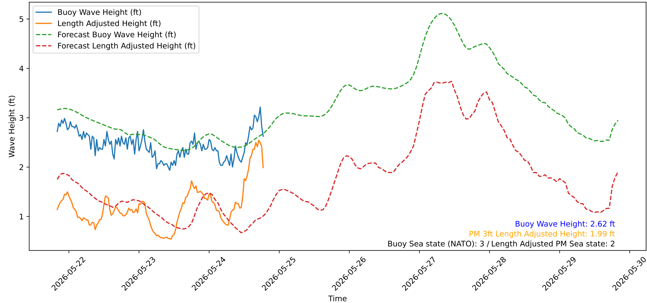
Wave Heights over Time for Red Beach at 2026-05-24 19:30:52
