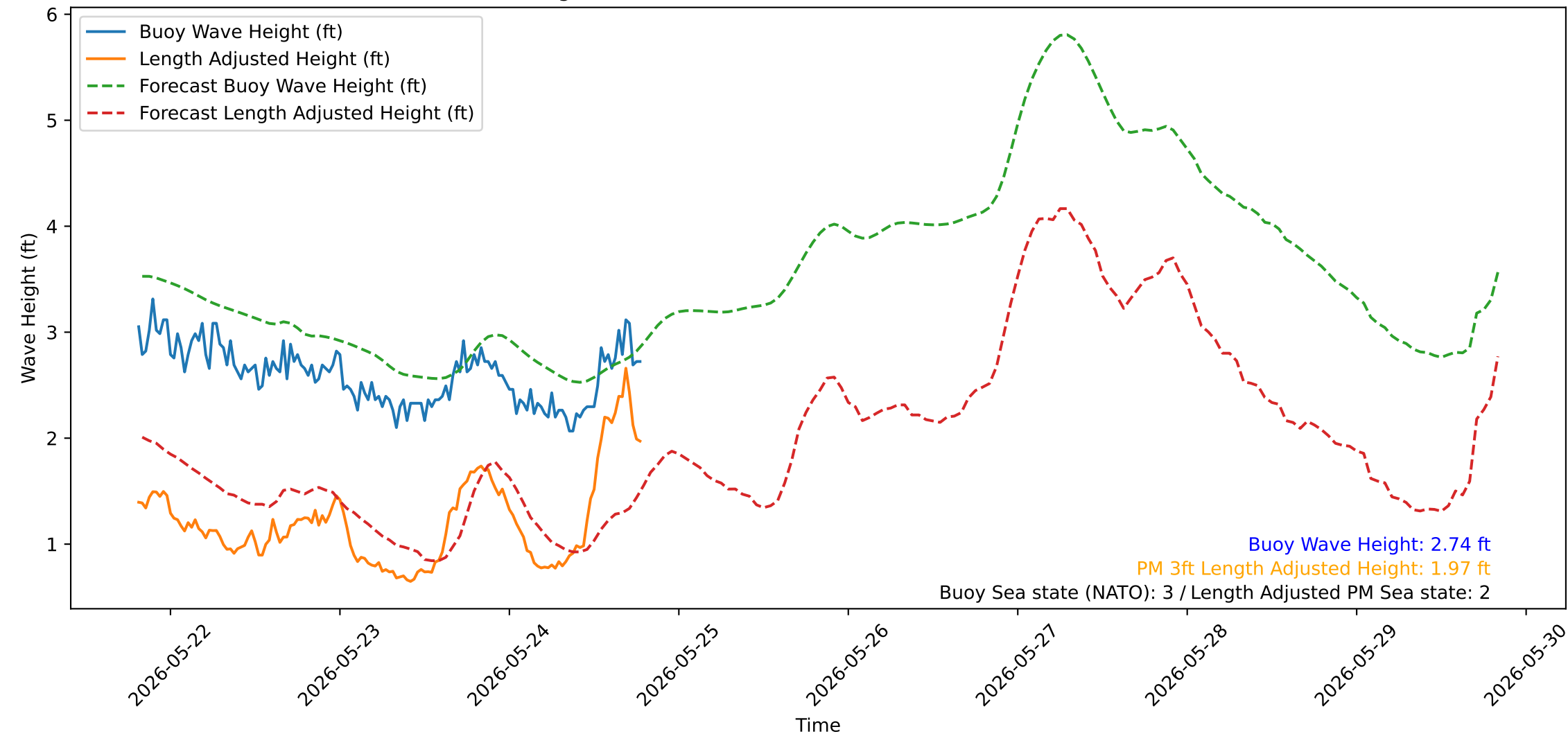
Wave Heights over Time for Green Beach at 2026-05-24 19:31:15
