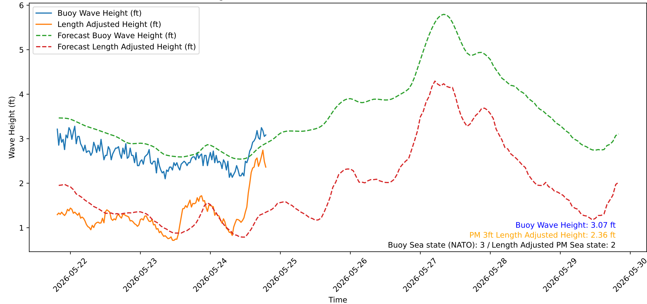
Wave Heights over Time for Oceanside Harbor at 2026-05-24 19:30:32
