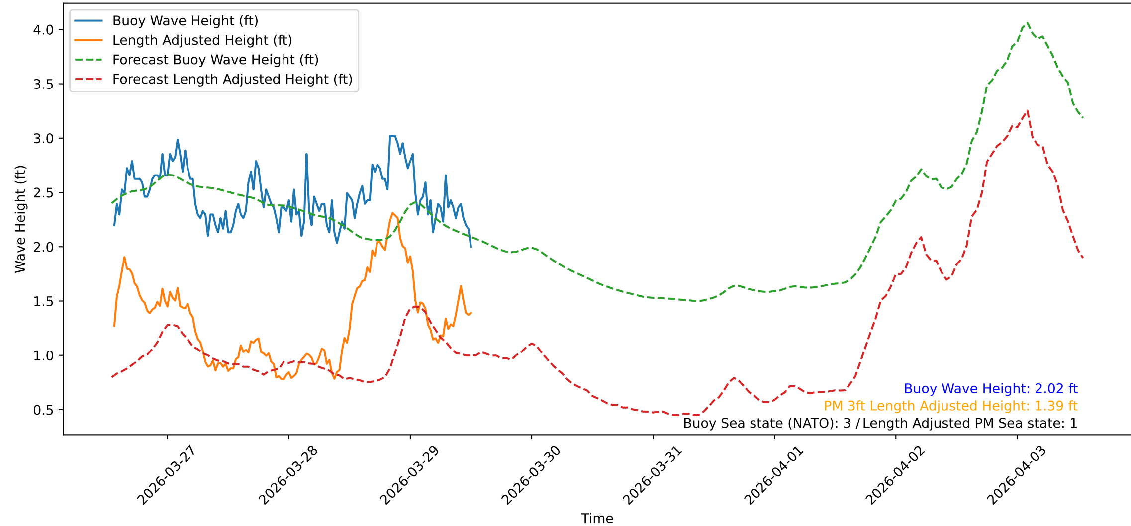
Wave Heights over Time for Red Beach at 2026-03-29 13:00:47
