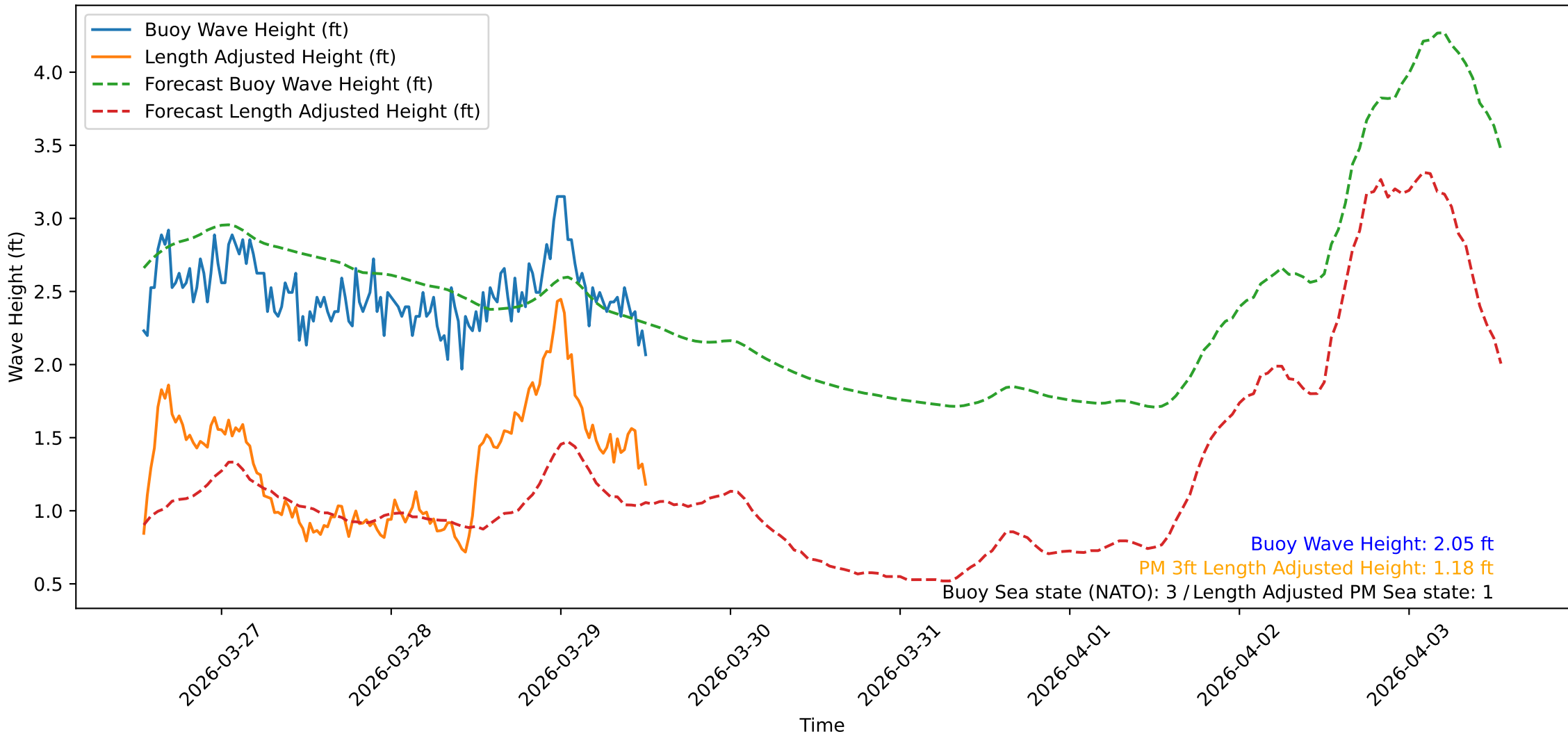
Wave Heights over Time for Oceanside Harbor at 2026-03-29 13:00:32
