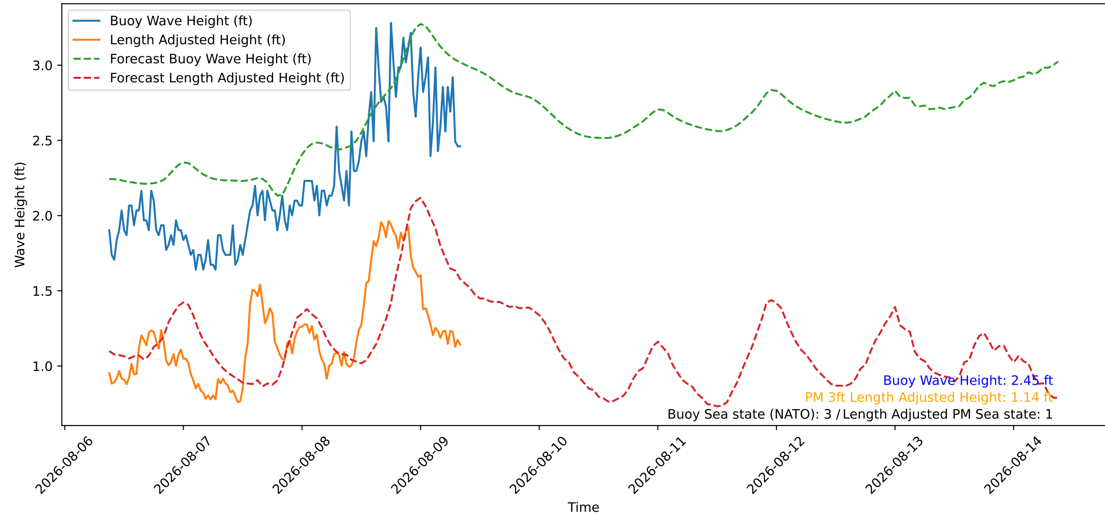
Wave Heights over Time for Oceanside Harbor at 2026-08-09 08:50:26
