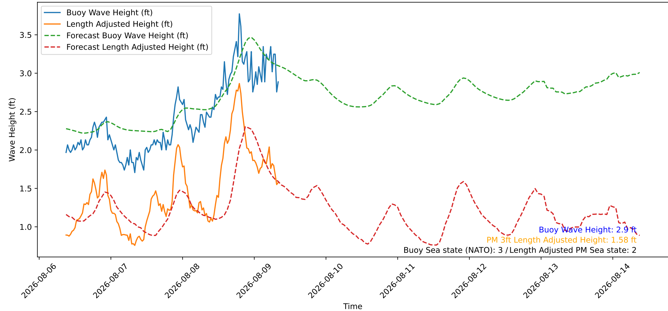
Wave Heights over Time for Green Beach at 2026-08-09 08:51:09
