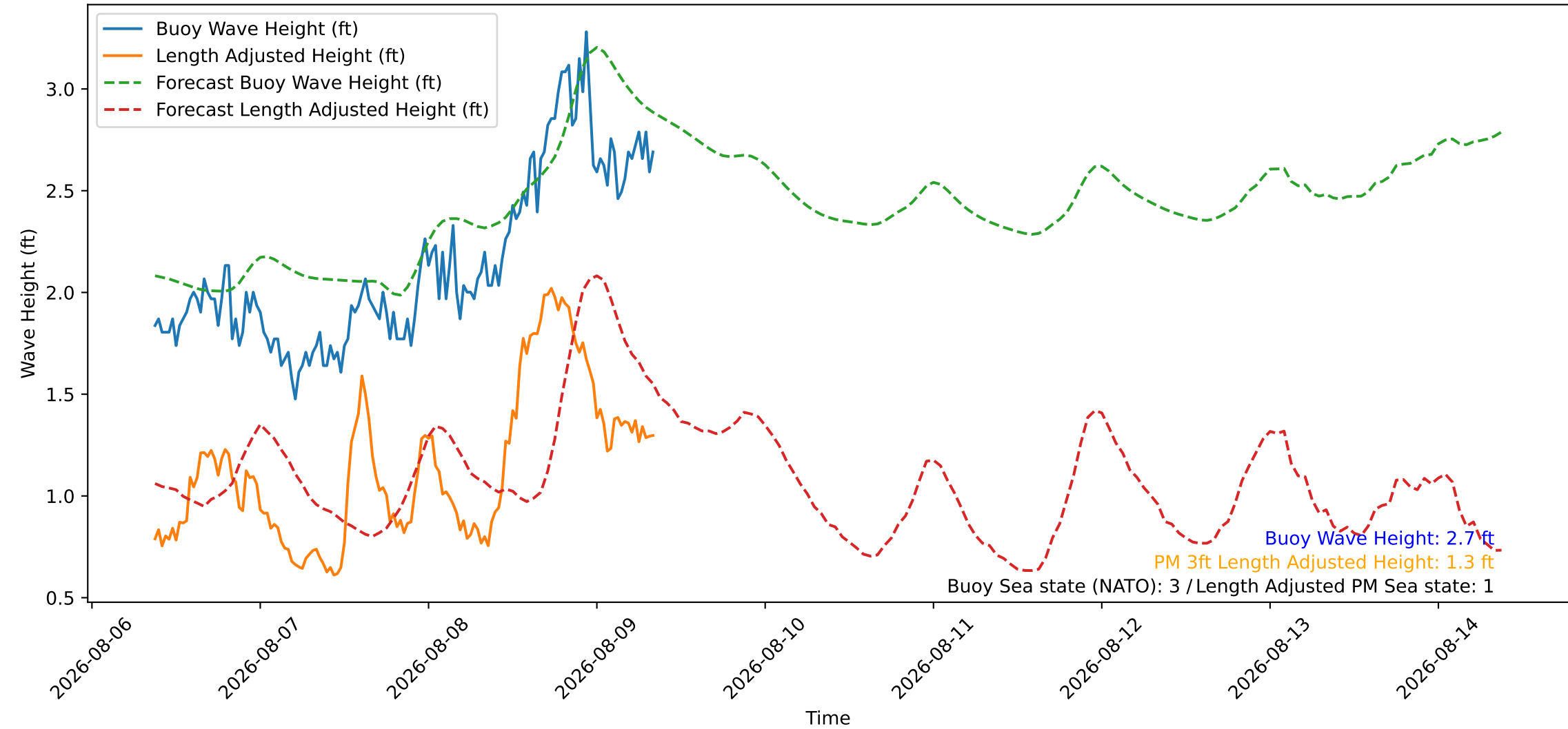
Wave Heights over Time for Red Beach at 2026-08-09 08:50:47
