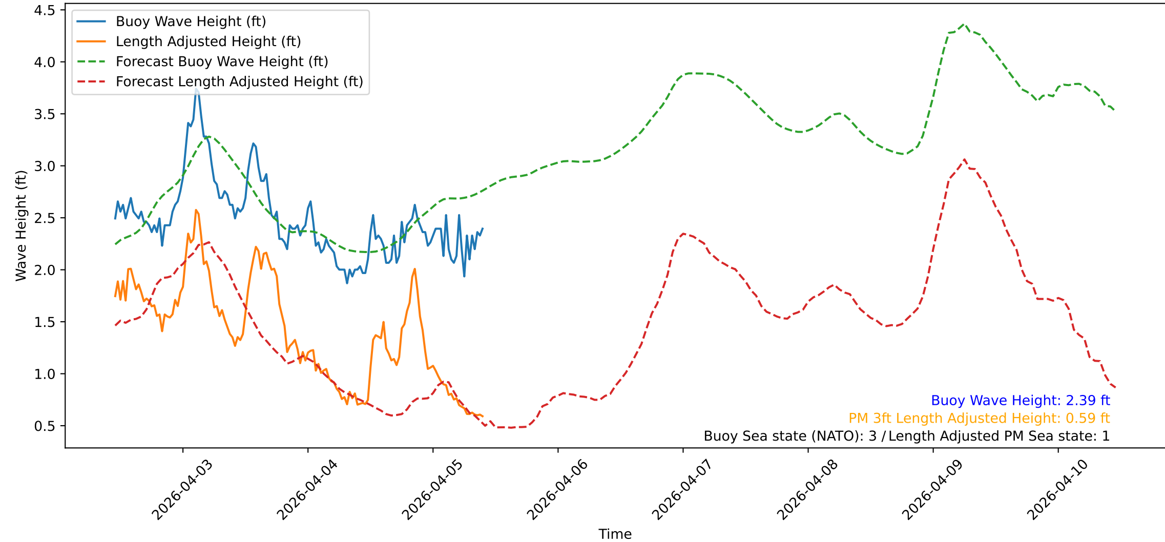
Wave Heights over Time for Red Beach at 2026-04-05 10:30:47
