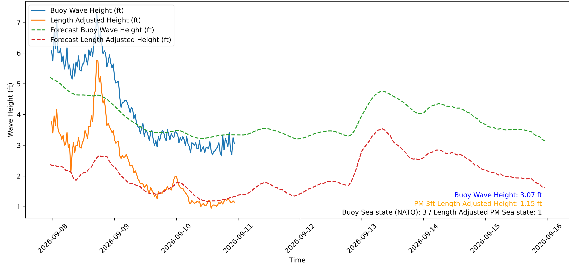
Wave Heights over Time for Oceanside Harbor at 2026-09-10 23:20:29
