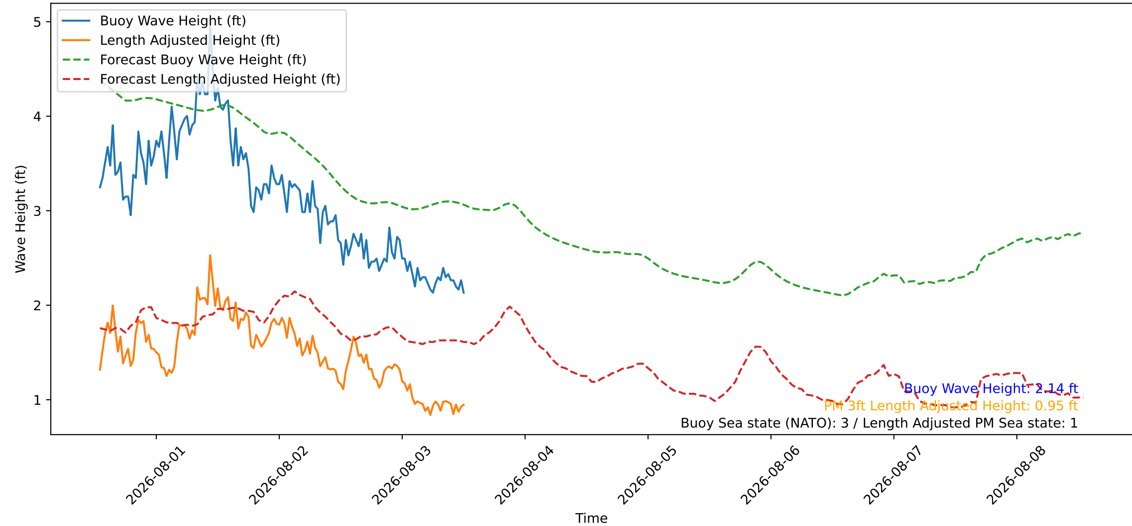
Wave Heights over Time for Green Beach at 2026-08-03 12:51:09
