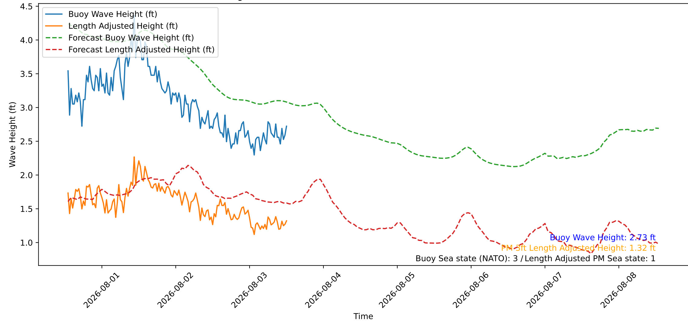
Wave Heights over Time for Oceanside Harbor at 2026-08-03 12:50:26
