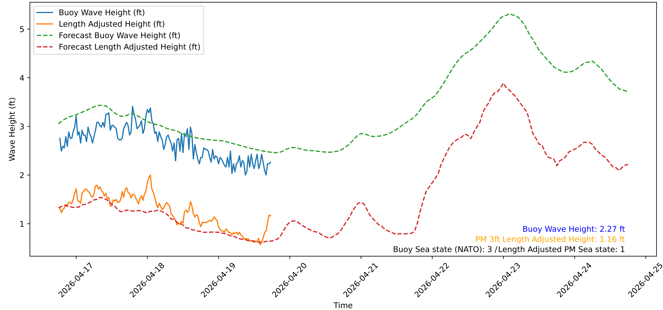
Wave Heights over Time for Oceanside Harbor at 2026-04-19 18:20:31
