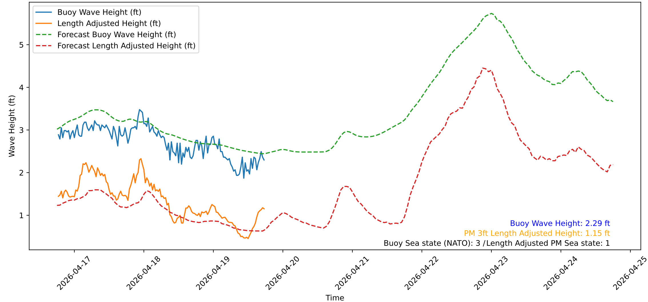
Wave Heights over Time for Green Beach at 2026-04-19 18:21:14
