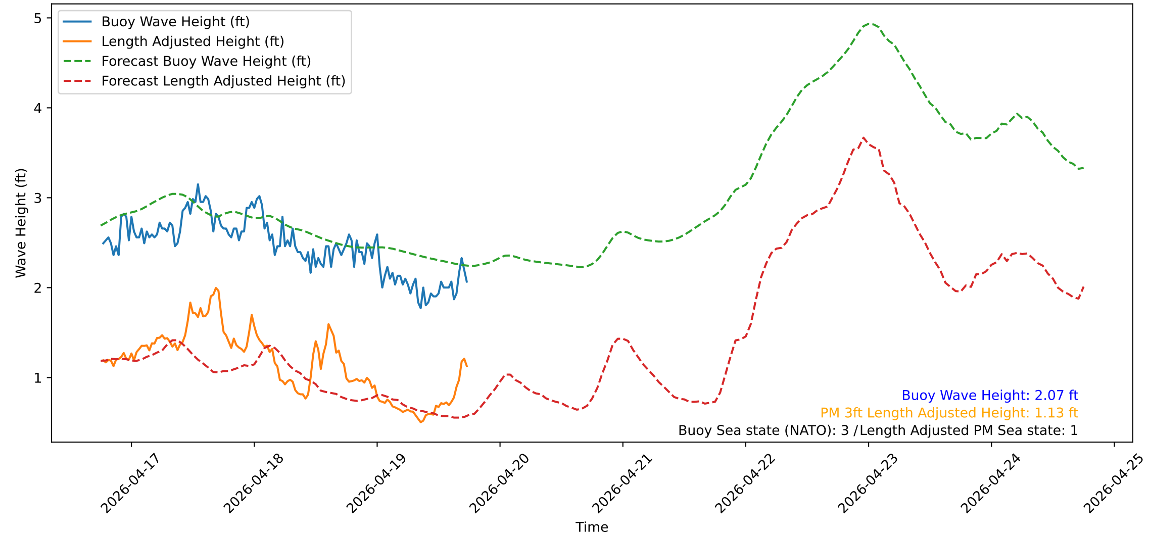
Wave Heights over Time for Red Beach at 2026-04-19 18:20:51
