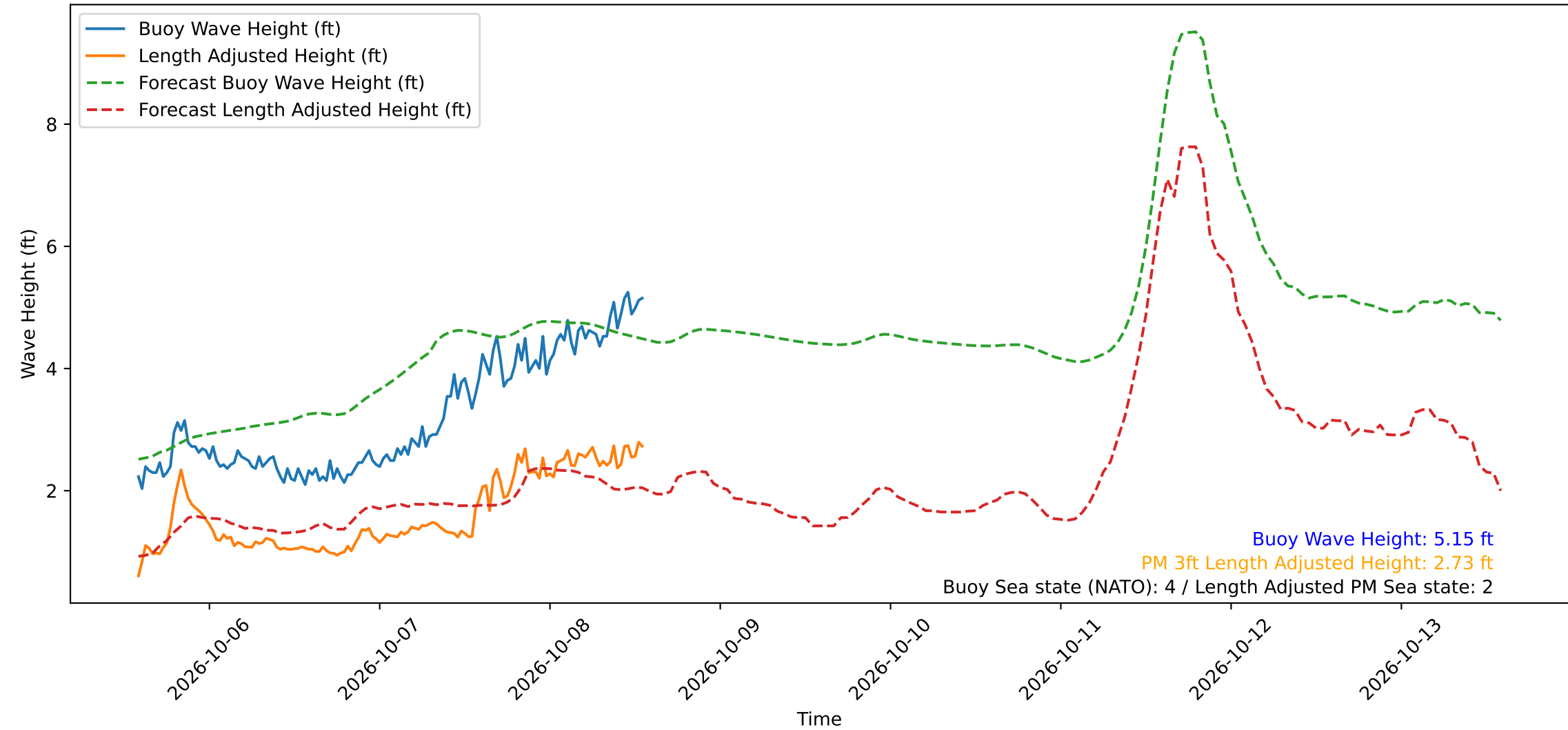
Wave Heights over Time for Green Beach at 2026-10-08 13:41:13
