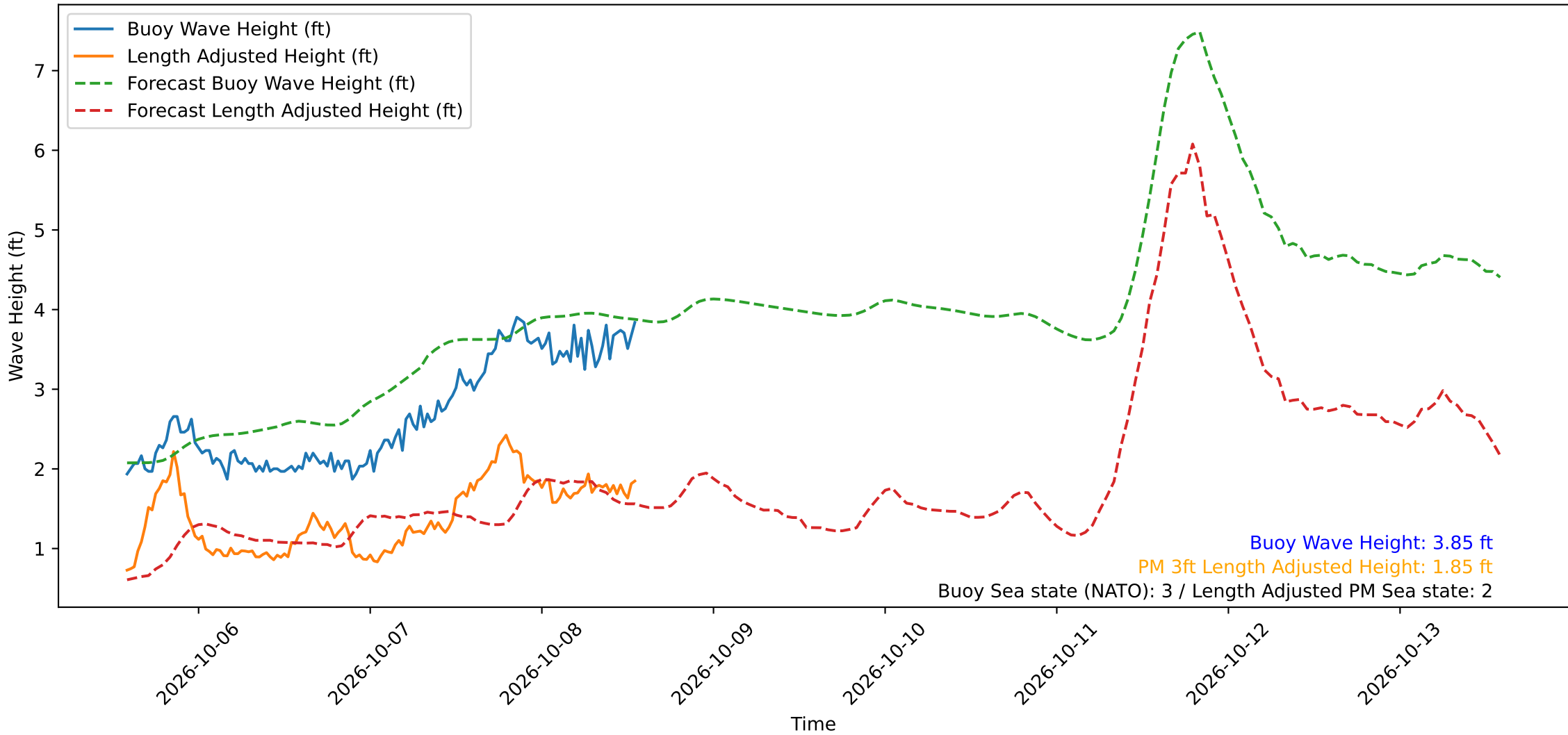
Wave Heights over Time for Red Beach at 2026-10-08 13:40:50
