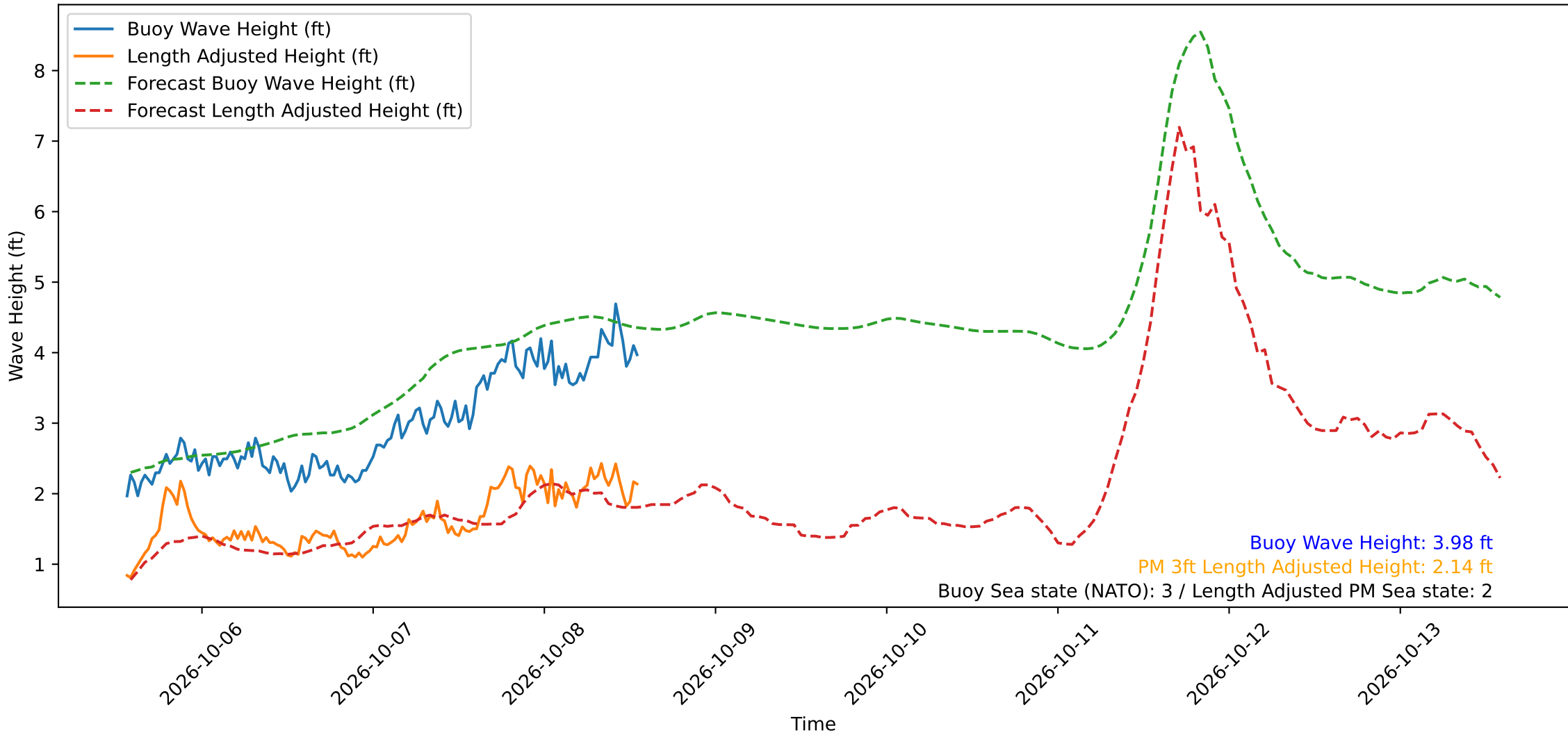
Wave Heights over Time for Oceanside Harbor at 2026-10-08 13:40:30
