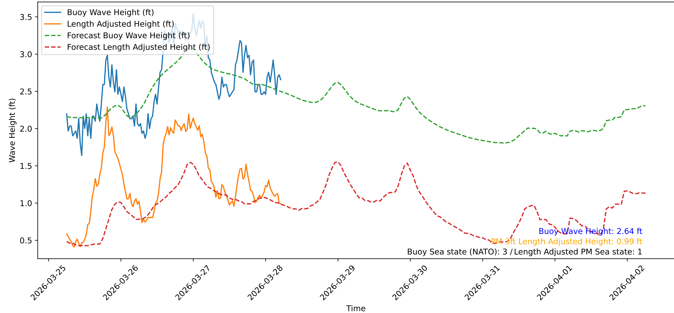
Wave Heights over Time for Green Beach at 2026-03-28 05:51:09
