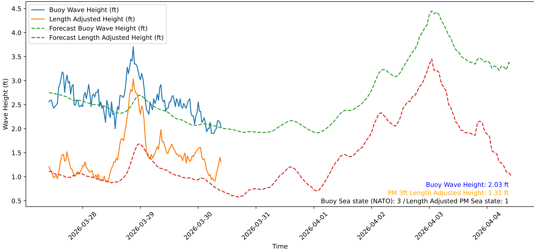
Wave Heights over Time for Green Beach at 2026-03-30 10:11:10
