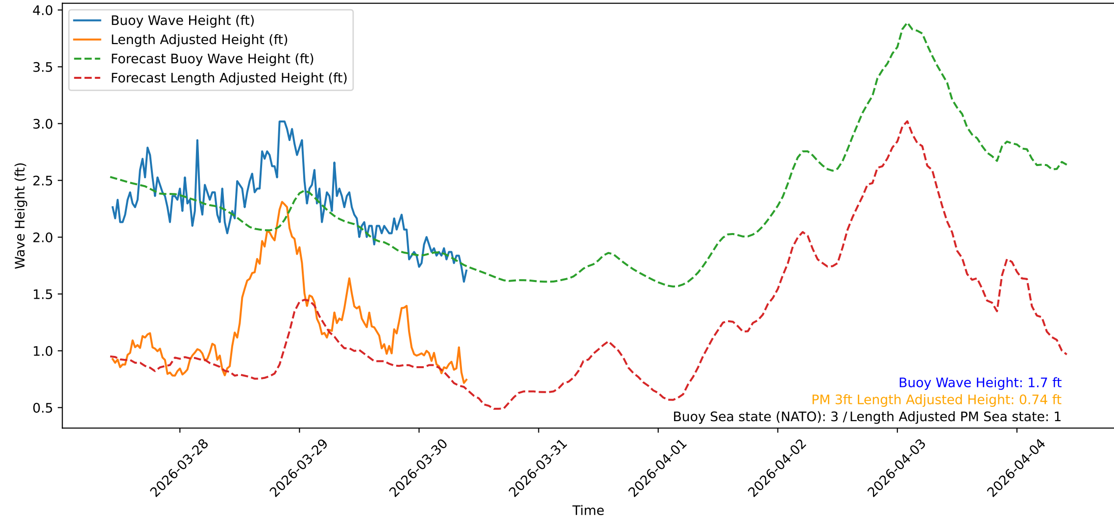
Wave Heights over Time for Red Beach at 2026-03-30 10:10:47
