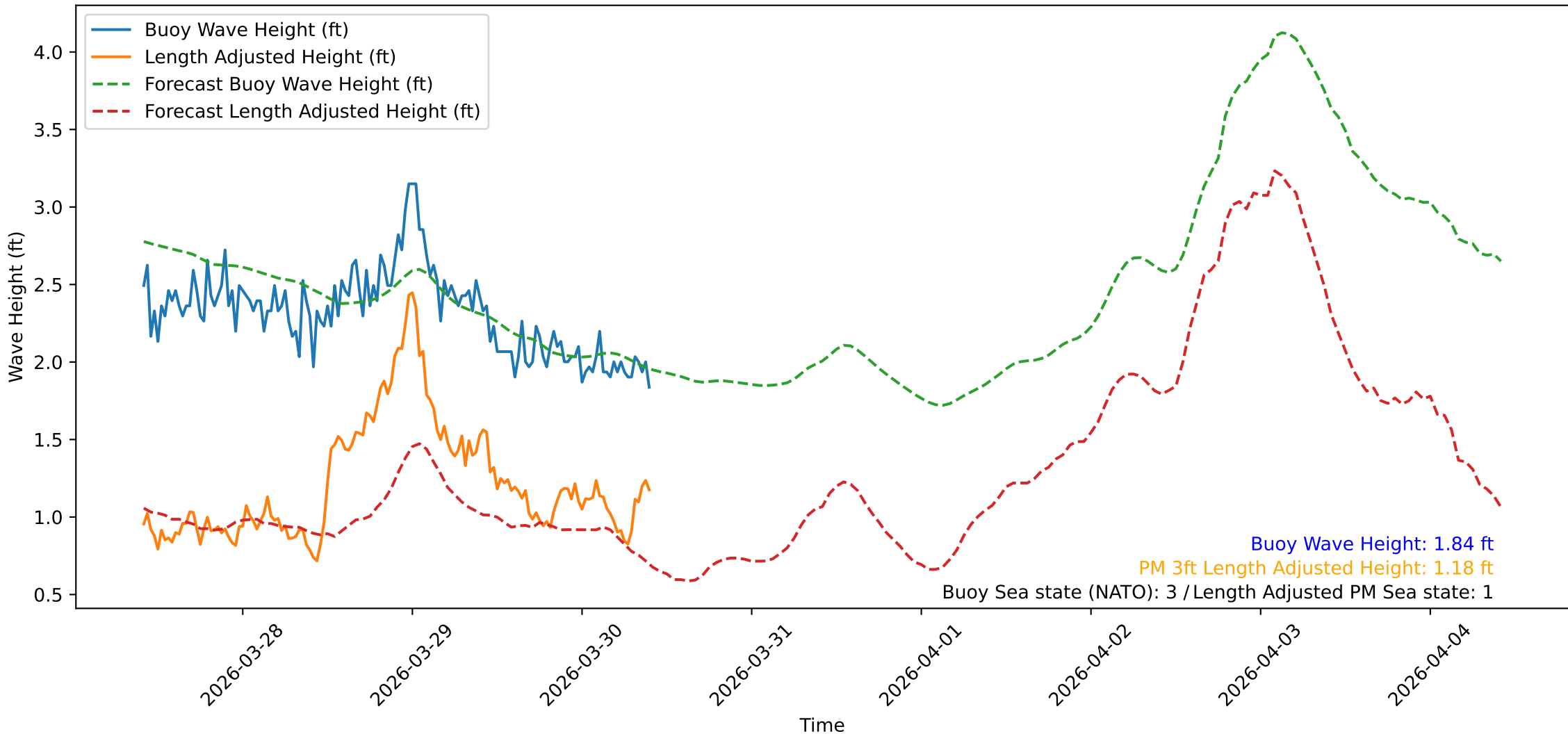
Wave Heights over Time for Oceanside Harbor at 2026-03-30 10:10:31
