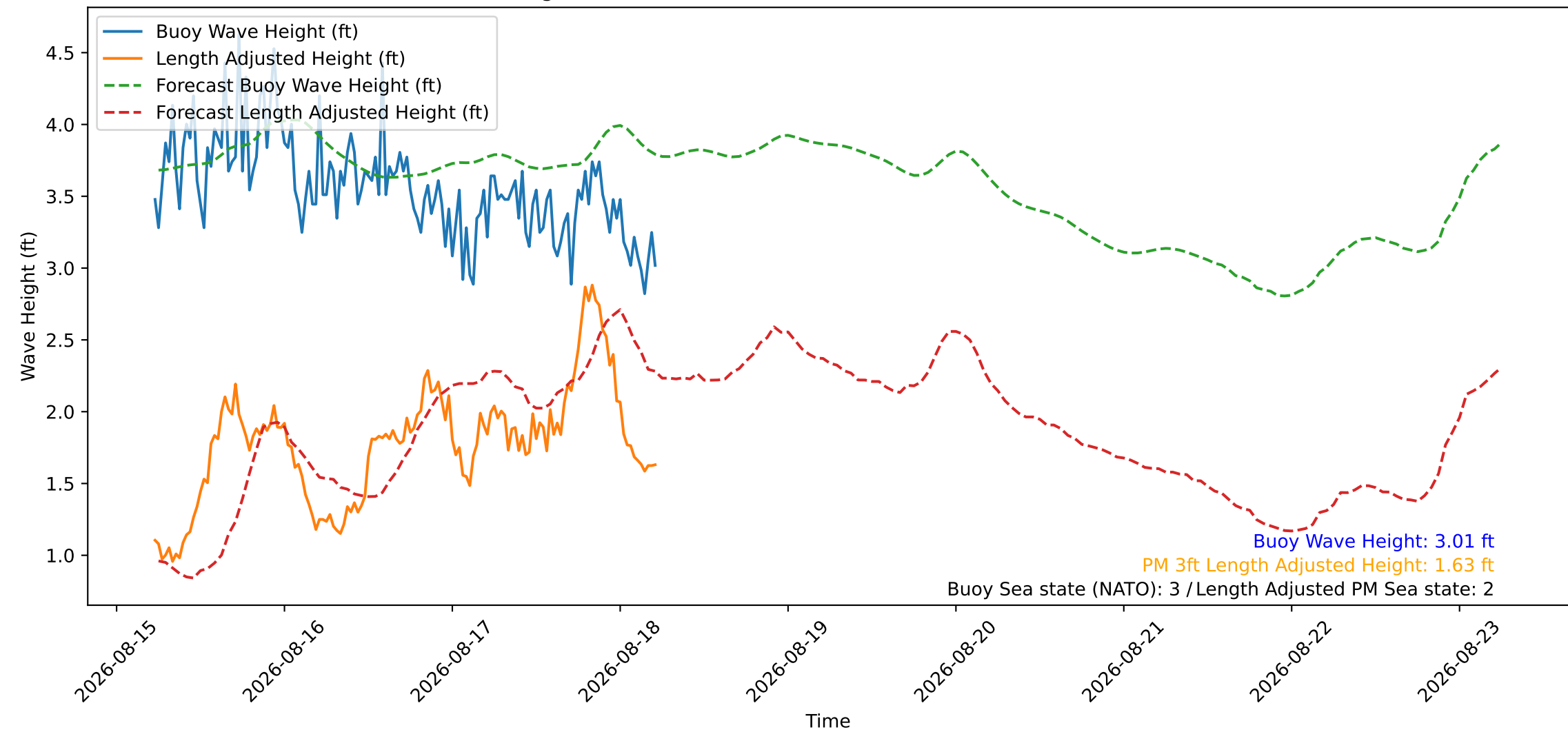
Wave Heights over Time for Oceanside Harbor at 2026-08-18 05:40:27
