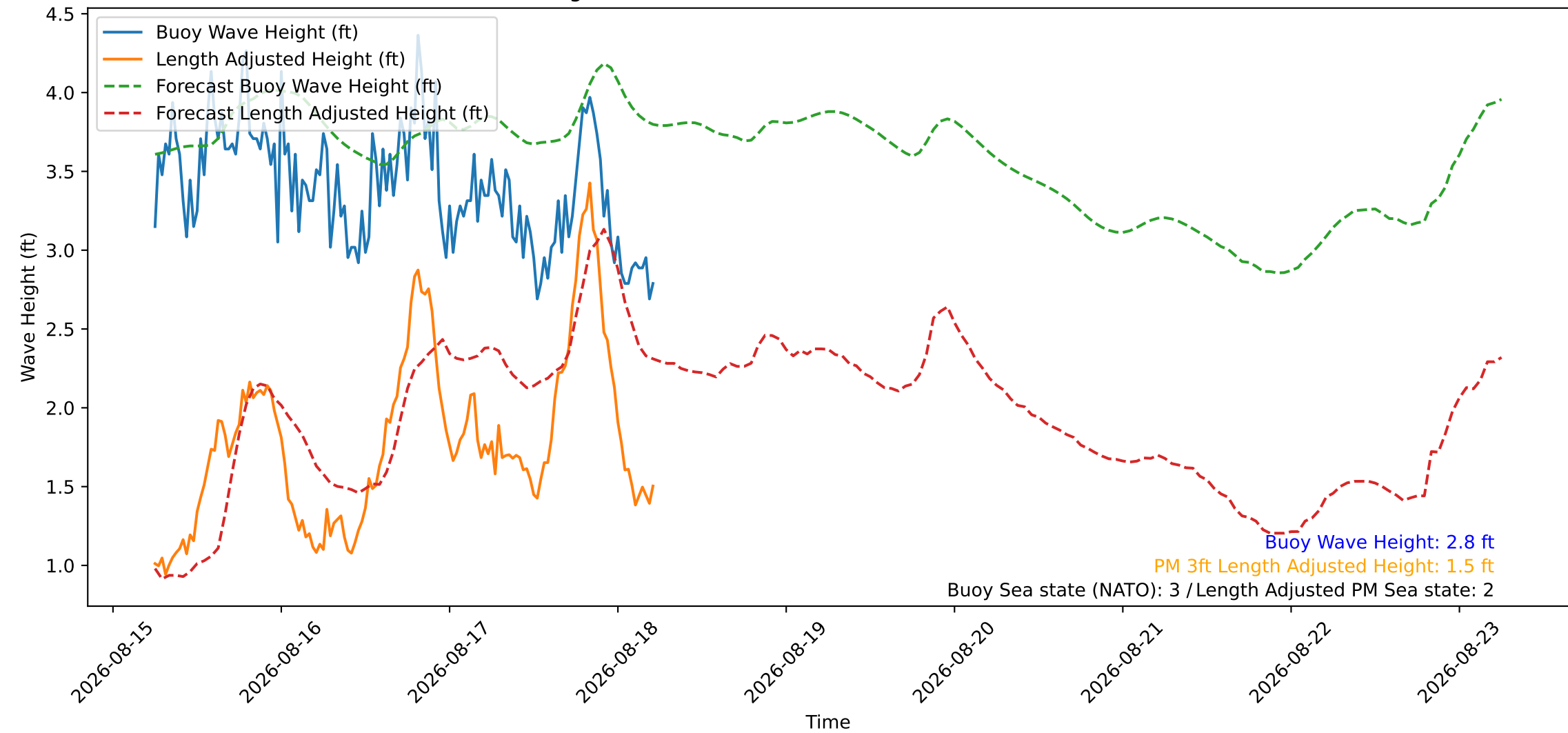
Wave Heights over Time for Green Beach at 2026-08-18 05:41:09
