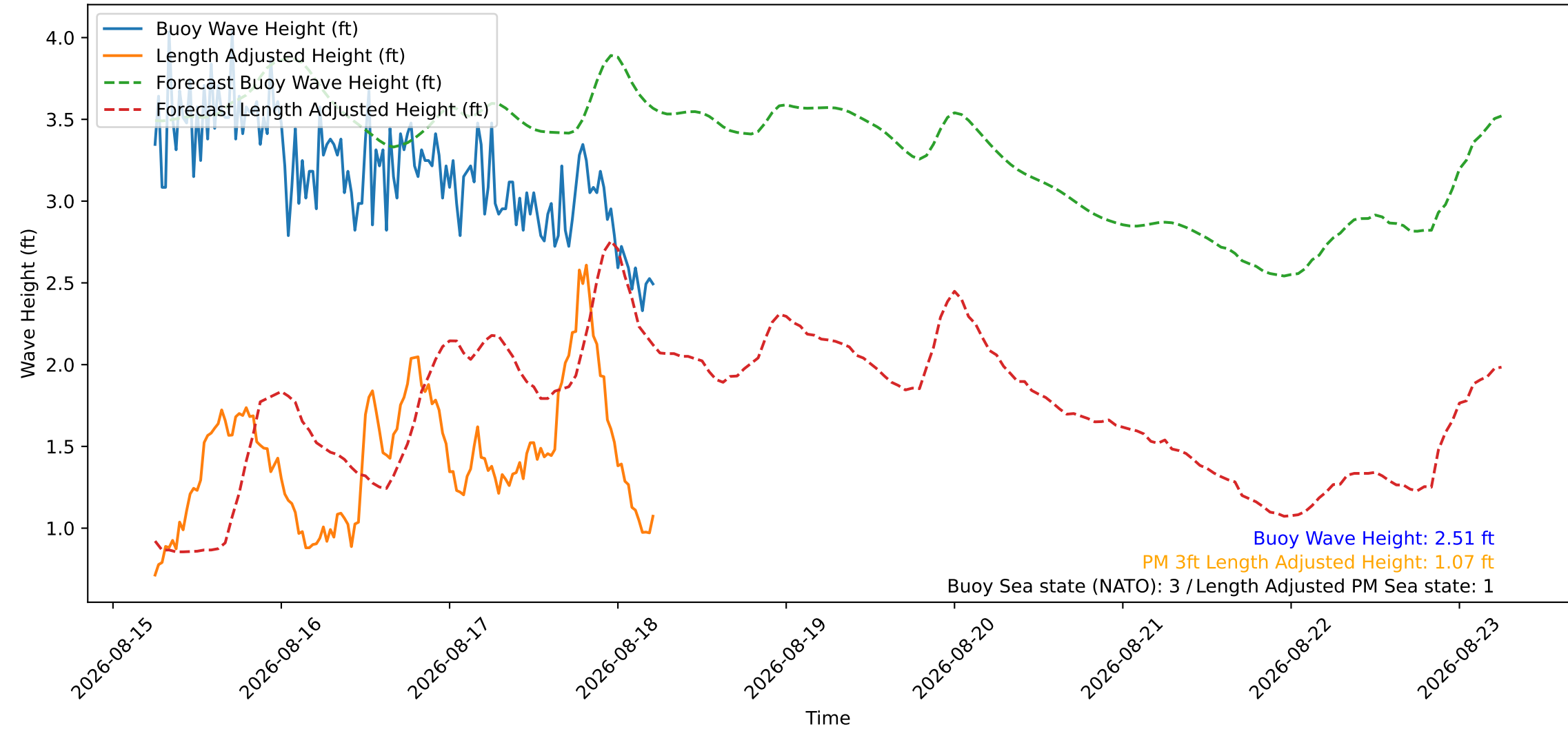
Wave Heights over Time for Red Beach at 2026-08-18 05:40:47
