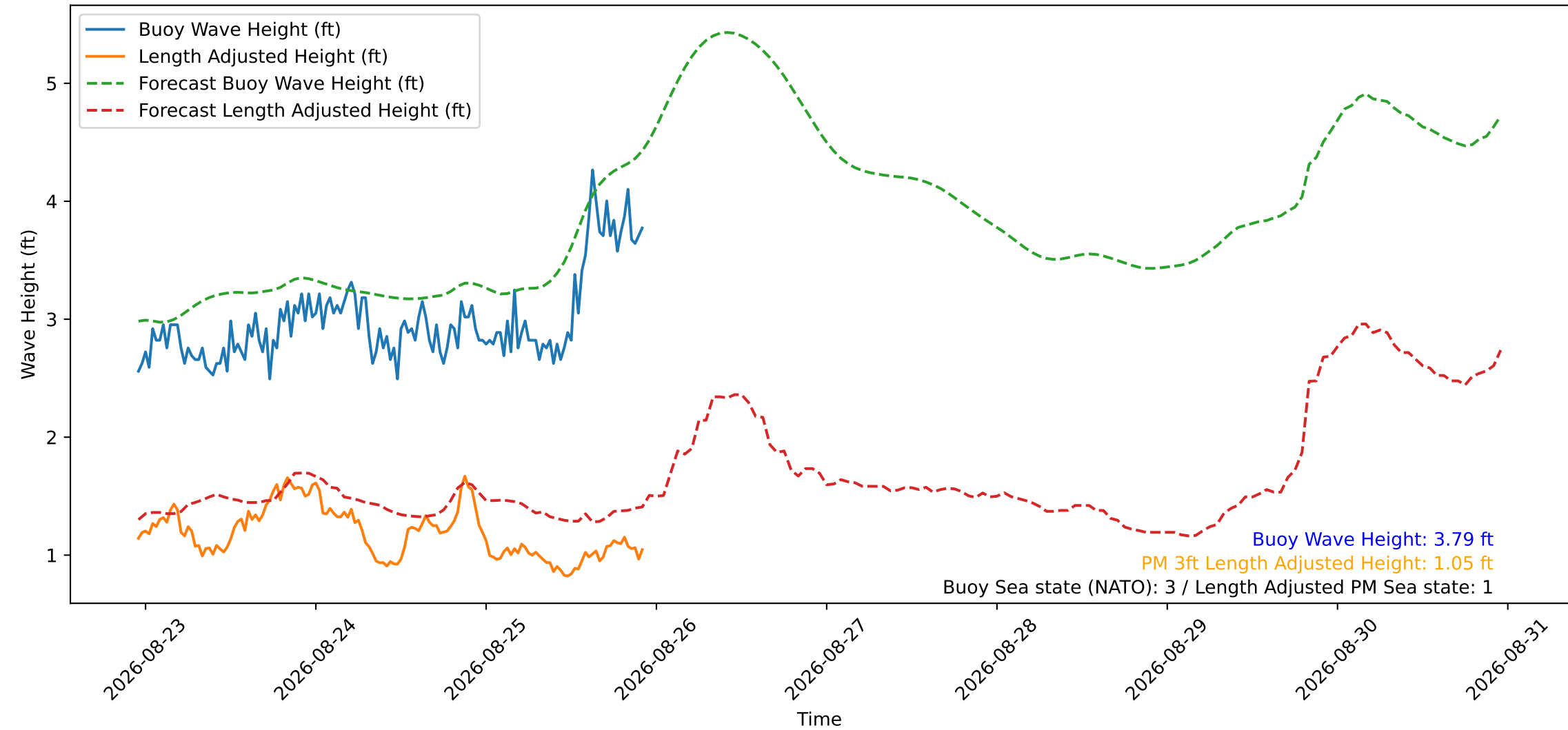
Wave Heights over Time for Green Beach at 2026-08-25 22:41:11
