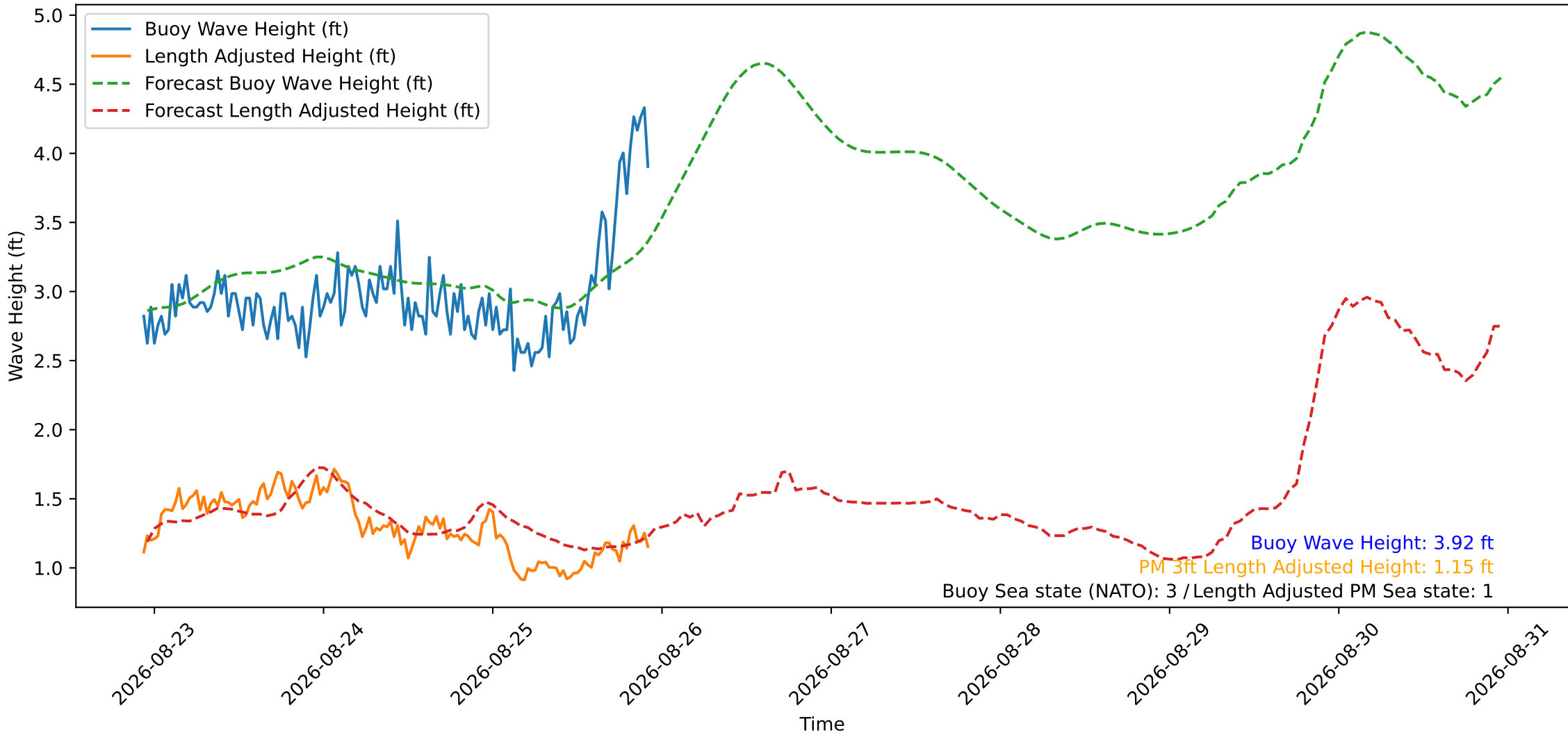
Wave Heights over Time for Oceanside Harbor at 2026-08-25 22:40:29
