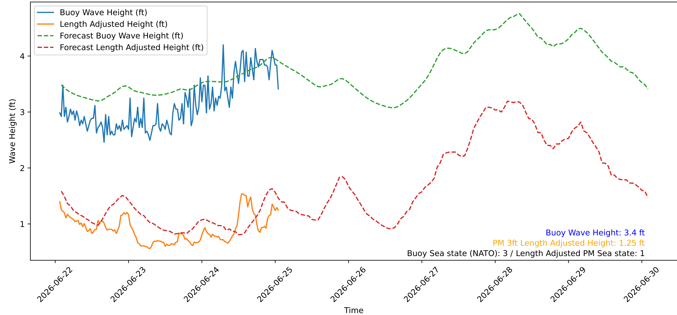
Wave Heights over Time for Green Beach at 2026-06-25 01:41:08
