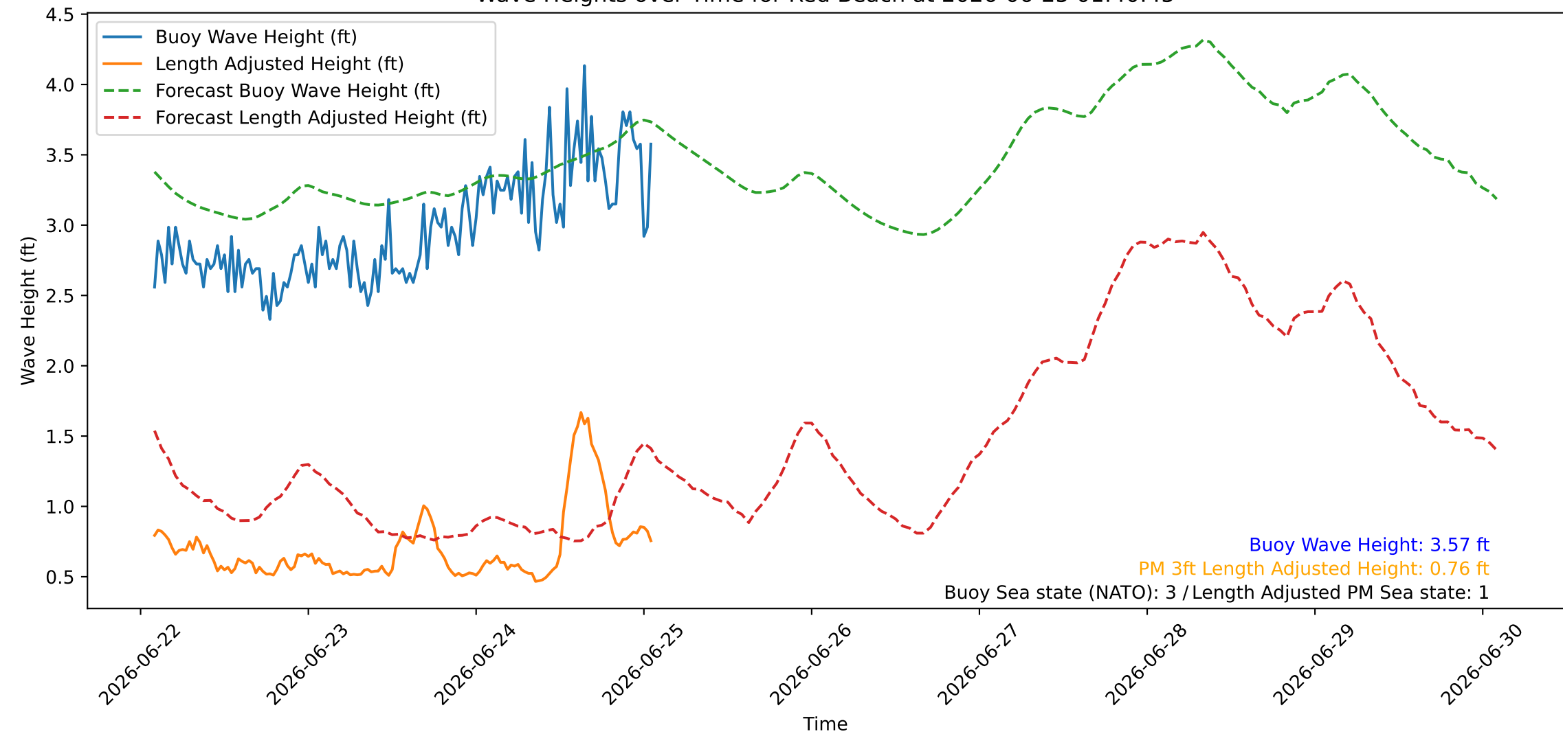
Wave Heights over Time for Red Beach at 2026-06-25 01:40:45
