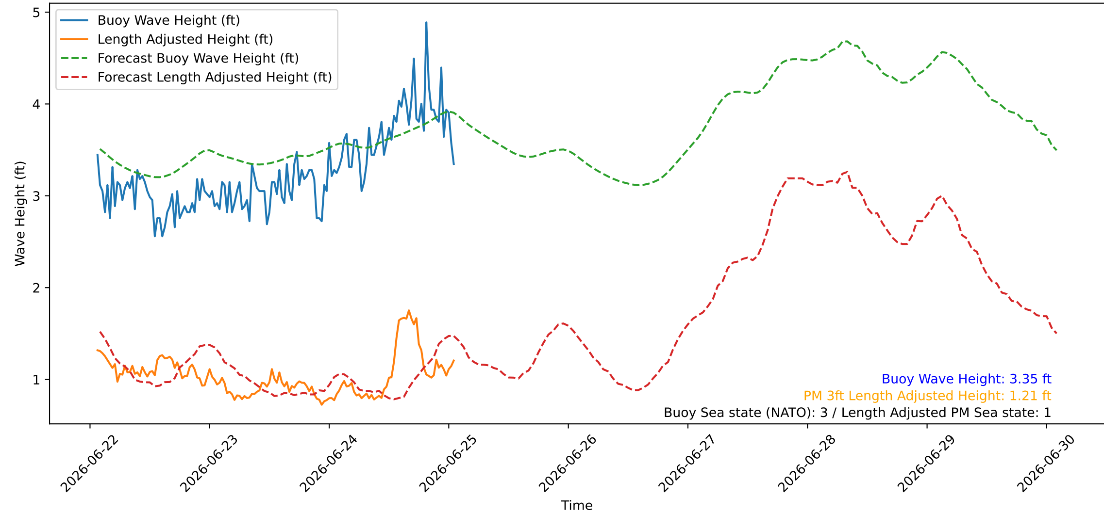
Wave Heights over Time for Oceanside Harbor at 2026-06-25 01:40:26
