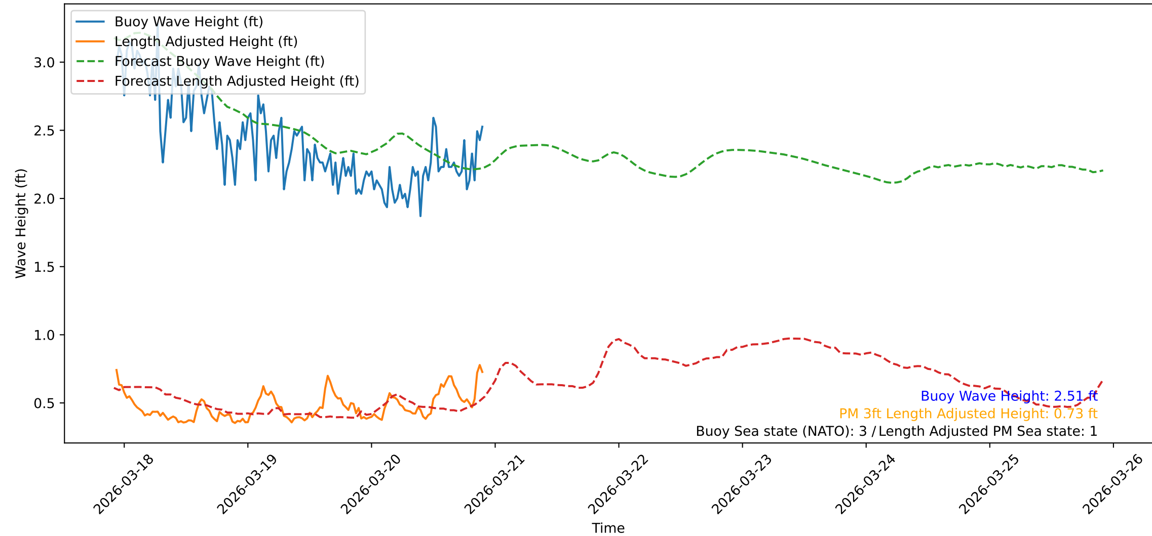
Wave Heights over Time for Red Beach at 2026-03-20 22:10:48
