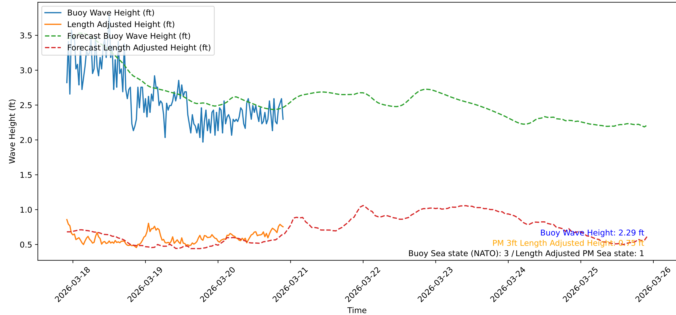
Wave Heights over Time for Oceanside Harbor at 2026-03-20 22:10:32
