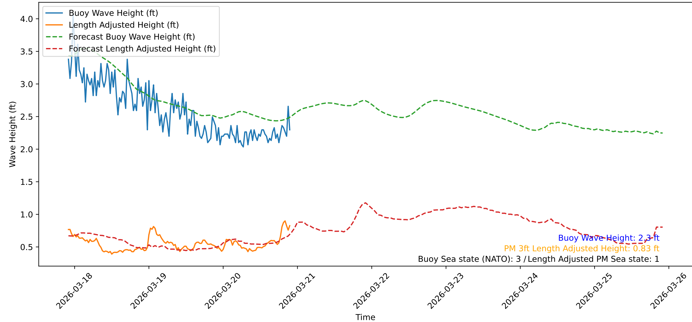
Wave Heights over Time for Green Beach at 2026-03-20 22:11:10
